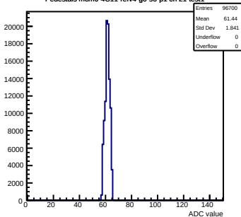
Pedestals mcm0-4C11-refV4-g0-s0-p1 ch 21 test1
