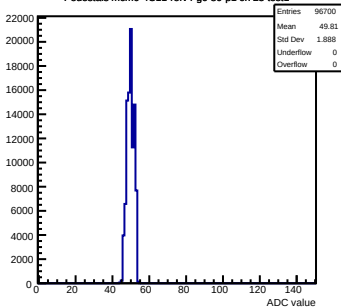
Pedestals mcm0-4C11-refV4-g0-s0-p1 ch 25 test1
