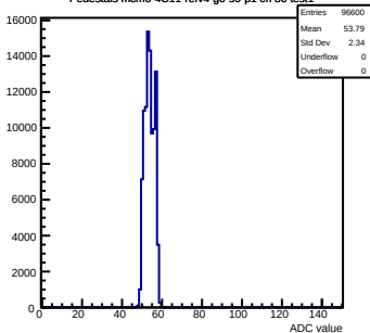
Pedestals mcm0-4C11-refV4-g0-s0-p1 ch 36 test1
