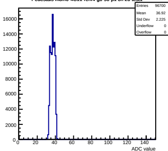
Pedestals mcm0-4C11-refV4-g0-s0-p1 ch 20 test1
