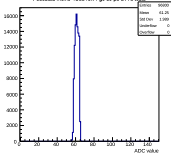
Pedestals mcm0-4C11-refV4-g0-s0-p1 ch 71 test1
