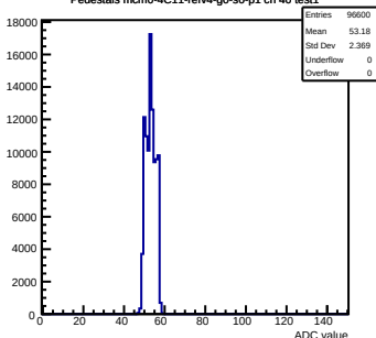
Pedestals mcm0-4C11-refV4-g0-s0-p1 ch 40 test1
