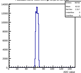
Pedestals mcm0-4C11-refV4-g0-s0-p1 ch 16 test1
