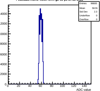
Pedestals mcm0-4C11-refV4-g0-s0-p1 ch 33 test1
