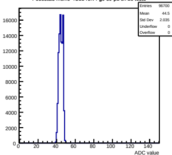
Pedestals mcm0-4C11-refV4-g0-s0-p1 ch 26 test1
