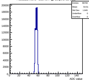
Pedestals mcm0-4C11-refV4-g0-s0-p1 ch 29 test1
