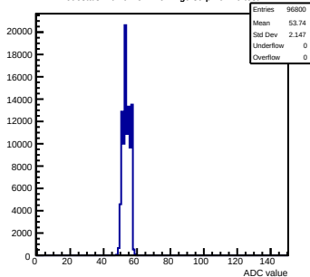
Pedestals mcm0-4C11-refV4-g0-s0-p1 ch 79 test1
