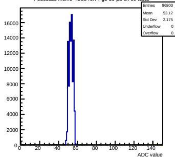
Pedestals mcm0-4C11-refV4-g0-s0-p1 ch 69 test1
