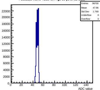
Pedestals mcm0-4C11-refV4-g0-s0-p1 ch 28 test1
