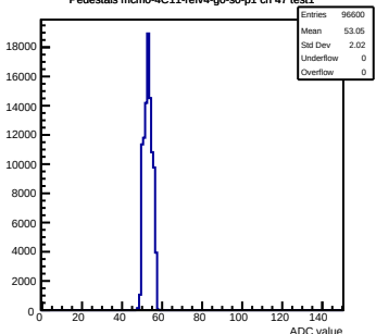
Pedestals mcm0-4C11-refV4-g0-s0-p1 ch 47 test1
