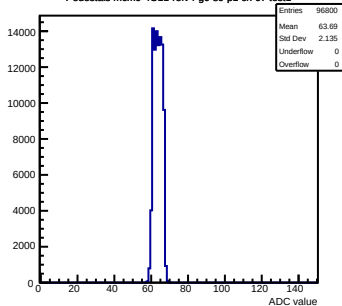
Pedestals mcm0-4C11-refV4-g0-s0-p1 ch 67 test1
