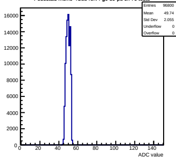
Pedestals mcm0-4C11-refV4-g0-s0-p1 ch 70 test1
