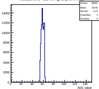
Pedestals mcm0-4C11-refV4-g0-s0-p1 ch 64 test1
