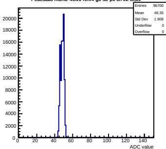
Pedestals mcm0-4C11-refV4-g0-s0-p1 ch 22 test1
