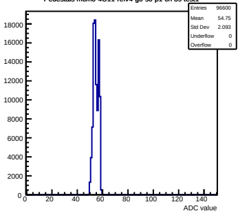
Pedestals mcm0-4C11-refV4-g0-s0-p1 ch 39 test1
