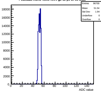
Pedestals mcm0-4C11-refV4-g0-s0-p1 ch 19 test1
