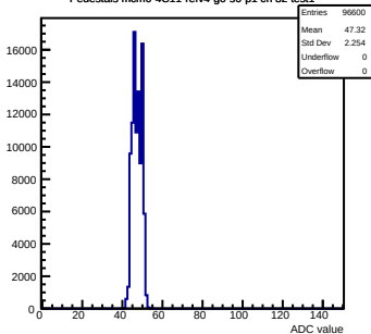
Pedestals mcm0-4C11-refV4-g0-s0-p1 ch 32 test1
