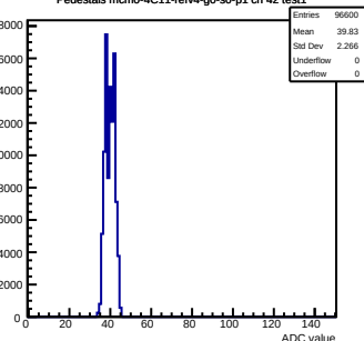
Pedestals mcm0-4C11-refV4-g0-s0-p1 ch 42 test1
