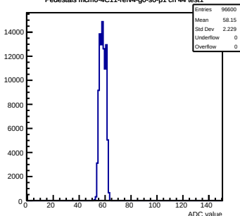
Pedestals mcm0-4C11-refV4-g0-s0-p1 ch 44 test1
