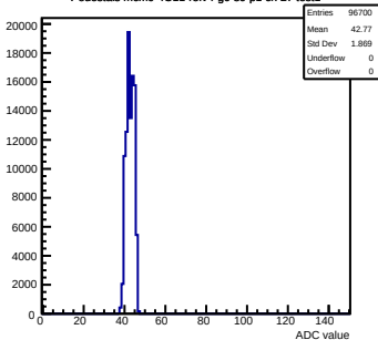
Pedestals mcm0-4C11-refV4-g0-s0-p1 ch 27 test1
