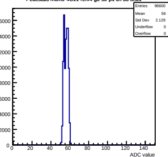
Pedestals mcm0-4C11-refV4-g0-s0-p1 ch 38 test1
