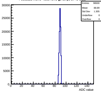
Pedestals mcm0-4C11-relV5-g0-s0-p1 ch 49 test1
