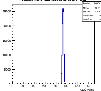
Pedestals mcm0-4C11-refV5-g0-s0-p1 ch 97 test1
