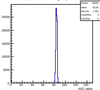
Pedestals mcm0-4C11-relV5-g0-s0-p1 ch 63 test1
