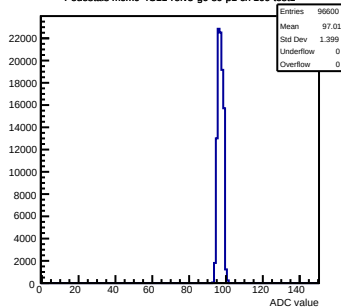
Pedestals mcm0-4C11-refV5-g0-s0-p1 ch 109 test1
