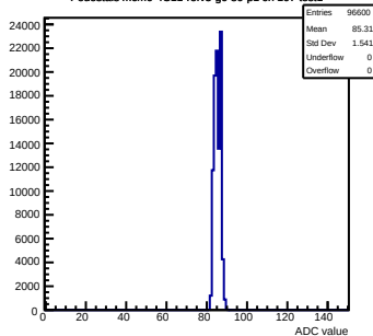
Pedestals mcm0-4C11-refV5-g0-s0-p1 ch 107 test1
