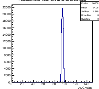
Pedestals mcm0-4C11-refV5-g0-s0-p1 ch 102 test1
