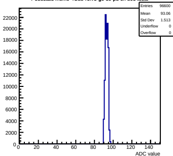
Pedestals mcm0-4C11-refV5-g0-s0-p1 ch 108 test1
