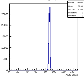
Pedestals mcm0-4C11-relV5-g0-s0-p1 ch 57 test1
