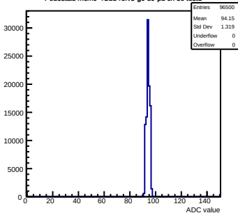
Pedestals mcm0-4C11-relV5-g0-s0-p1 ch 50 test1
