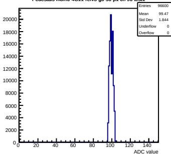
Pedestals mcm0-4C11-refV5-g0-s0-p1 ch 96 test1
