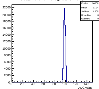
Pedestals mcm0-4C11-refV5-g0-s0-p1 ch 106 test1
