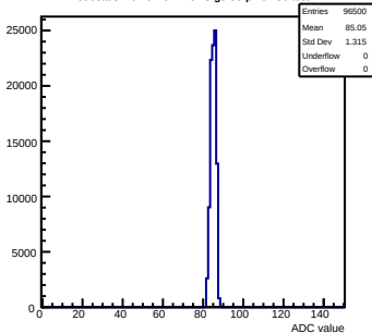
Pedestals mcm0-4C11-relV5-g0-s0-p1 ch 56 test1
