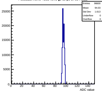
Pedestals mcm0-4C11-refV5-g0-s0-p1 ch 104 test1
