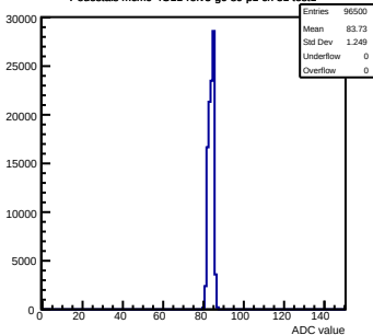
Pedestals mcm0-4C11-relV5-g0-s0-p1 ch 51 test1
