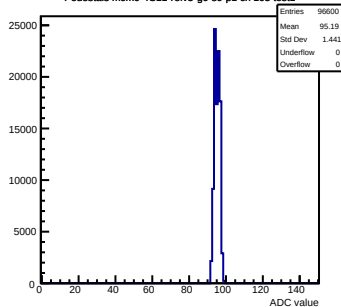
Pedestals mcm0-4C11-refV5-g0-s0-p1 ch 105 test1
