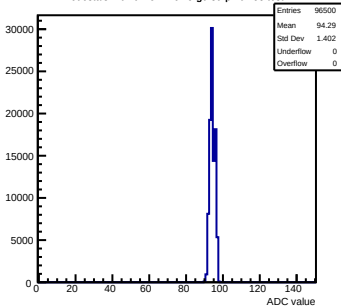
Pedestals mcm0-4C11-relV5-g0-s0-p1 ch 58 test1
