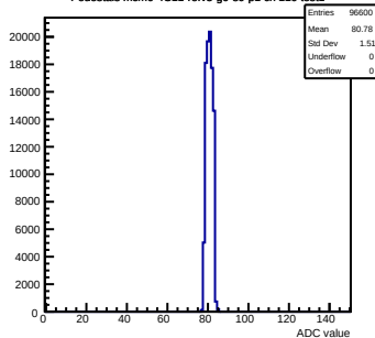
Pedestals mcm0-4C11-refV5-g0-s0-p1 ch 110 test1
