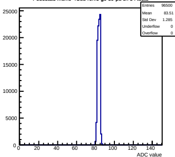
Pedestals mcm0-4C11-relV5-g0-s0-p1 ch 54 test1
