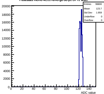
Pedestals mcm0-4C11-relv6-g0-s0-p1 ch 72 test1
