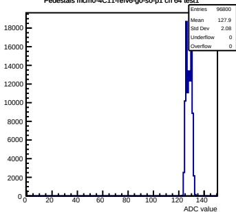
Pedestals mcm0-4C11-relv6-g0-s0-p1 ch 64 test1
