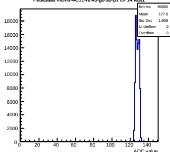
Pedestals mcm0-4C11-rlv6-g0-s0-p1 ch 14 test1
