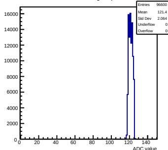
Pedestals mcm0-4C11-relv6-g0-s0-p1 ch 110 test1
