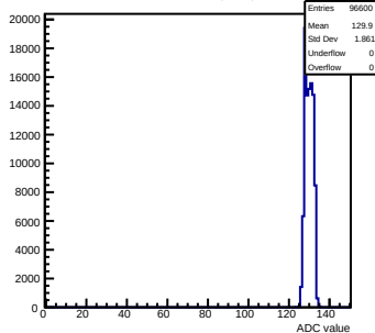
Pedestals mcm0-4C11-relv6-g0-s0-p1 ch 98 test1
