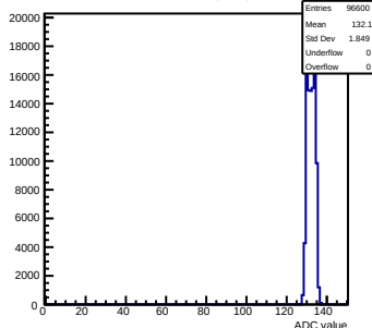
Pedestals mcm0-4C11-relv6-g0-s0-p1 ch 102 test1
