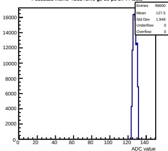
Pedestals mcm0-4C11-relv6-g0-s0-p1 ch 44 test1
