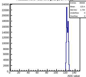
Pedestals mcm0-4C11-relv6-g0-s0-p1 ch 47 test1
