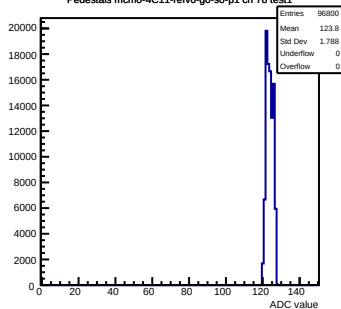
Pedestals mcm0-4C11-relv6-g0-s0-p1 ch 78 test1
