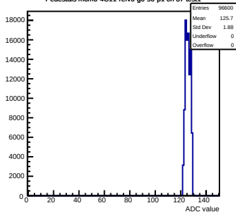
Pedestals mcm0-4C11-relv6-g0-s0-p1 ch 37 test1
