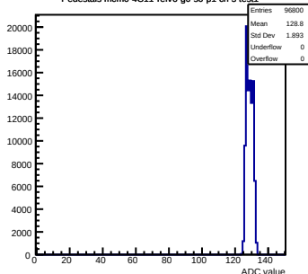
Pedestals mcm0-4C11-rlv6-g0-s0-p1 ch 5 test1
