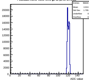
Pedestals mcm0-4C11-relv6-g0-s0-p1 ch 34 test1
