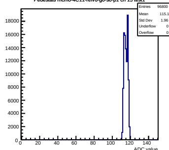
Pedestals mcm0-4C11-rlv6-g0-s0-p1 ch 15 test1
