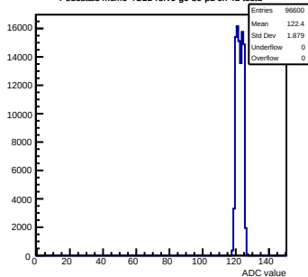
Pedestals mcm0-4C11-relv6-g0-s0-p1 ch 41 test1
