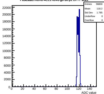
Pedestals mcm0-4C11-relv6-g0-s0-p1 ch 77 test1
