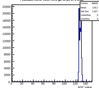
Pedestals mcm0-4C11-rlv6-g0-s0-p1 ch 6 test1
