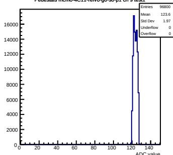
Pedestals mcm0-4C11-rlv6-g0-s0-p1 ch 9 test1
