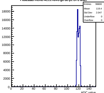
Pedestals mcm0-4C11-rlv6-g0-s0-p1 ch 8 test1
