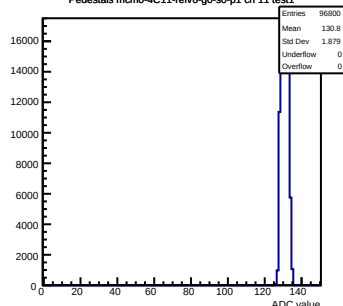
Pedestals mcm0-4C11-rlv6-g0-s0-p1 ch 11 test1
