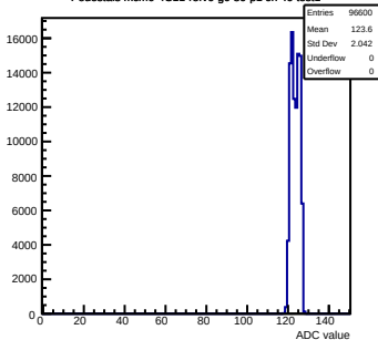
Pedestals mcm0-4C11-relv6-g0-s0-p1 ch 40 test1
