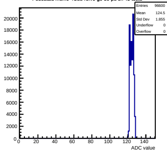
Pedestals mcm0-4C11-relv6-g0-s0-p1 ch 45 test1
