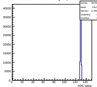
Pedestals mcm10-4C11-refV0-g0-s0-p1 ch 91 test1
