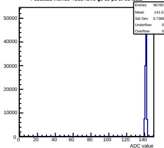
Pedestals mcm10-4C11-refV0-g0-s0-p1 ch 86 test1
