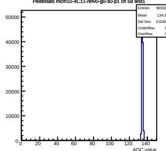
Pedestals mcm10-4C11-refV0-g0-s0-p1 ch 58 test1
