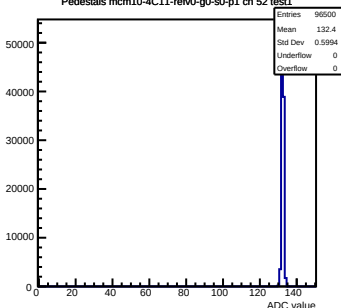
Pedestals mcm10-4C11-refV0-g0-s0-p1 ch 52 test1
