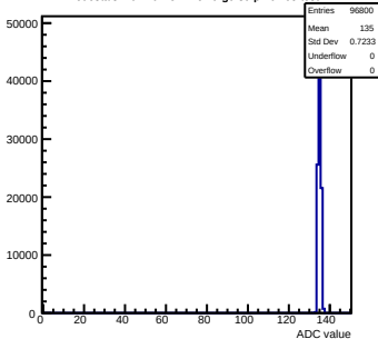
Pedestals mcm10-4C11-refV0-g0-s0-p1 ch 65 test1
