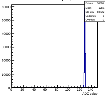
Pedestals mcm10-4C11-refV0-g0-s0-p1 ch 73 test1
