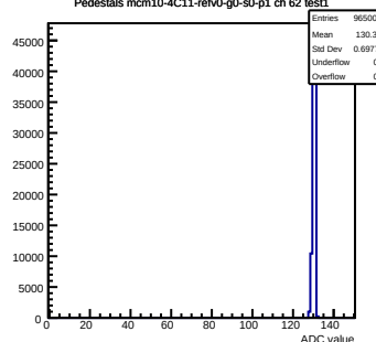
Pedestals mcm10-4C11-refV0-g0-s0-p1 ch 62 test1
