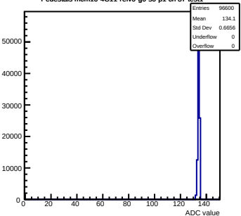
Pedestals mcm10-4C11-refV0-g0-s0-p1 ch 37 test1
