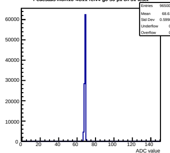
Pedestals mcm10-4C11-refV4-g0-s0-p1 ch 51 test1
