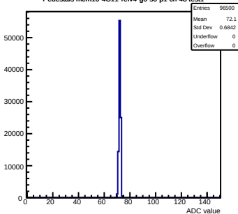
Pedestals mcm10-4C11-refV4-g0-s0-p1 ch 48 test1
