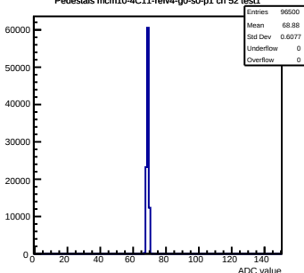
Pedestals mcm10-4C11-refV4-g0-s0-p1 ch 52 test1
