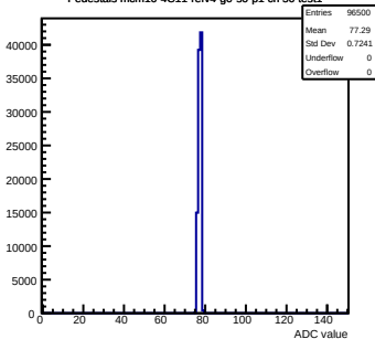
Pedestals mcm10-4C11-refV4-g0-s0-p1 ch 50 test1
