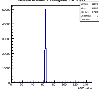
Pedestals mcm10-4C11-refV4-g0-s0-p1 ch 53 test1
