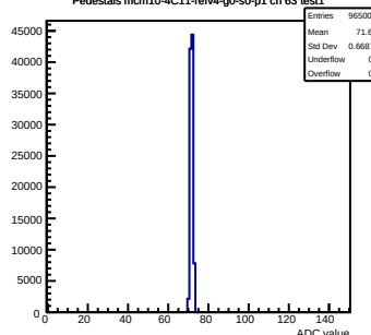
Pedestals mcm10-4C11-refV4-g0-s0-p1 ch 63 test1
