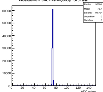
Pedestals mcm10-4C11-refV4-g0-s0-p1 ch 57 test1
