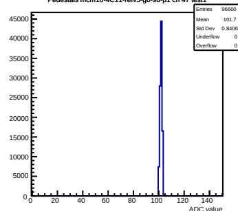
Pedestals mcm10-4C11-refV5-g0-s0-p1 ch 47 test1
