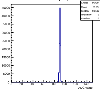
Pedestals mcm10-4C11-refV5-g0-s0-p1 ch 21 test1
