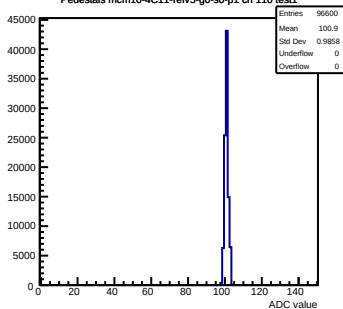
Pedestals mcm10-4C11-reV5-g0-s0-p1 ch 110 test1
