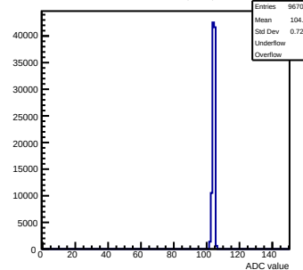
Pedestals mcm10-4C11-refV5-g0-s0-p1 ch 87 test1
