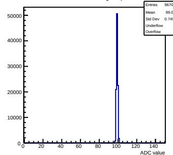
Pedestals mcm10-4C11-refV5-g0-s0-p1 ch 91 test1
