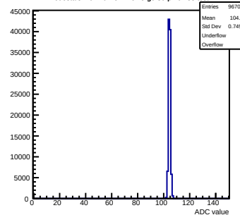
Pedestals mcm10-4C11-refV5-g0-s0-p1 ch 83 test1
