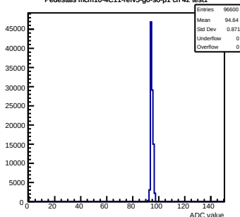
Pedestals mcm10-4C11-refV5-g0-s0-p1 ch 42 test1
