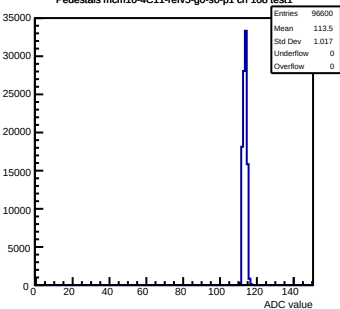
Pedestals mcm10-4C11-reV5-g0-s0-p1 ch 108 test1
