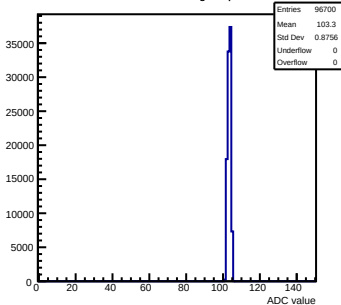
Pedestals mcm10-4C11-refV5-g0-s0-p1 ch 24 test1
