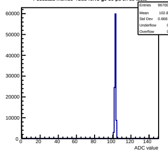
Pedestals mcm10-4C11-refV5-g0-s0-p1 ch 19 test1
