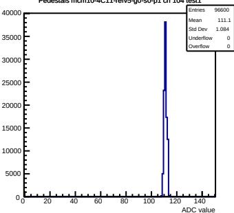
Pedestals mcm10-4C11-reV5-g0-s0-p1 ch 104 test1
