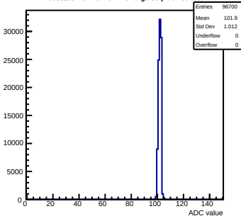
Pedestals mcm10-4C11-refV5-g0-s0-p1 ch 80 test1
