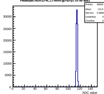
Pedestals mcm10-4C11-reV5-g0-s0-p1 ch 99 test1
