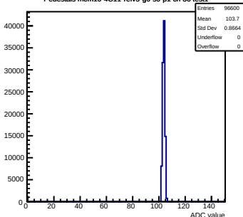
Pedestals mcm10-4C11-refV5-g0-s0-p1 ch 36 test1
