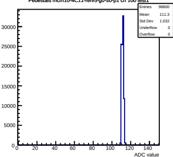
Pedestals mcm10-4C11-reV5-g0-s0-p1 ch 100 test1
