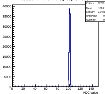
Pedestals mcm10-4C11-refV5-g0-s0-p1 ch 18 test1
