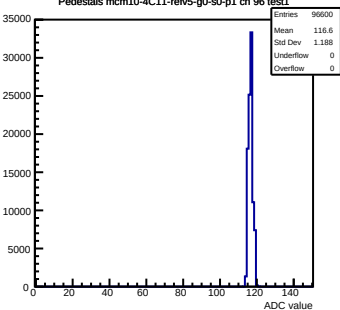
Pedestals mcm10-4C11-reV5-g0-s0-p1 ch 96 test1
