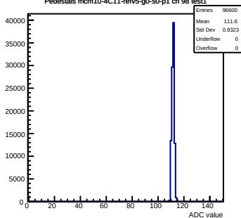
Pedestals mcm10-4C11-reV5-g0-s0-p1 ch 98 test1
