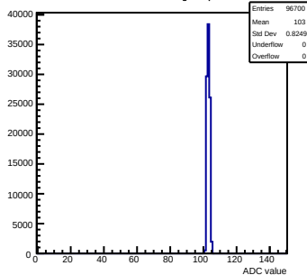
Pedestals mcm10-4C11-refV5-g0-s0-p1 ch 30 test1
