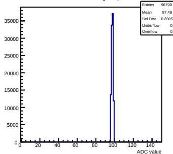
Pedestals mcm10-4C11-refV5-g0-s0-p1 ch 26 test1
