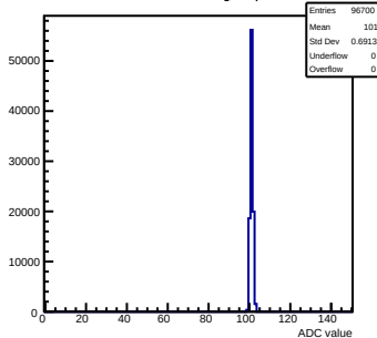
Pedestals mcm10-4C11-refV5-g0-s0-p1 ch 89 test1
