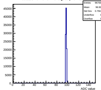
Pedestals mcm10-4C11-refV5-g0-s0-p1 ch 23 test1
