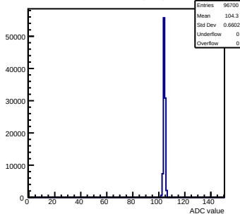
Pedestals mcm10-4C11-refV5-g0-s0-p1 ch 85 test1
