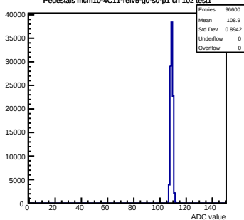
Pedestals mcm10-4C11-reV5-g0-s0-p1 ch 102 test1
