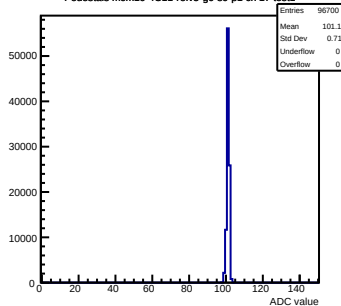
Pedestals mcm10-4C11-refV5-g0-s0-p1 ch 17 test1
