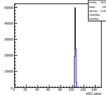
Pedestals mcm10-4C11-refV5-g0-s0-p1 ch 95 test1
