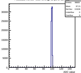
Pedestals mcm10-4C11-refV5-g0-s0-p1 ch 32 test1
