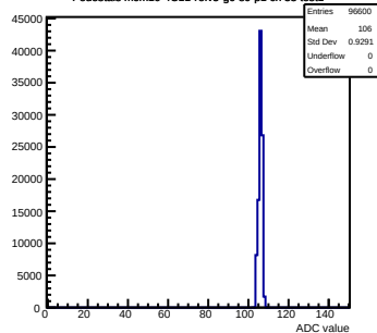
Pedestals mcm10-4C11-refV5-g0-s0-p1 ch 33 test1
