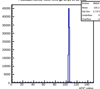
Pedestals mcm10-4C11-refV5-g0-s0-p1 ch 38 test1
