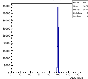
Pedestals mcm10-4C11-refV5-g0-s0-p1 ch 90 test1
