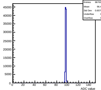
Pedestals mcm10-4C11-refV5-g0-s0-p1 ch 94 test1
