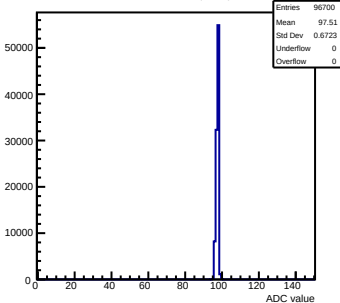
Pedestals mcm10-4C11-refV5-g0-s0-p1 ch 84 test1
