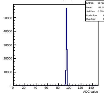
Pedestals mcm10-4C11-refV5-g0-s0-p1 ch 27 test1
