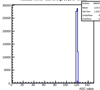
Pedestals mcm10-4C11-refV6-g0-s0-p1 ch 42 test1
