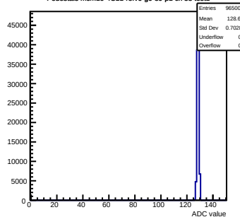
Pedestals mcm10-4C11-refV6-g0-s0-p1 ch 58 test1
