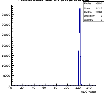
Pedestals mcm10-4C11-refV6-g0-s0-p1 ch 32 test1
