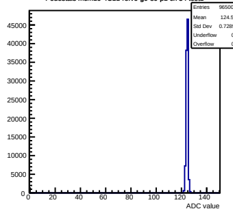
Pedestals mcm10-4C11-refV6-g0-s0-p1 ch 54 test1
