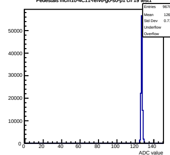
Pedestals mcm10-4C11-refV6-g0-s0-p1 ch 19 test1
