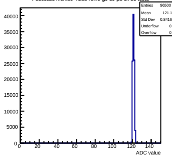
Pedestals mcm10-4C11-refV6-g0-s0-p1 ch 53 test1
