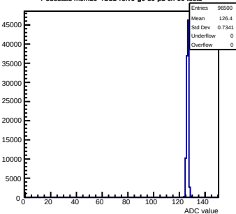
Pedestals mcm10-4C11-refV6-g0-s0-p1 ch 60 test1
