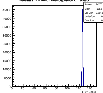
Pedestals mcm10-4C11-refV6-g0-s0-p1 ch 29 test1
