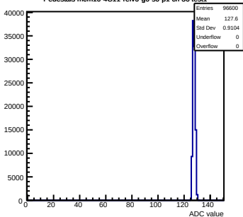
Pedestals mcm10-4C11-refV6-g0-s0-p1 ch 36 test1
