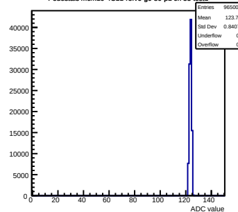
Pedestals mcm10-4C11-refV6-g0-s0-p1 ch 55 test1
