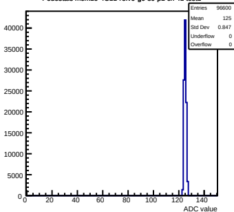
Pedestals mcm10-4C11-refV6-g0-s0-p1 ch 41 test1
