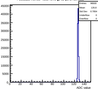
Pedestals mcm10-4C11-refV6-g0-s0-p1 ch 56 test1
