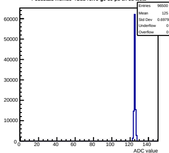
Pedestals mcm10-4C11-refV6-g0-s0-p1 ch 61 test1
