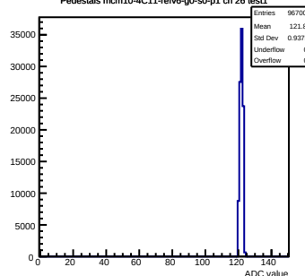
Pedestals mcm10-4C11-refV6-g0-s0-p1 ch 26 test1
