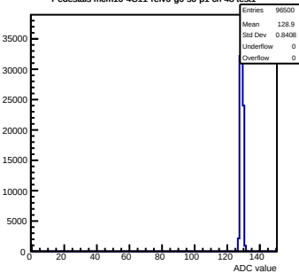
Pedestals mcm10-4C11-refV6-g0-s0-p1 ch 48 test1
