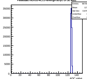
Pedestals mcm10-4C11-refV6-g0-s0-p1 ch 30 test1
