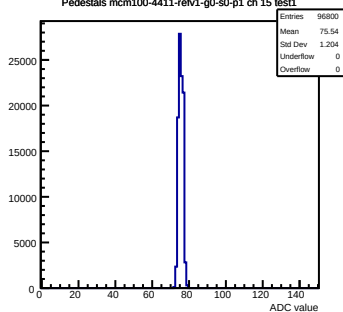
Pedestals mcm100-4411-refv1-g0-s0-p1 ch 15 test1
