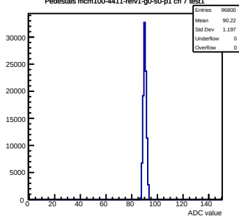
Pedestals mcm100-4411-refv1-g0-s0-p1 ch 7 test1
