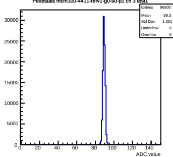
Pedestals mcm100-4411-refv1-g0-s0-p1 ch 3 test1
