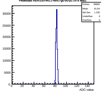
Pedestals mcm100-4411-refv1-g0-s0-p1 ch 6 test1
