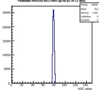
Pedestals mcm100-4411-refv1-g0-s0-p1 ch 11 test1
