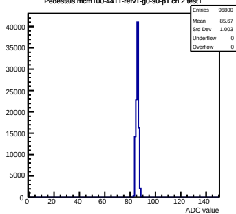
Pedestals mcm100-4411-refv1-g0-s0-p1 ch 2 test1
