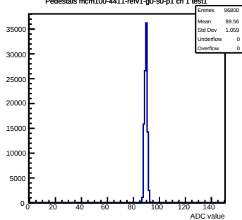
Pedestals mcm100-4411-refv1-g0-s0-p1 ch 1 test1
