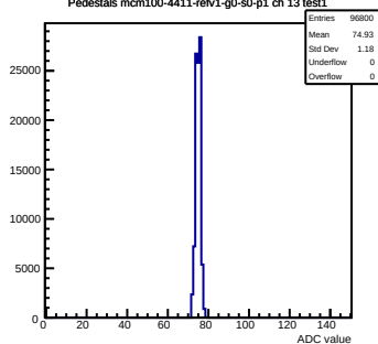
Pedestals mcm100-4411-refv1-g0-s0-p1 ch 13 test1
