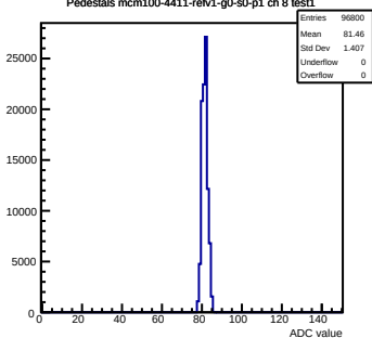
Pedestals mcm100-4411-refv1-g0-s0-p1 ch 8 test1
