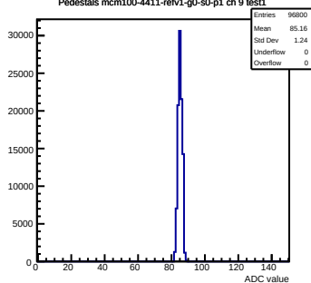
Pedestals mcm100-4411-refv1-g0-s0-p1 ch 9 test1
