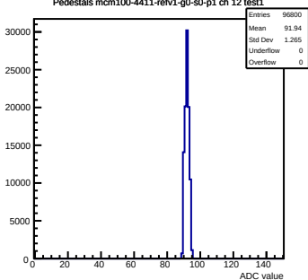
Pedestals mcm100-4411-refv1-g0-s0-p1 ch 12 test1
