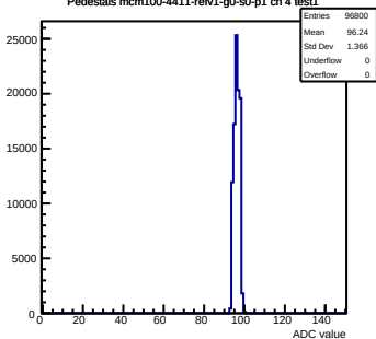
Pedestals mcm100-4411-refv1-g0-s0-p1 ch 4 test1
