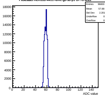
Pedestals mcm100-4411-refv2-g0-s0-p1 ch 78 test1
