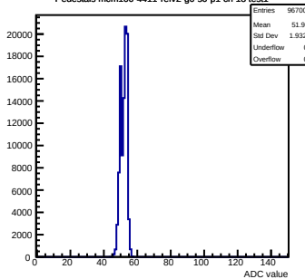
Pedestals mcm100-4411-refv2-g0-s0-p1 ch 18 test1
