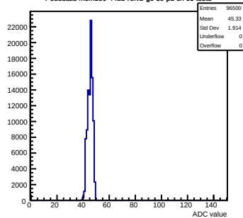
Pedestals mcm100-4411-refv2-g0-s0-p1 ch 63 test1
