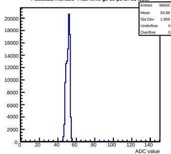
Pedestals mcm100-4411-refv2-g0-s0-p1 ch 53 test1
