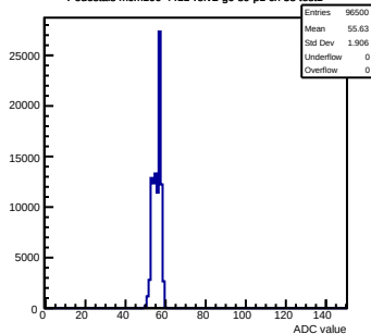
Pedestals mcm100-4411-refv2-g0-s0-p1 ch 58 test1
