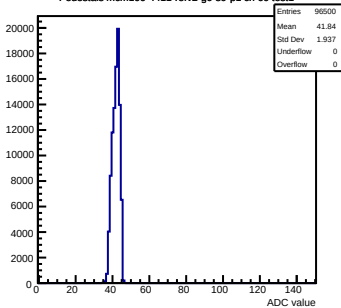
Pedestals mcm100-4411-refv2-g0-s0-p1 ch 60 test1
