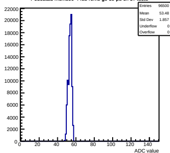
Pedestals mcm100-4411-refv2-g0-s0-p1 ch 57 test1
