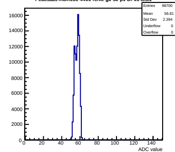
Pedestals mcm100-4411-refv2-g0-s0-p1 ch 16 test1
