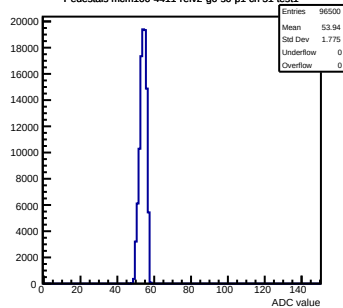
Pedestals mcm100-4411-refv2-g0-s0-p1 ch 51 test1
