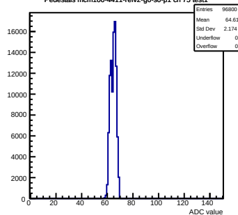
Pedestals mcm100-4411-refv2-g0-s0-p1 ch 75 test1
