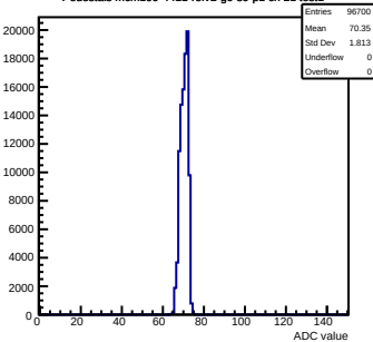
Pedestals mcm100-4411-refv2-g0-s0-p1 ch 21 test1
