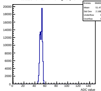
Pedestals mcm100-4411-refv2-g0-s0-p1 ch 15 test1
