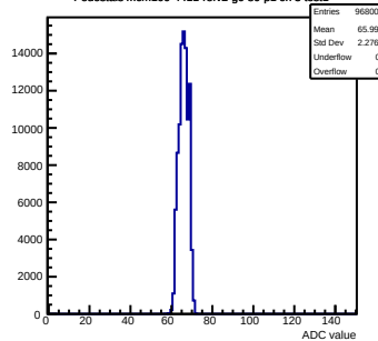
Pedestals mcm100-4411-refv2-g0-s0-p1 ch 3 test1
