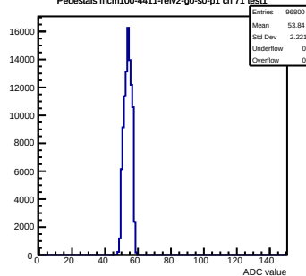
Pedestals mcm100-4411-refv2-g0-s0-p1 ch 71 test1
