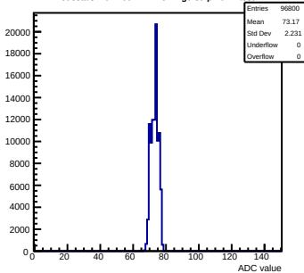
Pedestals mcm100-4411-refv2-g0-s0-p1 ch 4 test1
