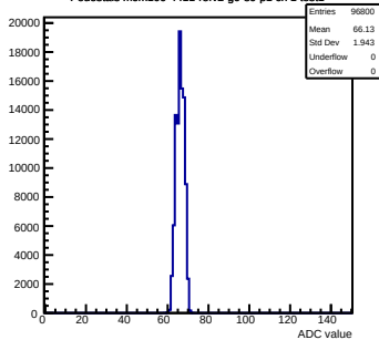
Pedestals mcm100-4411-refv2-g0-s0-p1 ch 1 test1
