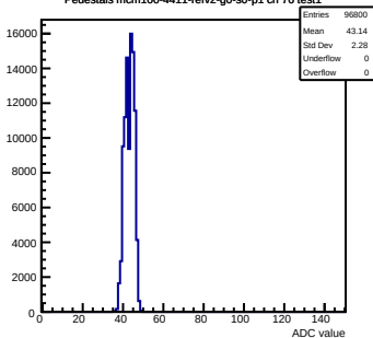
Pedestals mcm100-4411-refv2-g0-s0-p1 ch 76 test1
