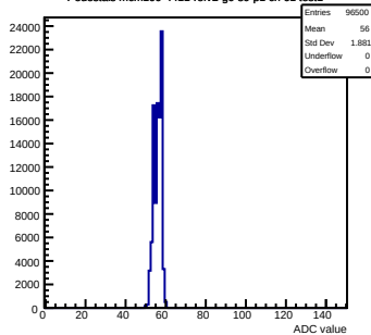
Pedestals mcm100-4411-refv2-g0-s0-p1 ch 61 test1
