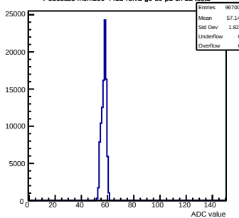
Pedestals mcm100-4411-refv2-g0-s0-p1 ch 22 test1
