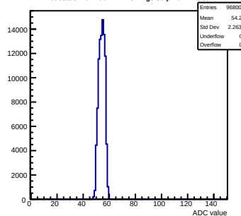
Pedestals mcm100-4411-refv2-g0-s0-p1 ch 11 test1
