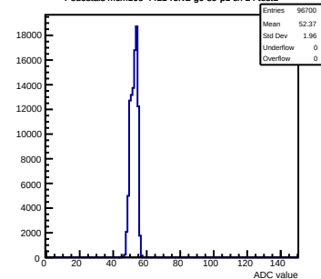
Pedestals mcm100-4411-refv2-g0-s0-p1 ch 24 test1
