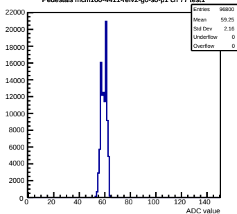
Pedestals mcm100-4411-refv2-g0-s0-p1 ch 77 test1
