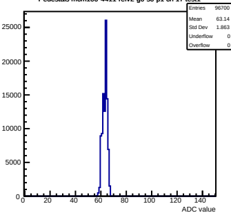
Pedestals mcm100-4411-refv2-g0-s0-p1 ch 17 test1
