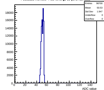
Pedestals mcm100-4411-refv2-g0-s0-p1 ch 28 test1
