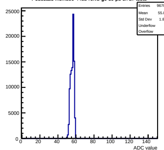
Pedestals mcm100-4411-refv2-g0-s0-p1 ch 27 test1
