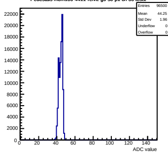
Pedestals mcm100-4411-refv2-g0-s0-p1 ch 50 test1
