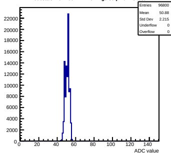
Pedestals mcm100-4411-refv2-g0-s0-p1 ch 13 test1
