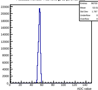
Pedestals mcm100-4411-refv2-g0-s0-p1 ch 25 test1
