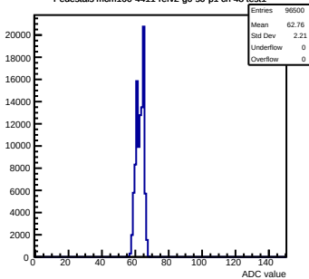
Pedestals mcm100-4411-refv2-g0-s0-p1 ch 48 test1
