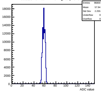
Pedestals mcm100-4411-refv2-g0-s0-p1 ch 6 test1
