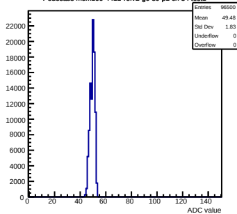
Pedestals mcm100-4411-refv2-g0-s0-p1 ch 54 test1
