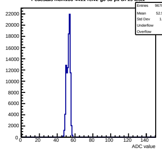
Pedestals mcm100-4411-refv2-g0-s0-p1 ch 19 test1
