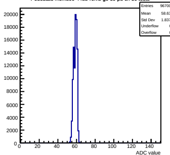
Pedestals mcm100-4411-refv2-g0-s0-p1 ch 30 test1
