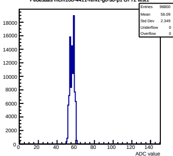
Pedestals mcm100-4411-refv2-g0-s0-p1 ch 72 test1
