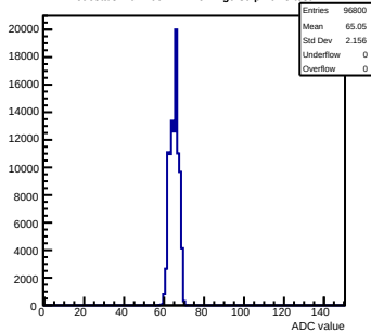
Pedestals mcm100-4411-refv2-g0-s0-p1 ch 5 test1
