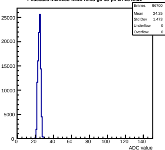
Pedestals mcm100-4411-refv3-g0-s0-p1 ch 16 test1
