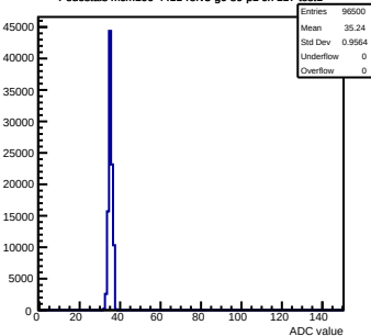
Pedestals mcm100-4411- rev3-g0-s0-p1 ch 117 test1
