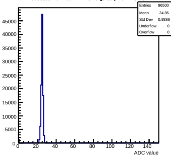
Pedestals mcm100-4411- rev3-g0-s0-p1 ch 123 test1
