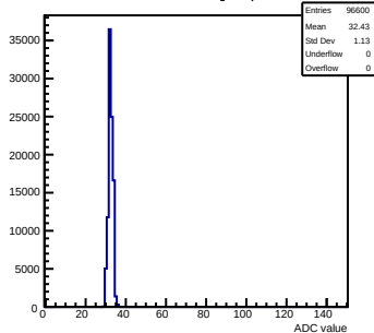
Pedestals mcm100-4411-refv3-g0-s0-p1 ch 110 test1
