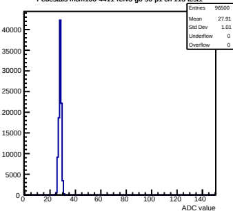
Pedestals mcm100-4411- rev3-g0-s0-p1 ch 113 test1
