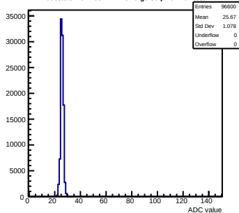
Pedestals mcm100-4411-refv3-g0-s0-p1 ch 102 test1
