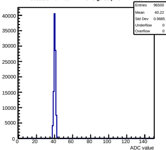
Pedestals mcm100-4411- rev3-g0-s0-p1 ch 122 test1
