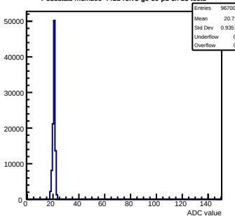
Pedestals mcm100-4411-refv3-g0-s0-p1 ch 25 test1
