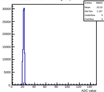
Pedestals mcm100-4411-refv3-g0-s0-p1 ch 101 test1
