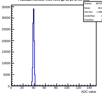
Pedestals mcm100-4411-refv3-g0-s0-p1 ch 21 test1
