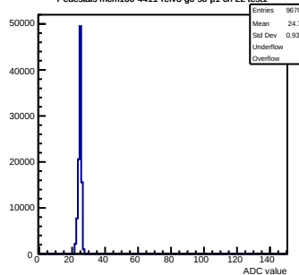
Pedestals mcm100-4411-refv3-g0-s0-p1 ch 22 test1
