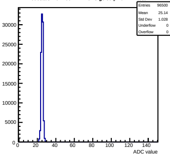
Pedestals mcm100-4411- rev3-g0-s0-p1 ch 127 test1
