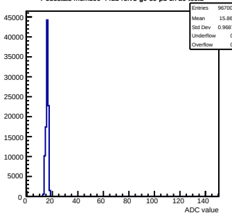
Pedestals mcm100-4411-refv3-g0-s0-p1 ch 29 test1
