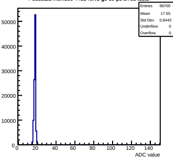
Pedestals mcm100-4411-refv3-g0-s0-p1 ch 28 test1
