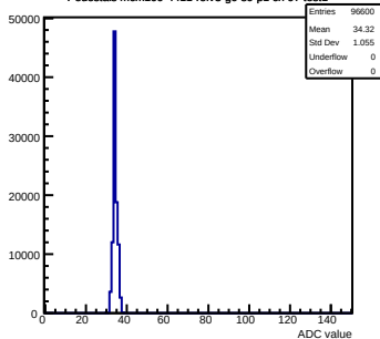
Pedestals mcm100-4411-refv3-g0-s0-p1 ch 97 test1
