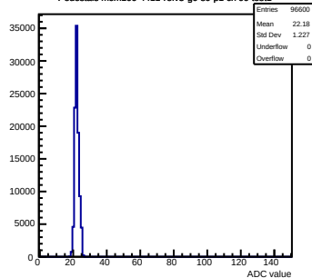
Pedestals mcm100-4411-refv3-g0-s0-p1 ch 99 test1
