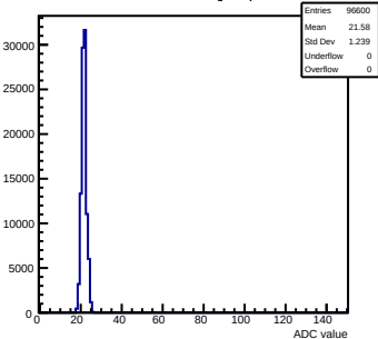
Pedestals mcm100-4411-refv3-g0-s0-p1 ch 104 test1
