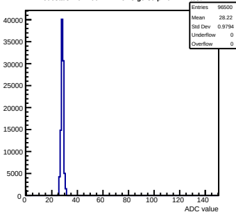
Pedestals mcm100-4411- rev3-g0-s0-p1 ch 124 test1
