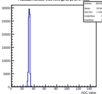
Pedestals mcm100-4411-refv3-g0-s0-p1 ch 17 test1
