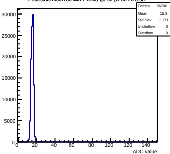
Pedestals mcm100-4411-refv3-g0-s0-p1 ch 20 test1
