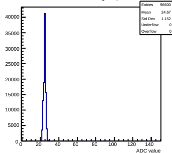
Pedestals mcm100-4411-refv3-g0-s0-p1 ch 111 test1
