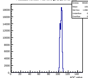
Pedestals mcm100-4411-rlv6-g0-s0-p1 ch 59 test1
