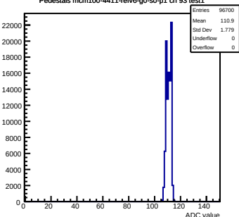
Pedestals mcm100-4411-rlv6-g0-s0-p1 ch 93 test1
