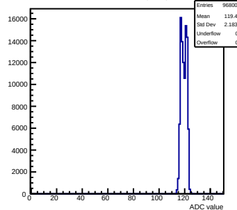
Pedestals mcm100-4411-rlv6-g0-s0-p1 ch 3 test1
