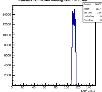
Pedestals mcm100-4411-rlv6-g0-s0-p1 ch 78 test1
