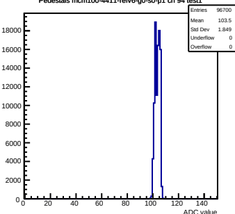
Pedestals mcm100-4411-rlv6-g0-s0-p1 ch 94 test1
