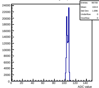
Pedestals mcm100-4411-rlv6-g0-s0-p1 ch 31 test1
