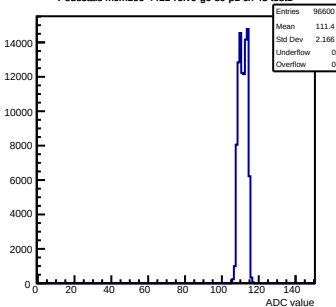
Pedestals mcm100-4411-rlv6-g0-s0-p1 ch 43 test1
