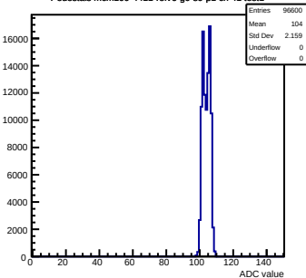
Pedestals mcm100-4411-rlv6-g0-s0-p1 ch 41 test1
