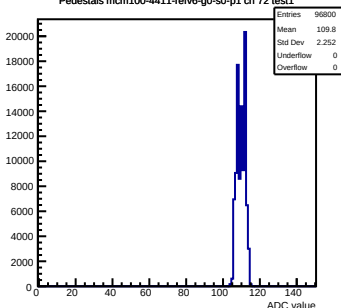
Pedestals mcm100-4411-rlv6-g0-s0-p1 ch 72 test1
