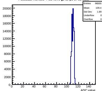
Pedestals mcm100-4411-rlv6-g0-s0-p1 ch 61 test1
