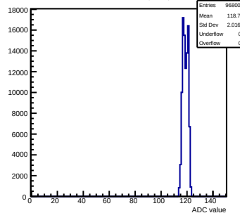
Pedestals mcm100-4411-rlv6-g0-s0-p1 ch 7 test1
