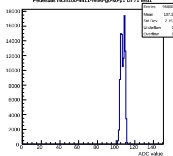
Pedestals mcm100-4411-rlv6-g0-s0-p1 ch 71 test1
