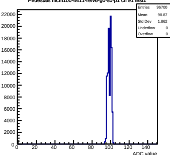
Pedestals mcm100-4411-rlv6-g0-s0-p1 ch 91 test1
