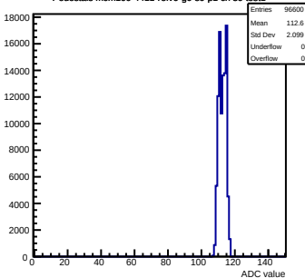
Pedestals mcm100-4411-rlv6-g0-s0-p1 ch 39 test1
