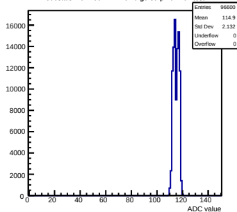
Pedestals mcm100-4411-rlv6-g0-s0-p1 ch 107 test1
