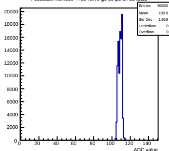
Pedestals mcm100-4411-rlv6-g0-s0-p1 ch 58 test1
