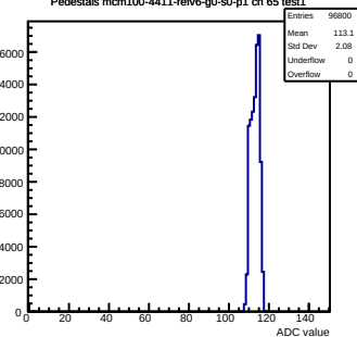
Pedestals mcm100-4411-rlv6-g0-s0-p1 ch 65 test1
