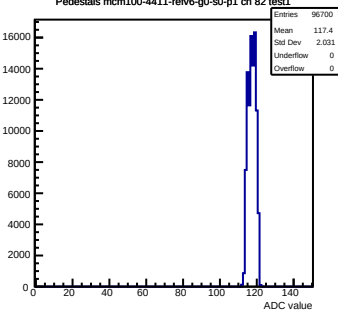
Pedestals mcm100-4411-rlv6-g0-s0-p1 ch 82 test1
