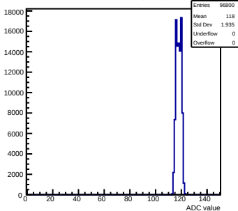
Pedestals mcm100-4411-rlv6-g0-s0-p1 ch 1 test1
