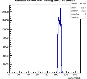
Pedestals mcm100-4411-rlv6-g0-s0-p1 ch 80 test1
