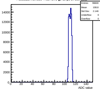
Pedestals mcm100-4411-rlv6-g0-s0-p1 ch 100 test1
