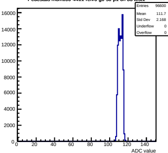
Pedestals mcm100-4411-rlv6-g0-s0-p1 ch 33 test1
