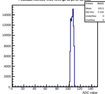
Pedestals mcm100-4411-rlv6-g0-s0-p1 ch 98 test1
