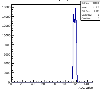
Pedestals mcm100-4411-rlv6-g0-s0-p1 ch 106 test1
