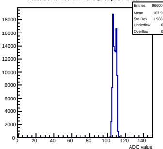
Pedestals mcm100-4411-rlv6-g0-s0-p1 ch 47 test1
