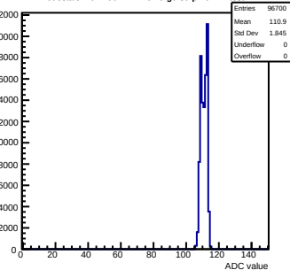
Pedestals mcm100-4411-rlv6-g0-s0-p1 ch 22 test1
