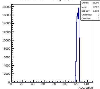
Pedestals mcm100-4411-rlv6-g0-s0-p1 ch 21 test1
