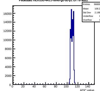
Pedestals mcm100-4411-rlv6-g0-s0-p1 ch 79 test1
