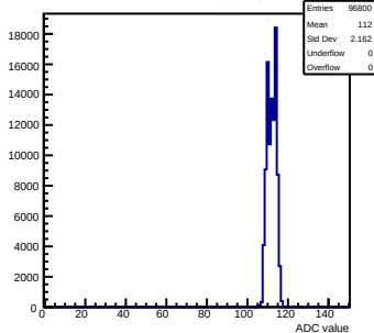
Pedestals mcm100-4411-rlv6-g0-s0-p1 ch 6 test1
