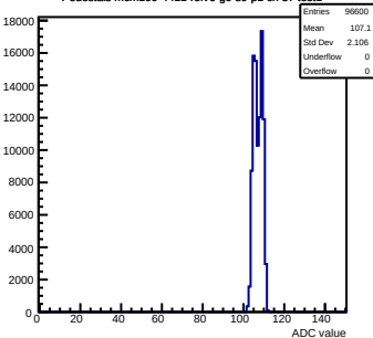
Pedestals mcm100-4411-rlv6-g0-s0-p1 ch 37 test1
