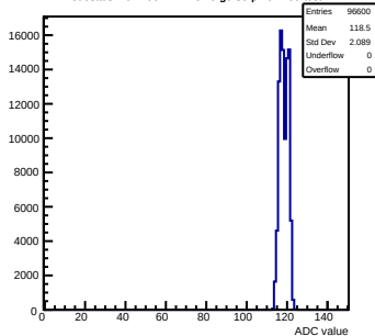
Pedestals mcm100-4411-rlv6-g0-s0-p1 ch 109 test1
