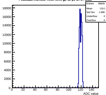
Pedestals mcm100-4411-rlv6-g0-s0-p1 ch 97 test1
