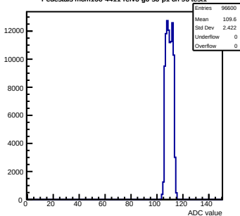
Pedestals mcm100-4411-rlv6-g0-s0-p1 ch 96 test1
