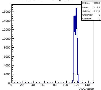
Pedestals mcm100-4411-rlv6-g0-s0-p1 ch 110 test1
