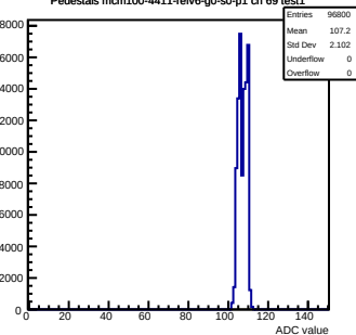
Pedestals mcm100-4411-rlv6-g0-s0-p1 ch 69 test1
