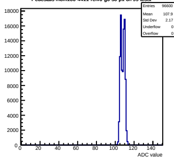
Pedestals mcm100-4411-rlv6-g0-s0-p1 ch 99 test1
