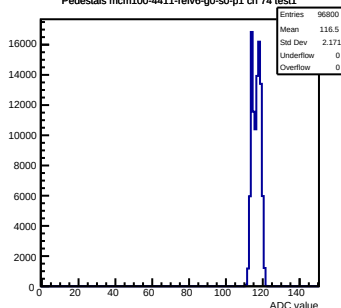
Pedestals mcm100-4411-rlv6-g0-s0-p1 ch 74 test1
