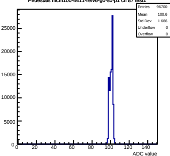
Pedestals mcm100-4411-rlv6-g0-s0-p1 ch 87 test1
