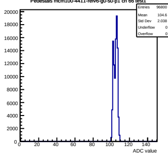
Pedestals mcm100-4411-rlv6-g0-s0-p1 ch 66 test1
