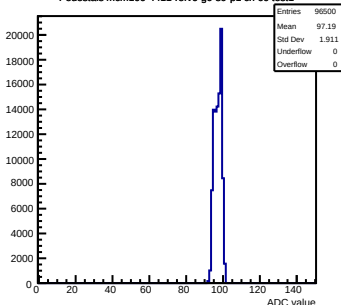
Pedestals mcm100-4411-rlv6-g0-s0-p1 ch 60 test1
