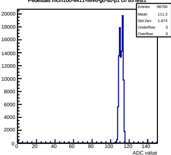
Pedestals mcm100-4411-rlv6-g0-s0-p1 ch 85 test1
