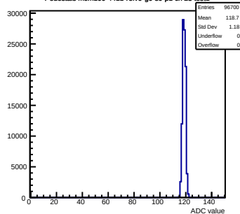
Pedestals mcm100-4411-rfv0-g0-s0-p1 ch 23 test1
