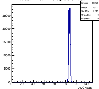
Pedestals mcm100-4411-rfv0-g0-s0-p1 ch 18 test1
