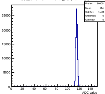
Pedestals mcm100-4411-rv0-g0-s0-p1 ch 44 test1
