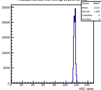
Pedestals mcm100-4411-rv0-g0-s0-p1 ch 36 test1
