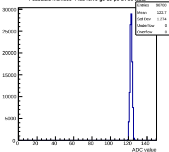
Pedestals mcm100-4411-rfv0-g0-s0-p1 ch 21 test1
