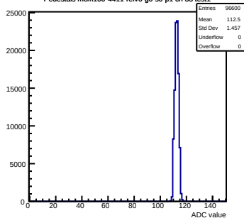
Pedestals mcm100-4411-rv0-g0-s0-p1 ch 33 test1
