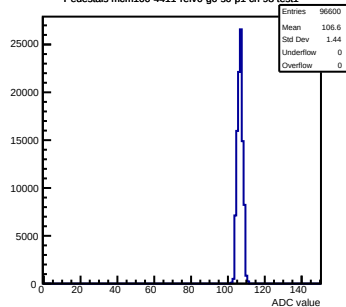
Pedestals mcm100-4411-refV0-g0-s0-p1 ch 98 test1
