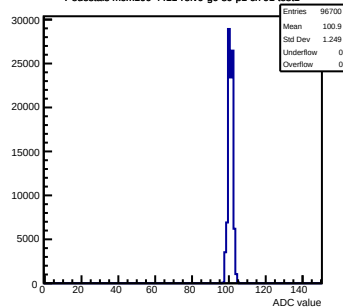
Pedestals mcm100-4411-rev0-g0-s0-p1 ch 91 test1
