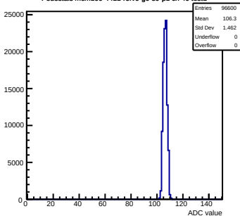
Pedestals mcm100-4411-rv0-g0-s0-p1 ch 40 test1
