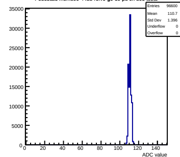
Pedestals mcm100-4411-refV0-g0-s0-p1 ch 108 test1
