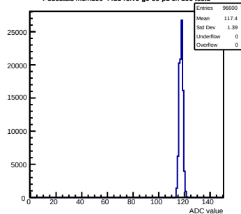
Pedestals mcm100-4411-refV0-g0-s0-p1 ch 106 test1
