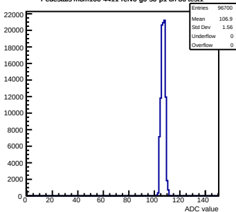
Pedestals mcm100-4411-rev0-g0-s0-p1 ch 80 test1
