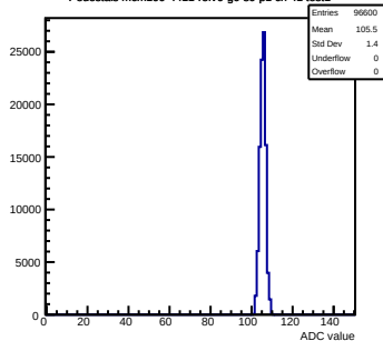
Pedestals mcm100-4411-rv0-g0-s0-p1 ch 41 test1
