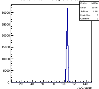
Pedestals mcm100-4411-rev0-g0-s0-p1 ch 88 test1
