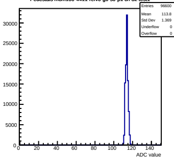
Pedestals mcm100-4411-rv0-g0-s0-p1 ch 32 test1
