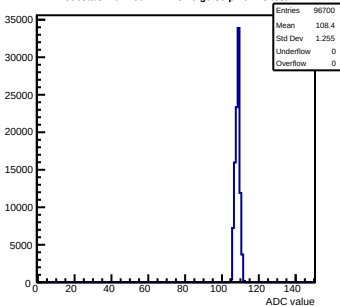
Pedestals mcm100-4411-rfv0-g0-s0-p1 ch 25 test1
