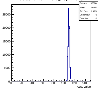
Pedestals mcm100-4411-rv0-g0-s0-p1 ch 45 test1
