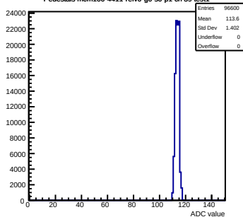
Pedestals mcm100-4411-rv0-g0-s0-p1 ch 39 test1
