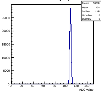
Pedestals mcm100-4411-rfv0-g0-s0-p1 ch 24 test1
