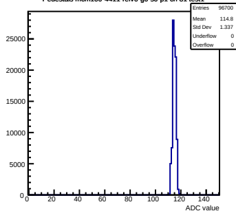
Pedestals mcm100-4411-rev0-g0-s0-p1 ch 81 test1
