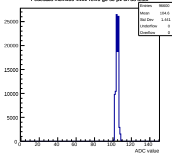
Pedestals mcm100-4411-rv0-g0-s0-p1 ch 38 test1
