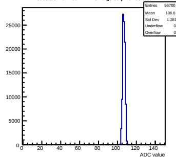
Pedestals mcm100-4411-rev0-g0-s0-p1 ch 95 test1
