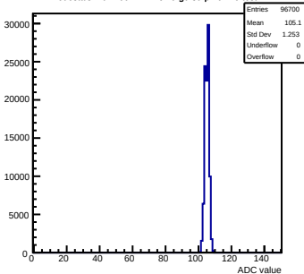
Pedestals mcm100-4411-rfv0-g0-s0-p1 ch 29 test1
