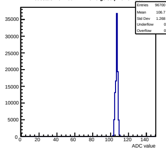
Pedestals mcm100-4411-rfv0-g0-s0-p1 ch 31 test1
