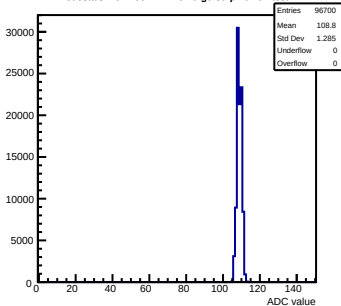
Pedestals mcm100-4411-rev0-g0-s0-p1 ch 92 test1
