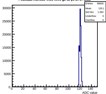
Pedestals mcm100-4411-refV0-g0-s0-p1 ch 97 test1
