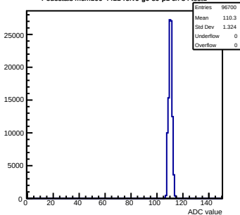
Pedestals mcm100-4411-rev0-g0-s0-p1 ch 84 test1
