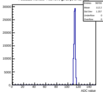
Pedestals mcm100-4411-rev0-g0-s0-p1 ch 85 test1
