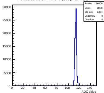
Pedestals mcm100-4411-rv0-g0-s0-p1 ch 42 test1
