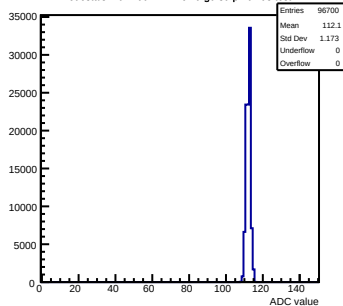
Pedestals mcm100-4411-rev0-g0-s0-p1 ch 93 test1
