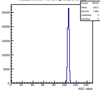
Pedestals mcm100-4411-rfv0-g0-s0-p1 ch 20 test1
