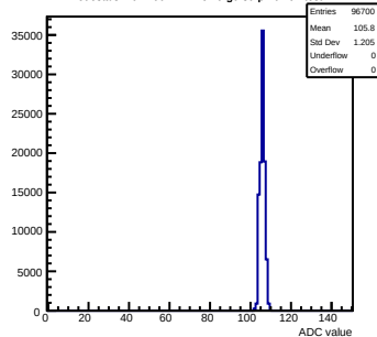
Pedestals mcm100-4411-rev0-g0-s0-p1 ch 94 test1
