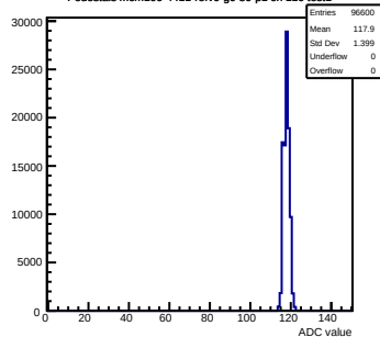
Pedestals mcm100-4411-refV0-g0-s0-p1 ch 110 test1
