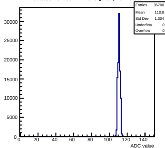
Pedestals mcm100-4411-rfv0-g0-s0-p1 ch 26 test1
