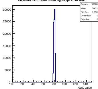
Pedestals mcm100-4411-rv1-g0-s0-p1 ch 47 test1
