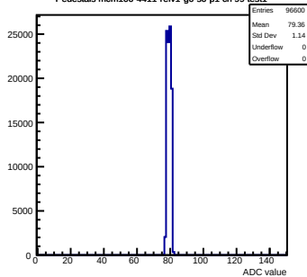
Pedestals mcm100-4411- \text{refV1-g0-s0-p1} ch 99 test1
