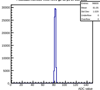
Pedestals mcm100-4411- \text{refV1-g0-s0-p1} ch 100 test1
