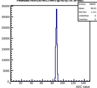
Pedestals mcm100-4411-rv1-g0-s0-p1 ch 36 test1
