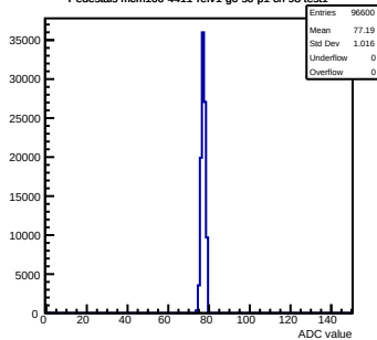
Pedestals mcm100-4411- \text{refV1-g0-s0-p1} ch 98 test1
