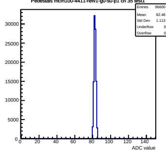
Pedestals mcm100-4411-rv1-g0-s0-p1 ch 35 test1
