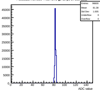
Pedestals mcm100-4411- \text{refV1-g0-s0-p1} ch 108 test1
