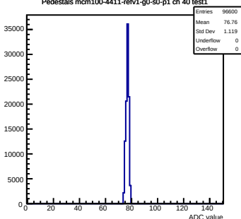
Pedestals mcm100-4411-rv1-g0-s0-p1 ch 40 test1
