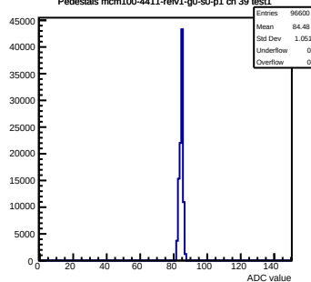
Pedestals mcm100-4411-rv1-g0-s0-p1 ch 39 test1
