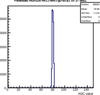
Pedestals mcm100-4411-rv1-g0-s0-p1 ch 37 test1
