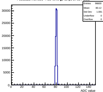
Pedestals mcm100-4411- \text{refV1-g0-s0-p1} ch 104 test1
