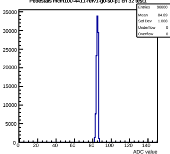
Pedestals mcm100-4411-g0-s0-p1 ch 32 test1
