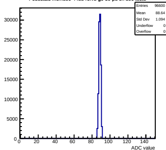
Pedestals mcm100-4411- \text{refV1-g0-s0-p1} ch 106 test1
