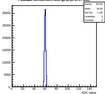
Pedestals mcm100-4411-refv2-g0-s0-p1 ch 27 test1
