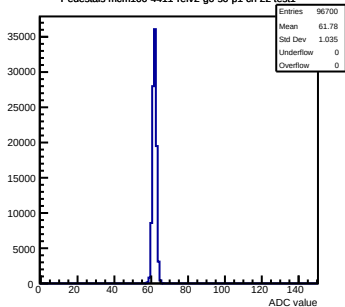
Pedestals mcm100-4411-refv2-g0-s0-p1 ch 22 test1
