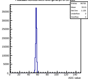
Pedestals mcm100-4411-refv2-g0-s0-p1 ch 31 test1
