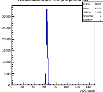
Pedestals mcm100-4411-refv2-g0-s0-p1 ch 30 test1
