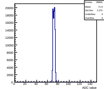
Pedestals mcm100-4411-refv2-g0-s0-p1 ch 0 test1
