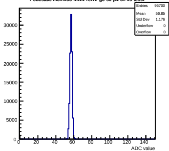
Pedestals mcm100-4411-refv2-g0-s0-p1 ch 19 test1
