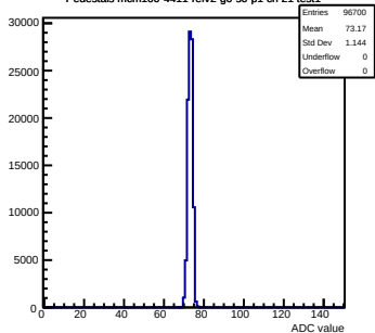
Pedestals mcm100-4411-refv2-g0-s0-p1 ch 21 test1
