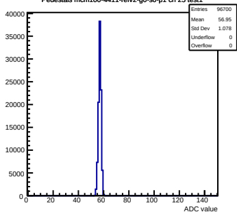
Pedestals mcm100-4411-refv2-g0-s0-p1 ch 25 test1
