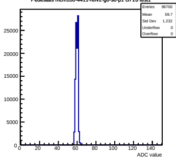
Pedestals mcm100-4411-refv2-g0-s0-p1 ch 26 test1
