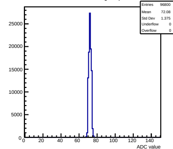
Pedestals mcm100-4411-refv2-g0-s0-p1 ch 12 test1
