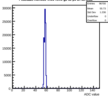
Pedestals mcm100-4411-refv2-g0-s0-p1 ch 18 test1
