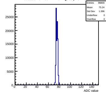
Pedestals mcm100-4411-refv2-g0-s0-p1 ch 4 test1
