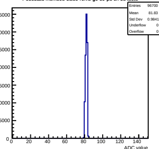
Pedestals mcm101-5E10-refV2-g0-s0-p1 ch 31 test1
