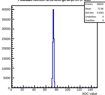
Pedestals mcm101-5E10-refv2-g0-s0-p1 ch 57 test1
