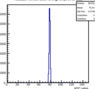
Pedestals mcm101-5E10-refV2-g0-s0-p1 ch 26 test1
