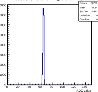
Pedestals mcm101-5E10-refV2-g0-s0-p1 ch 22 test1
