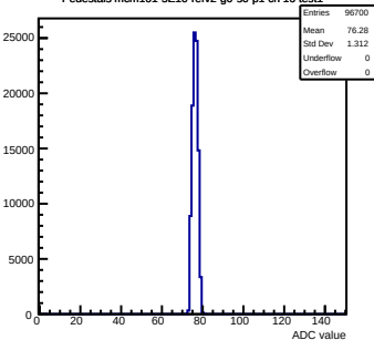
Pedestals mcm101-5E10-refV2-g0-s0-p1 ch 16 test1
