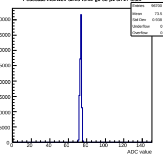
Pedestals mcm101-5E10-refV2-g0-s0-p1 ch 17 test1
