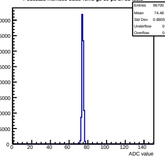
Pedestals mcm101-5E10-refV2-g0-s0-p1 ch 23 test1
