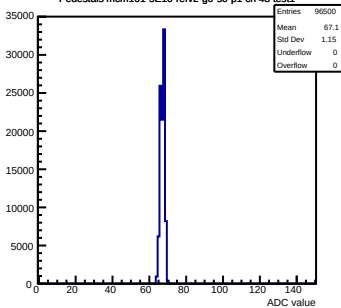
Pedestals mcm101-5E10-refv2-g0-s0-p1 ch 48 test1
