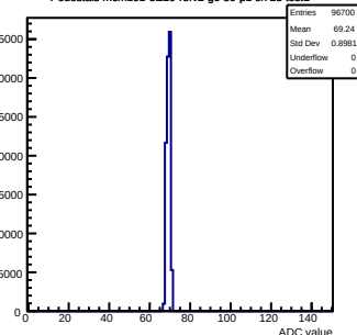
Pedestals mcm101-5E10-refV2-g0-s0-p1 ch 25 test1
