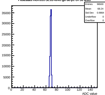
Pedestals mcm101-5E10-refv2-g0-s0-p1 ch 56 test1
