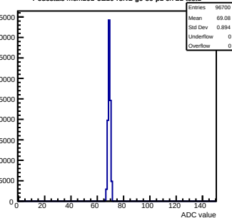
Pedestals mcm101-5E10-refV2-g0-s0-p1 ch 21 test1
