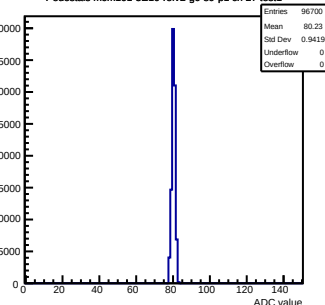
Pedestals mcm101-5E10-refV2-g0-s0-p1 ch 27 test1
