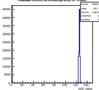
Pedestals mcm101-5E10-refv6-g0-s0-p1 ch 79 test1
