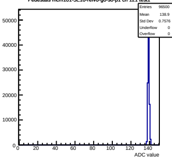
Pedestals mcm101-5E10-refV6-g0-s0-p1 ch 121 test1
