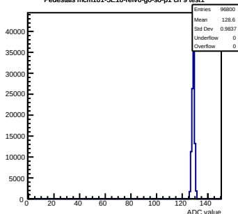
Pedestals mcm101-5E10-relv6-g0-s0-p1 ch 9 test1
