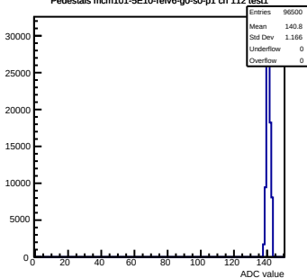
Pedestals mcm101-5E10-refV6-g0-s0-p1 ch 112 test1
