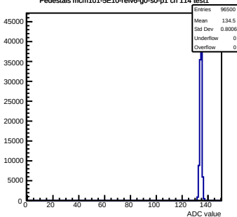
Pedestals mcm101-5E10-refV6-g0-s0-p1 ch 114 test1
