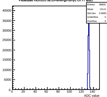
Pedestals mcm101-5E10-refv6-g0-s0-p1 ch 77 test1
