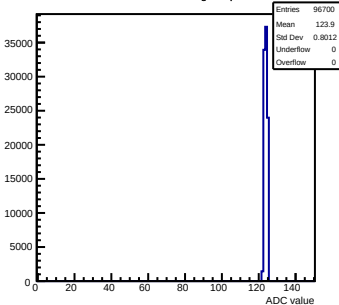
Pedestals mcm101-5E10-refv6-g0-s0-p1 ch 95 test1
