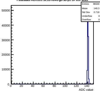
Pedestals mcm101-5E10-refV6-g0-s0-p1 ch 122 test1
