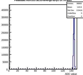
Pedestals mcm101-5E10-refv6-g0-s0-p1 ch 76 test1
