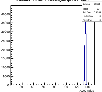
Pedestals mcm101-5E10-refV6-g0-s0-p1 ch 115 test1
