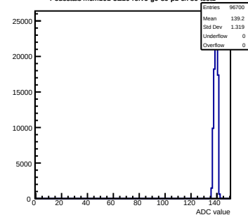
Pedestals mcm101-5E10-refv6-g0-s0-p1 ch 80 test1
