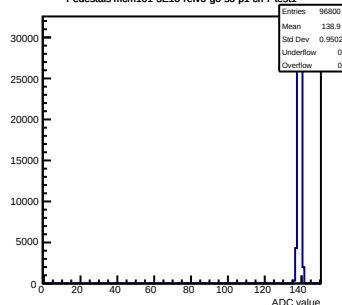
Pedestals mcm101-5E10-relv6-g0-s0-p1 ch 7 test1
