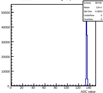
Pedestals mcm101-5E10-refv6-g0-s0-p1 ch 87 test1
