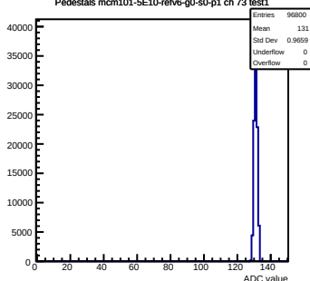
Pedestals mcm101-5E10-refv6-g0-s0-p1 ch 73 test1
