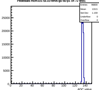
Pedestals mcm101-5E10-refv6-g0-s0-p1 ch 72 test1
