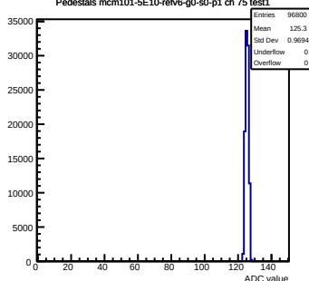
Pedestals mcm101-5E10-refv6-g0-s0-p1 ch 75 test1
