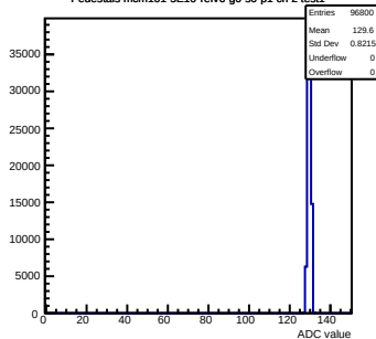
Pedestals mcm101-5E10-relv6-g0-s0-p1 ch 2 test1
