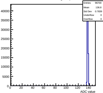
Pedestals mcm101-5E10-refv6-g0-s0-p1 ch 93 test1
