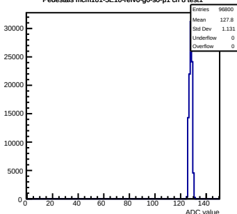
Pedestals mcm101-5E10-relv6-g0-s0-p1 ch 8 test1
