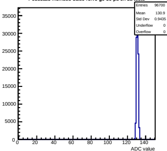
Pedestals mcm101-5E10-refv6-g0-s0-p1 ch 82 test1
