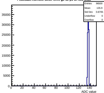
Pedestals mcm101-5E10-refV6-g0-s0-p1 ch 116 test1
