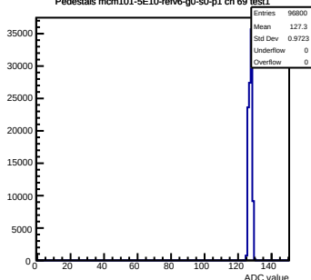
Pedestals mcm101-5E10-refv6-g0-s0-p1 ch 69 test1
