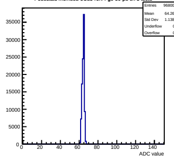
Pedestals mcm102-5C13-refV4-g0-s0-p1 ch 3 test1
