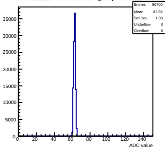
Pedestals mcm102-5C13-refv4-g0-s0-p1 ch 20 test1
