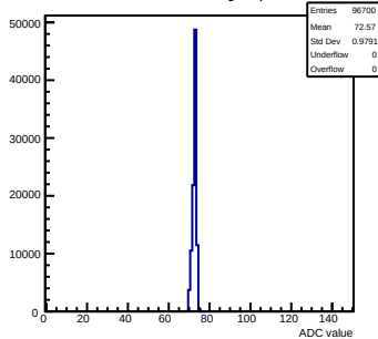
Pedestals mcm102-5C13-refv4-g0-s0-p1 ch 30 test1
