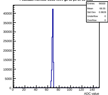
Pedestals mcm102-5C13-refV4-g0-s0-p1 ch 51 test1
