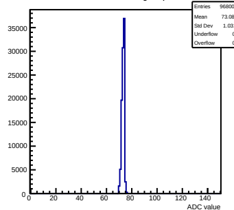
Pedestals mcm102-5C13-refV4-g0-s0-p1 ch 15 test1
