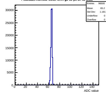
Pedestals mcm102-5C13-refV4-g0-s0-p1 ch 48 test1
