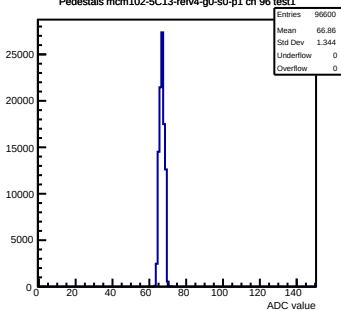
Pedestals mcm102-5C13-refV4-g0-s0-p1 ch 96 test1
