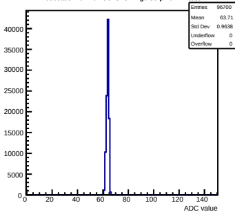
Pedestals mcm102-5C13-refv4-g0-s0-p1 ch 24 test1
