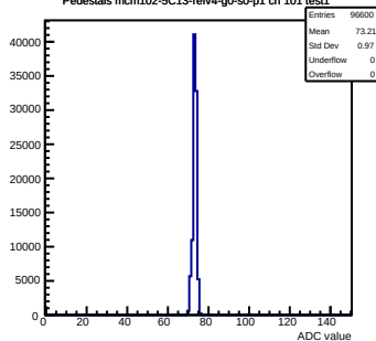
Pedestals mcm102-5C13-refV4-g0-s0-p1 ch 101 test1
