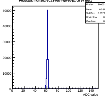
Pedestals mcm102-5C13-refV4-g0-s0-p1 ch 97 test1
