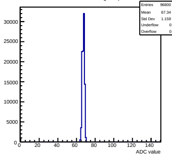
Pedestals mcm102-5C13-refV4-g0-s0-p1 ch 14 test1
