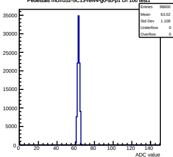
Pedestals mcm102-5C13-refV4-g0-s0-p1 ch 100 test1
