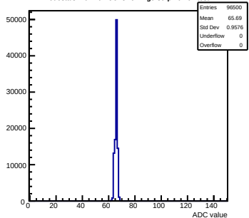
Pedestals mcm102-5C13-refV4-g0-s0-p1 ch 61 test1
