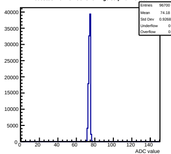
Pedestals mcm102-5C13-refv4-g0-s0-p1 ch 25 test1
