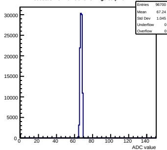
Pedestals mcm102-5C13-refv4-g0-s0-p1 ch 22 test1
