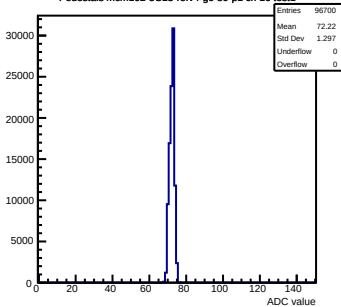
Pedestals mcm102-5C13-refv4-g0-s0-p1 ch 16 test1
