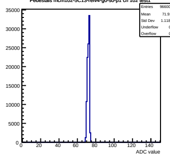
Pedestals mcm102-5C13-refV4-g0-s0-p1 ch 102 test1
