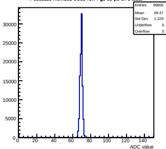
Pedestals mcm102-5C13-refV4-g0-s0-p1 ch 0 test1
