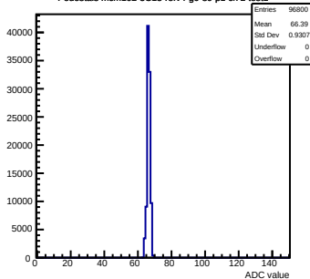
Pedestals mcm102-5C13-refV4-g0-s0-p1 ch 2 test1
