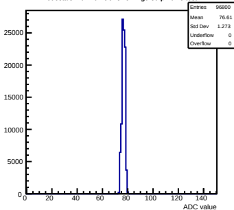
Pedestals mcm102-5C13-refV4-g0-s0-p1 ch 8 test1
