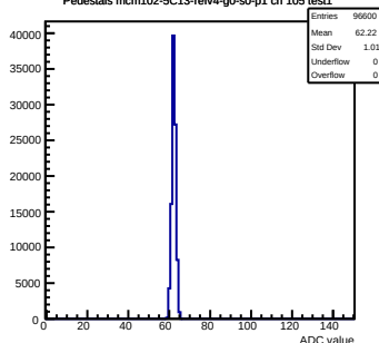
Pedestals mcm102-5C13-refV4-g0-s0-p1 ch 105 test1
