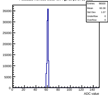
Pedestals mcm102-5C13-refV4-g0-s0-p1 ch 58 test1
