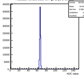
Pedestals mcm102-5C13-refv4-g0-s0-p1 ch 19 test1
