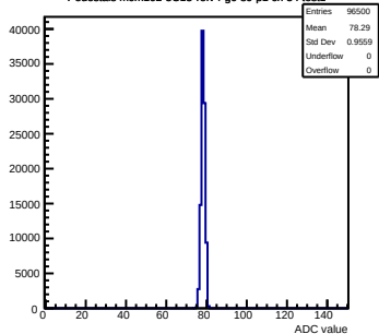
Pedestals mcm102-5C13-refV4-g0-s0-p1 ch 54 test1
