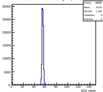
Pedestals mcm102-5C13-refV4-g0-s0-p1 ch 5 test1
