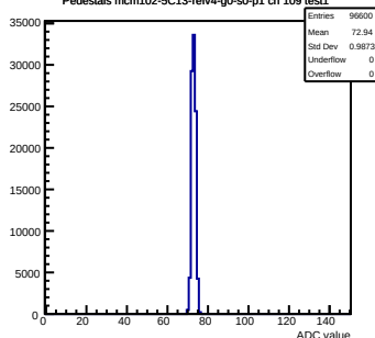
Pedestals mcm102-5C13-refV4-g0-s0-p1 ch 109 test1
