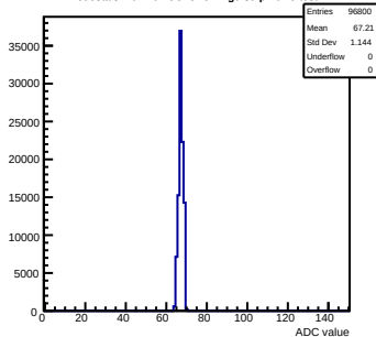
Pedestals mcm102-5C13-refV4-g0-s0-p1 ch 9 test1
