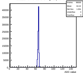
Pedestals mcm102-5C13-refV4-g0-s0-p1 ch 62 test1
