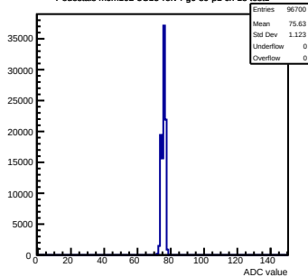
Pedestals mcm102-5C13-refv4-g0-s0-p1 ch 18 test1
