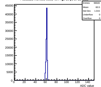
Pedestals mcm102-5C13-refV4-g0-s0-p1 ch 52 test1
