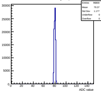
Pedestals mcm102-5C13-refV4-g0-s0-p1 ch 12 test1
