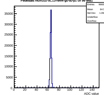
Pedestals mcm102-5C13-refV4-g0-s0-p1 ch 99 test1
