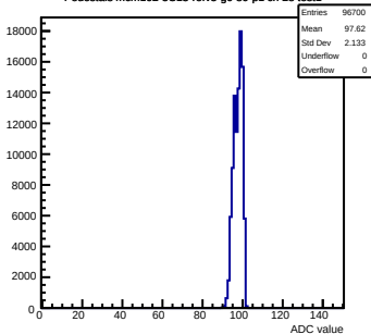
Pedestals mcm102-5C13-refV5-g0-s0-p1 ch 28 test1
