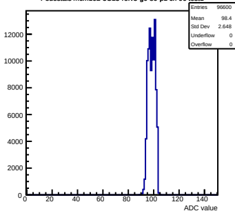
Pedestals mcm102-5C13-refV5-g0-s0-p1 ch 96 test1
