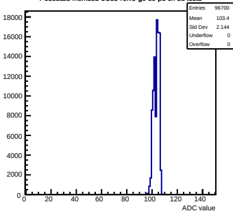
Pedestals mcm102-5C13-refV5-g0-s0-p1 ch 31 test1
