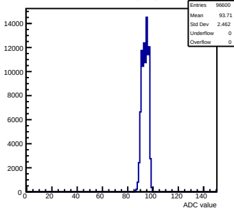
Pedestals mcm102-5C13-refV5-g0-s0-p1 ch 100 test1
