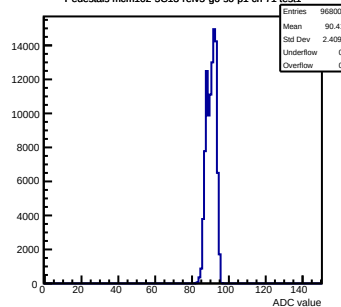
Pedestals mcm102-5C13-refV5-g0-s0-p1 ch 71 test1
