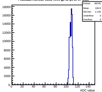
Pedestals mcm102-5C13-refV5-g0-s0-p1 ch 17 test1
