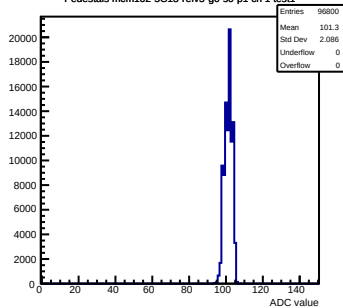
Pedestals mcm102-5C13-reV5-g0-s0-p1 ch 1 test1
