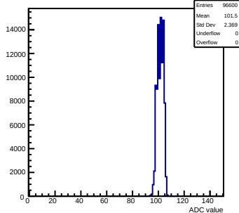
Pedestals mcm102-5C13-refV5-g0-s0-p1 ch 110 test1
