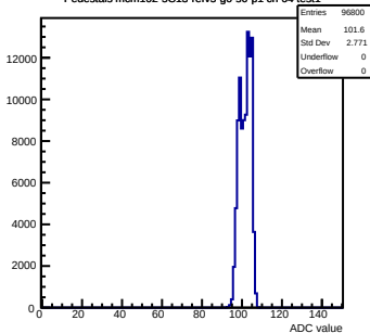
Pedestals mcm102-5C13-refV5-g0-s0-p1 ch 64 test1
