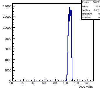
Pedestals mcm102-5C13-refV5-g0-s0-p1 ch 111 test1
