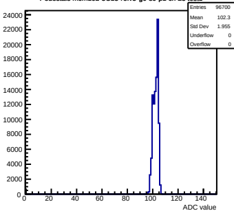
Pedestals mcm102-5C13-refV5-g0-s0-p1 ch 23 test1
