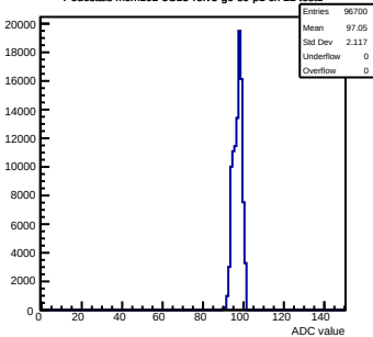
Pedestals mcm102-5C13-refV5-g0-s0-p1 ch 22 test1
