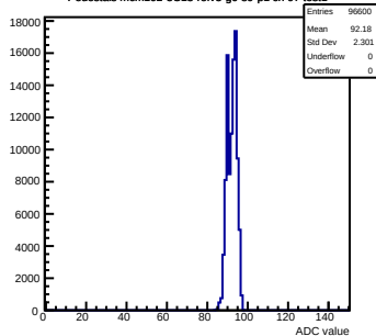
Pedestals mcm102-5C13-refV5-g0-s0-p1 ch 97 test1
