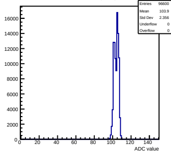
Pedestals mcm102-5C13-refV5-g0-s0-p1 ch 101 test1
