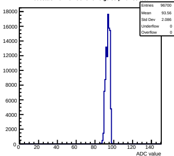
Pedestals mcm102-5C13-refV5-g0-s0-p1 ch 88 test1
