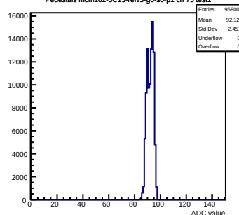
Pedestals mcm102-5C13-refV5-g0-s0-p1 ch 75 test1
