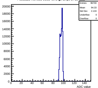
Pedestals mcm102-5C13-refV5-g0-s0-p1 ch 82 test1
