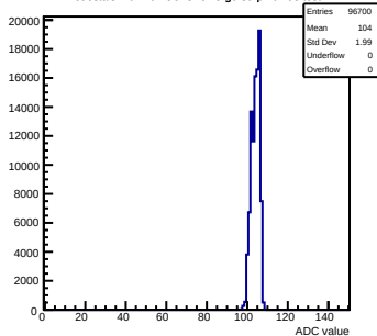
Pedestals mcm102-5C13-refV5-g0-s0-p1 ch 93 test1
