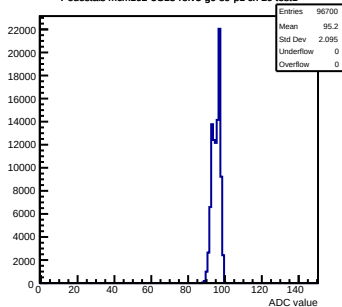
Pedestals mcm102-5C13-refV5-g0-s0-p1 ch 29 test1
