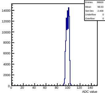
Pedestals mcm102-5C13-refV5-g0-s0-p1 ch 108 test1
