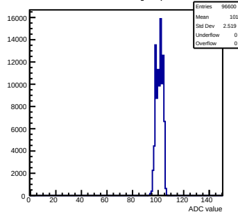
Pedestals mcm102-5C13-refV5-g0-s0-p1 ch 107 test1
