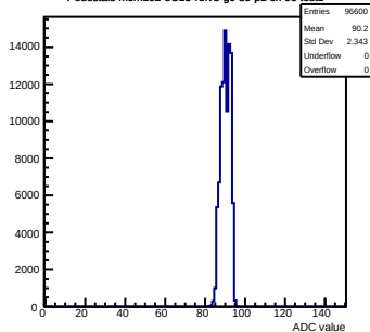
Pedestals mcm102-5C13-refV5-g0-s0-p1 ch 98 test1
