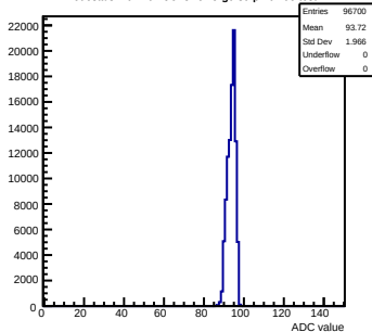
Pedestals mcm102-5C13-refV5-g0-s0-p1 ch 95 test1
