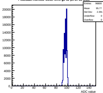
Pedestals mcm102-5C13-refV5-g0-s0-p1 ch 65 test1
