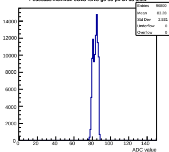
Pedestals mcm102-5C13-refV5-g0-s0-p1 ch 68 test1
