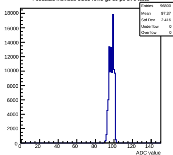
Pedestals mcm102-5C13-reV5-g0-s0-p1 ch 9 test1
