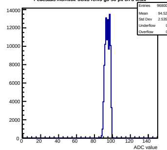
Pedestals mcm102-5C13-reV5-g0-s0-p1 ch 3 test1
