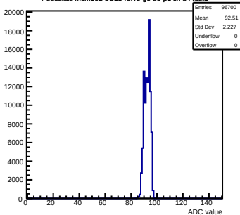
Pedestals mcm102-5C13-refV5-g0-s0-p1 ch 84 test1
