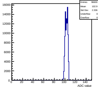
Pedestals mcm102-5C13-refV5-g0-s0-p1 ch 102 test1
