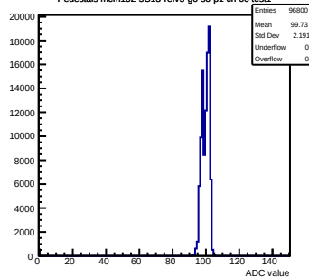
Pedestals mcm102-5C13-refV5-g0-s0-p1 ch 66 test1
