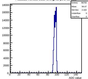
Pedestals mcm102-5C13-refV5-g0-s0-p1 ch 85 test1
