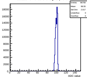
Pedestals mcm102-5C13-refV5-g0-s0-p1 ch 91 test1
