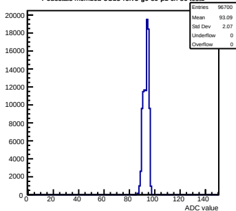
Pedestals mcm102-5C13-refV5-g0-s0-p1 ch 86 test1
