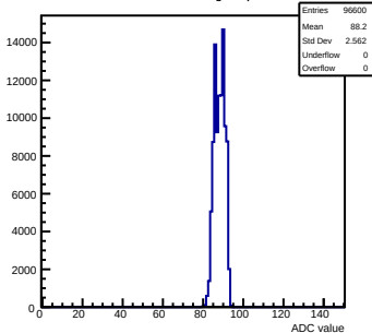
Pedestals mcm102-5C13-refV5-g0-s0-p1 ch 104 test1
