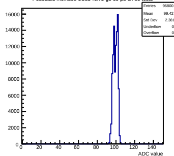
Pedestals mcm102-5C13-reV5-g0-s0-p1 ch 10 test1
