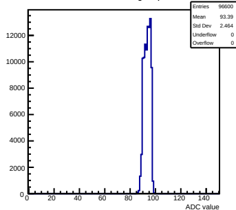
Pedestals mcm102-5C13-refV5-g0-s0-p1 ch 105 test1
