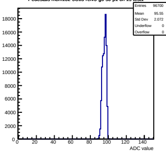
Pedestals mcm102-5C13-refV5-g0-s0-p1 ch 19 test1
