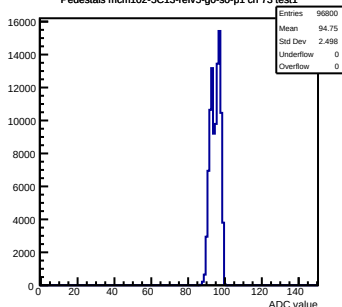
Pedestals mcm102-5C13-refV5-g0-s0-p1 ch 73 test1
