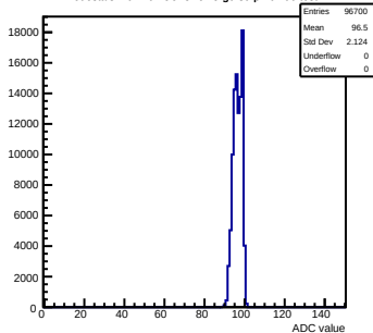
Pedestals mcm102-5C13-refV5-g0-s0-p1 ch 90 test1
