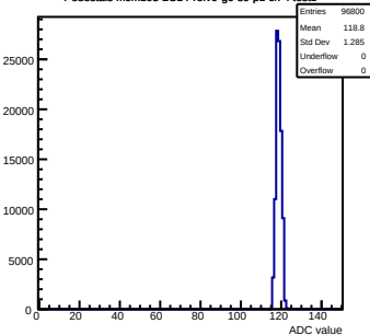
Pedestals mcm103-2C14-reV0-g0-s0-p1 ch 4 test1
