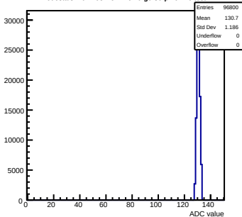
Pedestals mcm103-2C14-refV0-g0-s0-p1 ch 76 test1
