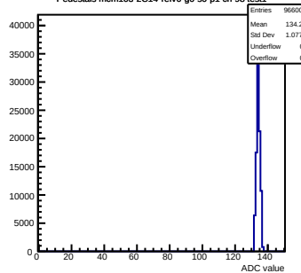
Pedestals mcm103-2C14-refV0-g0-s0-p1 ch 98 test1
