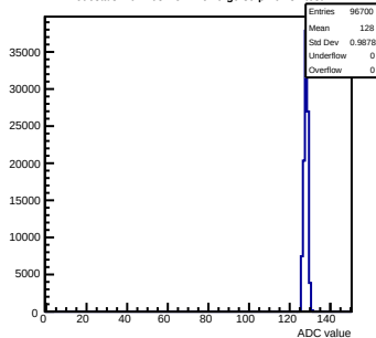
Pedestals mcm103-2C14-refV0-g0-s0-p1 ch 31 test1
