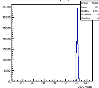
Pedestals mcm103-2C14-refV0-g0-s0-p1 ch 78 test1
