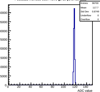
Pedestals mcm103-2C14-refV0-g0-s0-p1 ch 21 test1
