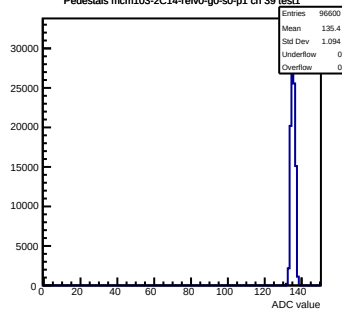
Pedestals mcm103-2C14-refV0-g0-s0-p1 ch 39 test1
