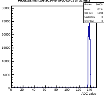
Pedestals mcm103-2C14-refV0-g0-s0-p1 ch 32 test1
