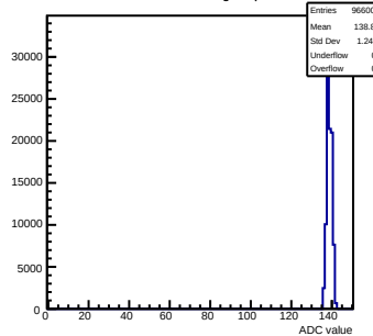
Pedestals mcm103-2C14-refV0-g0-s0-p1 ch 106 test1
