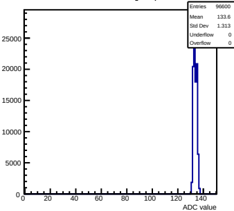
Pedestals mcm103-2C14-refV0-g0-s0-p1 ch 104 test1
