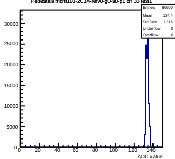
Pedestals mcm103-2C14-refV0-g0-s0-p1 ch 33 test1
