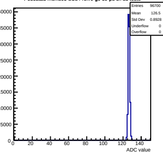
Pedestals mcm103-2C14-refV0-g0-s0-p1 ch 25 test1
