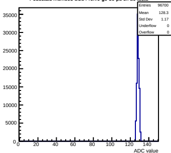
Pedestals mcm103-2C14-refV0-g0-s0-p1 ch 20 test1
