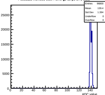
Pedestals mcm103-2C14-reV0-g0-s0-p1 ch 8 test1
