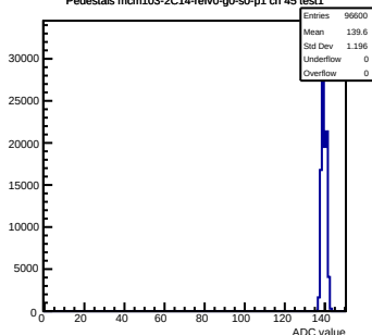
Pedestals mcm103-2C14-refV0-g0-s0-p1 ch 45 test1
