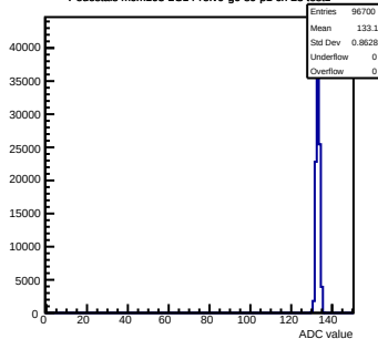
Pedestals mcm103-2C14-refV0-g0-s0-p1 ch 23 test1
