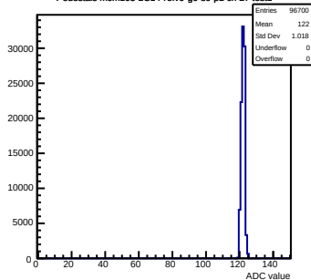
Pedestals mcm103-2C14-refV0-g0-s0-p1 ch 27 test1
