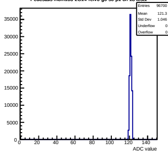
Pedestals mcm103-2C14-refV0-g0-s0-p1 ch 18 test1
