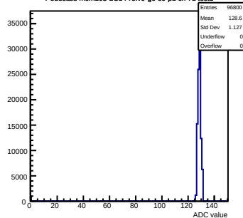
Pedestals mcm103-2C14-refV0-g0-s0-p1 ch 71 test1
