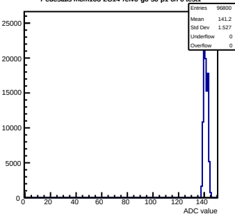
Pedestals mcm103-2C14-reV0-g0-s0-p1 ch 0 test1
