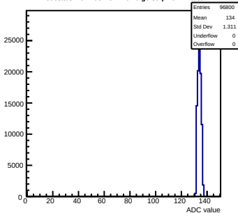
Pedestals mcm103-2C14-refV0-g0-s0-p1 ch 72 test1
