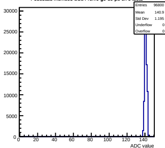
Pedestals mcm103-2C14-reV0-g0-s0-p1 ch 6 test1
