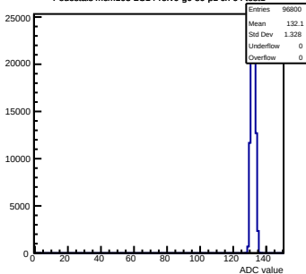
Pedestals mcm103-2C14-refV0-g0-s0-p1 ch 64 test1
