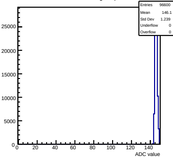
Pedestals mcm103-2C14-refV0-g0-s0-p1 ch 108 test1
