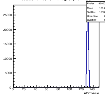
Pedestals mcm103-2C14-reV0-g0-s0-p1 ch 11 test1
