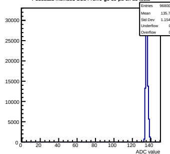
Pedestals mcm103-2C14-reV0-g0-s0-p1 ch 15 test1
