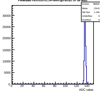
Pedestals mcm103-2C14-refV0-g0-s0-p1 ch 38 test1
