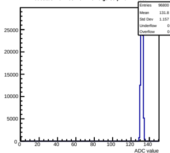
Pedestals mcm103-2C14-refV0-g0-s0-p1 ch 74 test1
