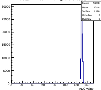
Pedestals mcm103-2C14-refV0-g0-s0-p1 ch 68 test1
