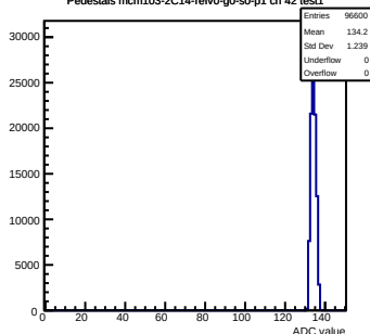
Pedestals mcm103-2C14-refV0-g0-s0-p1 ch 42 test1
