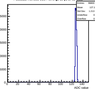
Pedestals mcm103-2C14-refV0-g0-s0-p1 ch 69 test1
