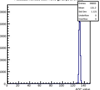
Pedestals mcm103-2C14-reV0-g0-s0-p1 ch 9 test1
