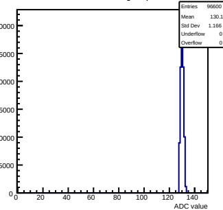
Pedestals mcm103-2C14-refV0-g0-s0-p1 ch 109 test1
