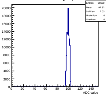
Pedestals mcm103-2C14-refv1-g0-s0-p1 ch 36 test1
