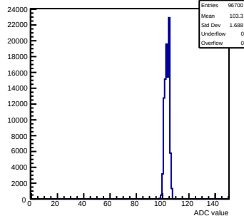
Pedestals mcm103-2C14-refv1-g0-s0-p1 ch 30 test1
