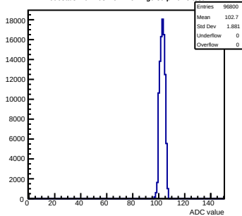
Pedestals mcm103-2C14-refV1-g0-s0-p1 ch 5 test1
