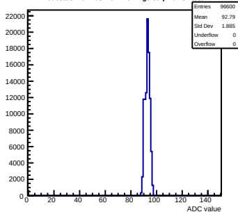
Pedestals mcm103-2C14-refv1-g0-s0-p1 ch 37 test1
