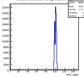
Pedestals mcm103-2C14-refV1-g0-s0-p1 ch 2 test1
