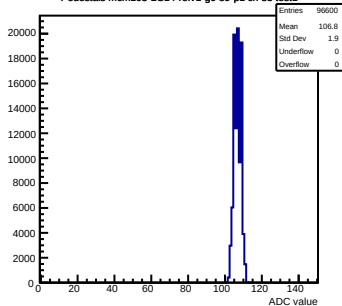
Pedestals mcm103-2C14-refv1-g0-s0-p1 ch 33 test1
