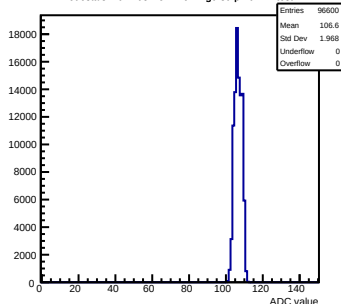
Pedestals mcm103-2C14-refv1-g0-s0-p1 ch 42 test1
