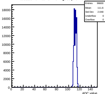
Pedestals mcm103-2C14-refv1-g0-s0-p1 ch 40 test1
