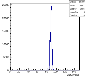
Pedestals mcm103-2C14-refv1-g0-s0-p1 ch 21 test1
