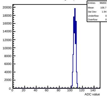
Pedestals mcm103-2C14-refV1-g0-s0-p1 ch 10 test1
