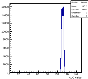
Pedestals mcm103-2C14-refV1-g0-s0-p1 ch 12 test1
