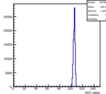
Pedestals mcm103-2C14-refv1-g0-s0-p1 ch 23 test1
