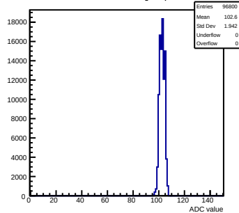
Pedestals mcm103-2C14-refV1-g0-s0-p1 ch 11 test1
