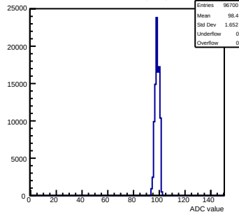
Pedestals mcm103-2C14-refv1-g0-s0-p1 ch 22 test1
