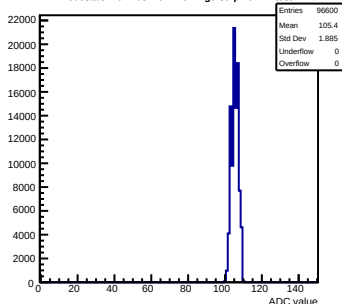
Pedestals mcm103-2C14-refv1-g0-s0-p1 ch 41 test1
