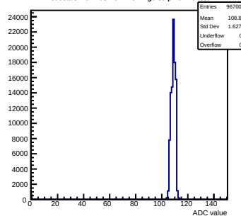
Pedestals mcm103-2C14-refv1-g0-s0-p1 ch 19 test1
