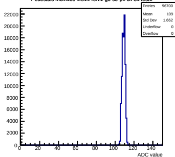
Pedestals mcm103-2C14-refv1-g0-s0-p1 ch 81 test1
