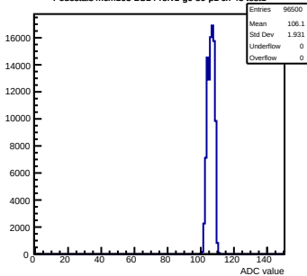
Pedestals mcm103-2C14-refV1-g0-s0-p1 ch 48 test1
