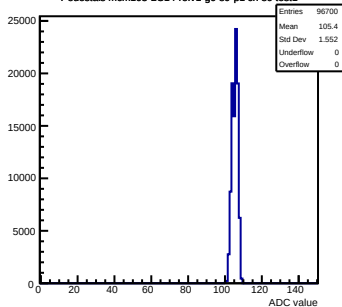
Pedestals mcm103-2C14-refv1-g0-s0-p1 ch 89 test1
