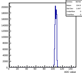
Pedestals mcm103-2C14-refv1-g0-s0-p1 ch 28 test1
