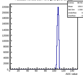
Pedestals mcm103-2C14-refv1-g0-s0-p1 ch 86 test1
