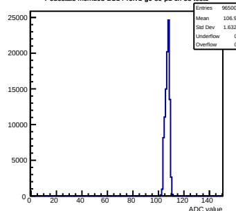
Pedestals mcm103-2C14-refV1-g0-s0-p1 ch 58 test1
