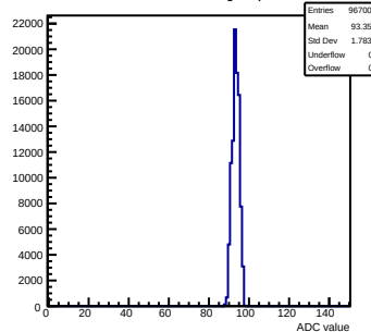
Pedestals mcm103-2C14-refv1-g0-s0-p1 ch 27 test1
