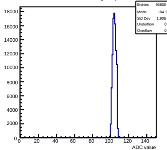
Pedestals mcm103-2C14-refV1-g0-s0-p1 ch 14 test1
