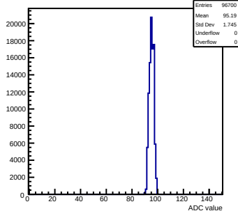
Pedestals mcm103-2C14-refv1-g0-s0-p1 ch 29 test1
