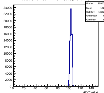
Pedestals mcm103-2C14-refV1-g0-s0-p1 ch 62 test1
