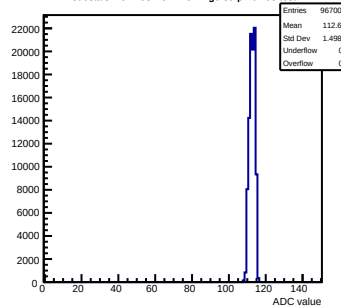
Pedestals mcm103-2C14-refv1-g0-s0-p1 ch 95 test1
