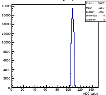
Pedestals mcm103-2C14-refv1-g0-s0-p1 ch 44 test1
