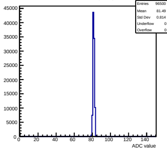
Pedestals mcm103-2C14-rev2-g0-s0-p1 ch 119 test1
