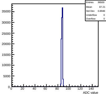
Pedestals mcm103-2C14-rev2-g0-s0-p1 ch 120 test1
