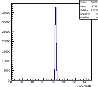
Pedestals mcm103-2C14-rev2-g0-s0-p1 ch 123 test1
