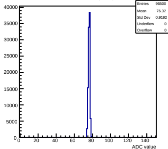
Pedestals mcm103-2C14-rev2-g0-s0-p1 ch 117 test1
