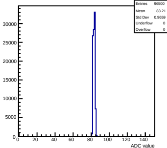
Pedestals mcm103-2C14-rev2-g0-s0-p1 ch 124 test1
