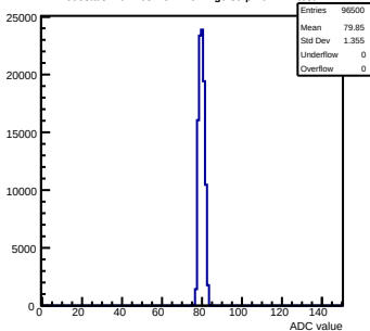
Pedestals mcm103-2C14-rev2-g0-s0-p1 ch 112 test1
