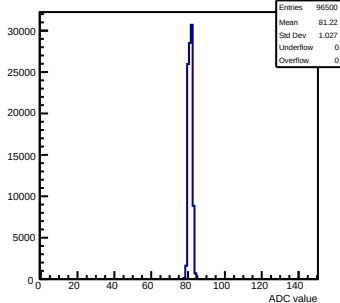
Pedestals mcm103-2C14-rev2-g0-s0-p1 ch 127 test1
