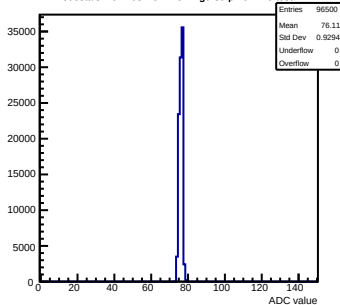
Pedestals mcm103-2C14-rev2-g0-s0-p1 ch 115 test1
