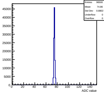
Pedestals mcm103-2C14-rev2-g0-s0-p1 ch 121 test1
