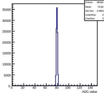
Pedestals mcm103-2C14-rev2-g0-s0-p1 ch 122 test1
