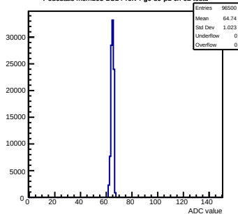
Pedestals mcm103-2C14-refV4-g0-s0-p1 ch 62 test1
