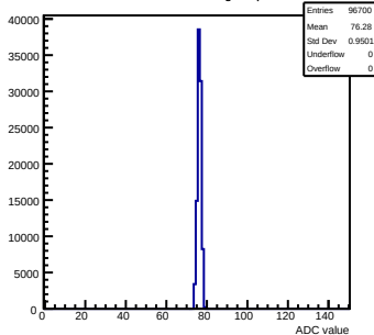
Pedestals mcm103-2C14-refV4-g0-s0-p1 ch 94 test1
