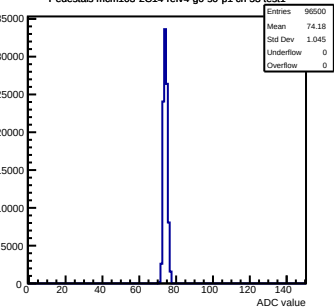
Pedestals mcm103-2C14-refV4-g0-s0-p1 ch 53 test1
