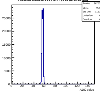
Pedestals mcm103-2C14-refv4-g0-s0-p1 ch 18 test1
