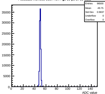
Pedestals mcm103-2C14-refV4-g0-s0-p1 ch 60 test1
