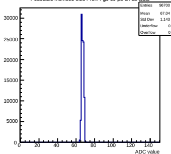
Pedestals mcm103-2C14-refV4-g0-s0-p1 ch 82 test1
