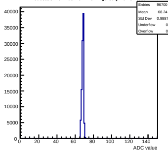
Pedestals mcm103-2C14-refV4-g0-s0-p1 ch 87 test1
