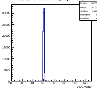
Pedestals mcm103-2C14-refv4-g0-s0-p1 ch 29 test1
