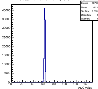
Pedestals mcm103-2C14-refv4-g0-s0-p1 ch 22 test1
