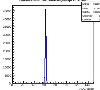
Pedestals mcm103-2C14-refV4-g0-s0-p1 ch 51 test1
