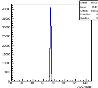
Pedestals mcm103-2C14-refV4-g0-s0-p1 ch 93 test1
