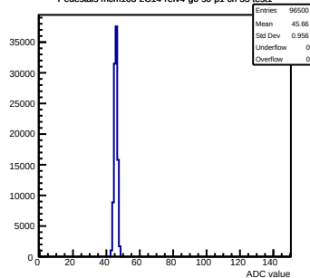
Pedestals mcm103-2C14-refV4-g0-s0-p1 ch 55 test1
