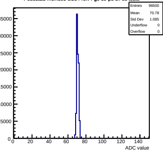
Pedestals mcm103-2C14-refV4-g0-s0-p1 ch 61 test1
