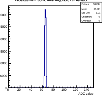
Pedestals mcm103-2C14-refV4-g0-s0-p1 ch 49 test1
