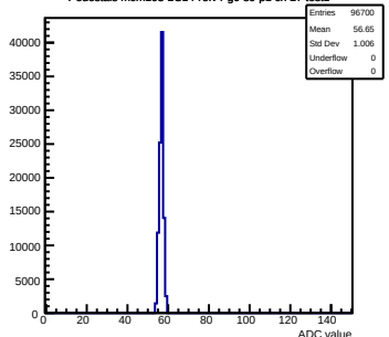
Pedestals mcm103-2C14-refv4-g0-s0-p1 ch 27 test1
