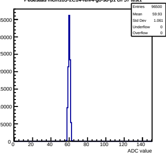
Pedestals mcm103-2C14-refV4-g0-s0-p1 ch 57 test1
