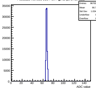
Pedestals mcm103-2C14-refv4-g0-s0-p1 ch 30 test1
