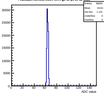
Pedestals mcm103-2C14-refV4-g0-s0-p1 ch 52 test1
