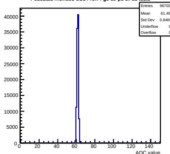
Pedestals mcm103-2C14-refv4-g0-s0-p1 ch 25 test1
