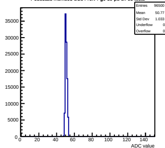
Pedestals mcm103-2C14-refV4-g0-s0-p1 ch 63 test1
