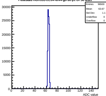
Pedestals mcm103-2C14-refV4-g0-s0-p1 ch 56 test1
