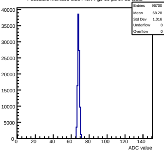
Pedestals mcm103-2C14-refv4-g0-s0-p1 ch 28 test1
