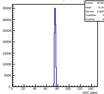
Pedestals mcm103-2C14-refV4-g0-s0-p1 ch 95 test1
