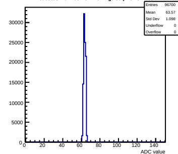
Pedestals mcm103-2C14-refV4-g0-s0-p1 ch 84 test1
