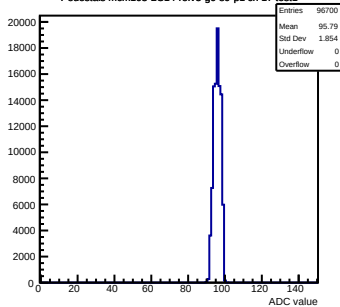
Pedestals mcm103-2C14-refV5-g0-s0-p1 ch 17 test1
