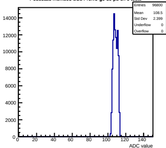
Pedestals mcm103-2C14-refV5-g0-s0-p1 ch 0 test1
