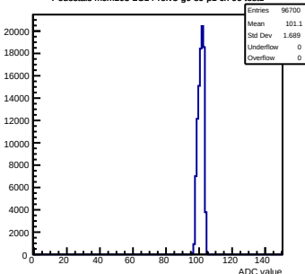
Pedestals mcm103-2C14-refV5-g0-s0-p1 ch 90 test1
