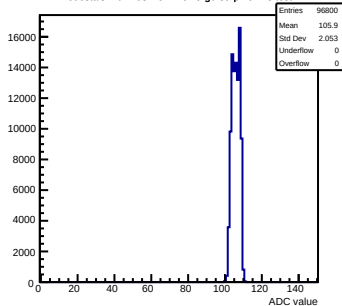
Pedestals mcm103-2C14-refV5-g0-s0-p1 ch 13 test1
