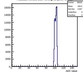
Pedestals mcm103-2C14-refV5-g0-s0-p1 ch 48 test1
