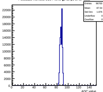
Pedestals mcm103-2C14-refV5-g0-s0-p1 ch 27 test1
