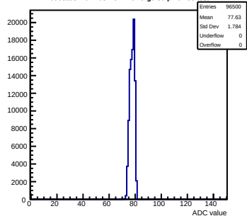
Pedestals mcm103-2C14-refV5-g0-s0-p1 ch 55 test1
