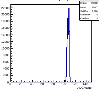
Pedestals mcm103-2C14-refV5-g0-s0-p1 ch 94 test1
