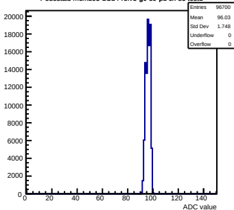
Pedestals mcm103-2C14-refV5-g0-s0-p1 ch 85 test1
