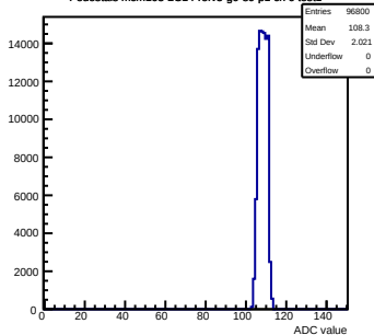
Pedestals mcm103-2C14-refV5-g0-s0-p1 ch 6 test1
