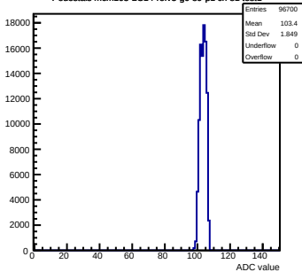
Pedestals mcm103-2C14-refV5-g0-s0-p1 ch 81 test1
