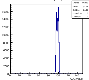
Pedestals mcm103-2C14-refV5-g0-s0-p1 ch 9 test1
