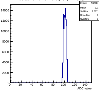
Pedestals mcm103-2C14-refV5-g0-s0-p1 ch 16 test1
