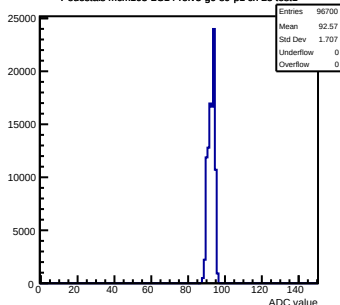
Pedestals mcm103-2C14-refV5-g0-s0-p1 ch 25 test1
