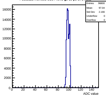
Pedestals mcm103-2C14-refV5-g0-s0-p1 ch 5 test1
