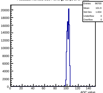
Pedestals mcm103-2C14-refV5-g0-s0-p1 ch 24 test1
