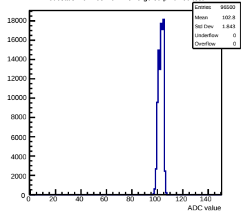
Pedestals mcm103-2C14-refV5-g0-s0-p1 ch 59 test1
