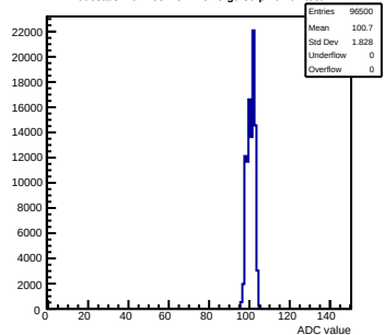
Pedestals mcm103-2C14-refV5-g0-s0-p1 ch 61 test1
