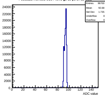
Pedestals mcm103-2C14-refV5-g0-s0-p1 ch 22 test1
