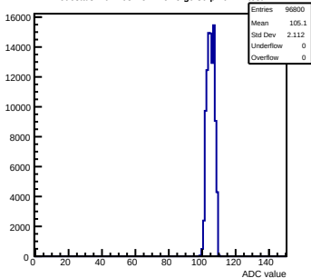
Pedestals mcm103-2C14-refV5-g0-s0-p1 ch 12 test1
