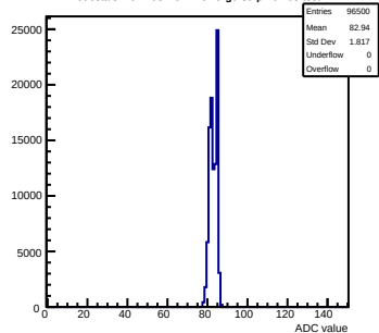
Pedestals mcm103-2C14-refV5-g0-s0-p1 ch 63 test1
