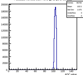
Pedestals mcm103-2C14-refV5-g0-s0-p1 ch 91 test1
