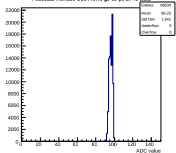
Pedestals mcm103-2C14-refV5-g0-s0-p1 ch 49 test1
