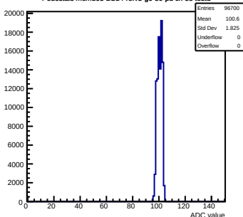
Pedestals mcm103-2C14-refV5-g0-s0-p1 ch 88 test1
