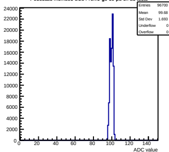
Pedestals mcm103-2C14-refV5-g0-s0-p1 ch 23 test1
