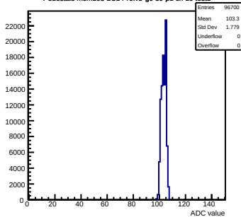
Pedestals mcm103-2C14-refV5-g0-s0-p1 ch 19 test1
