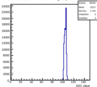
Pedestals mcm103-2C14-refV5-g0-s0-p1 ch 92 test1
