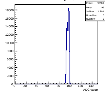
Pedestals mcm103-2C14-refV5-g0-s0-p1 ch 56 test1
