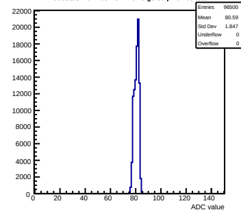
Pedestals mcm103-2C14-refV5-g0-s0-p1 ch 60 test1
