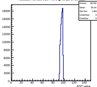
Pedestals mcm103-2C14-refV5-g0-s0-p1 ch 26 test1
