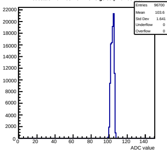
Pedestals mcm103-2C14-refV5-g0-s0-p1 ch 93 test1
