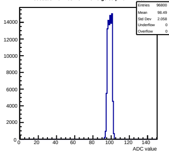
Pedestals mcm103-2C14-refV5-g0-s0-p1 ch 14 test1
