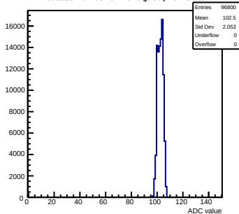
Pedestals mcm103-2C14-refV5-g0-s0-p1 ch 15 test1
