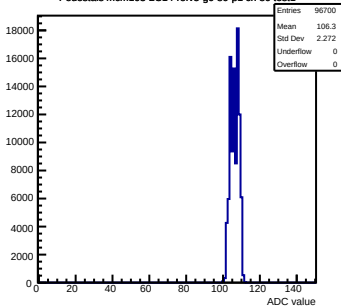
Pedestals mcm103-2C14-refV5-g0-s0-p1 ch 80 test1
