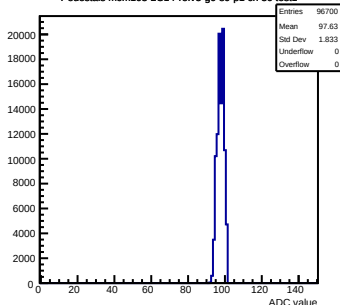
Pedestals mcm103-2C14-refV5-g0-s0-p1 ch 30 test1
