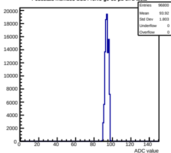
Pedestals mcm103-2C14-refV5-g0-s0-p1 ch 2 test1
