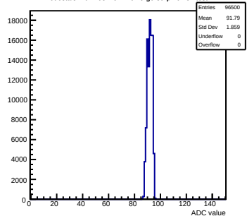
Pedestals mcm103-2C14-refV5-g0-s0-p1 ch 57 test1
