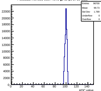
Pedestals mcm103-2C14-refV5-g0-s0-p1 ch 89 test1
