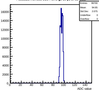
Pedestals mcm103-2C14-refV5-g0-s0-p1 ch 20 test1
