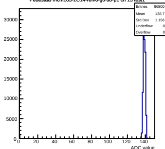
Pedestals mcm103-2C14-refV6-g0-s0-p1 ch 13 test1
