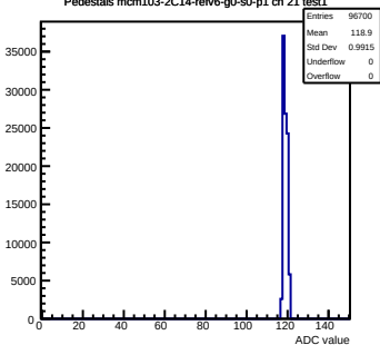
Pedestals mcm103-2C14-refV6-g0-s0-p1 ch 21 test1
