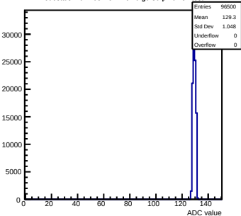
Pedestals mcm103-2C14-refV6-g0-s0-p1 ch 52 test1
