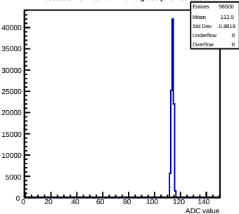
Pedestals mcm103-2C14-refV6-g0-s0-p1 ch 55 test1
