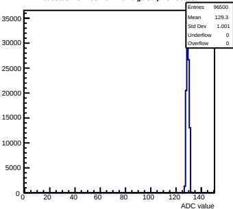
Pedestals mcm103-2C14-refV6-g0-s0-p1 ch 56 test1
