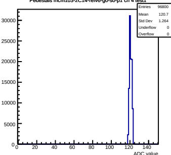
Pedestals mcm103-2C14-refV6-g0-s0-p1 ch 4 test1
