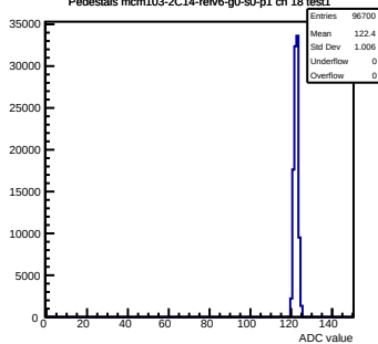
Pedestals mcm103-2C14-refV6-g0-s0-p1 ch 18 test1
