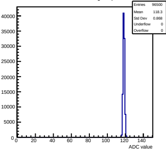
Pedestals mcm103-2C14-refV6-g0-s0-p1 ch 63 test1
