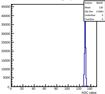
Pedestals mcm103-2C14-refV6-g0-s0-p1 ch 62 test1
