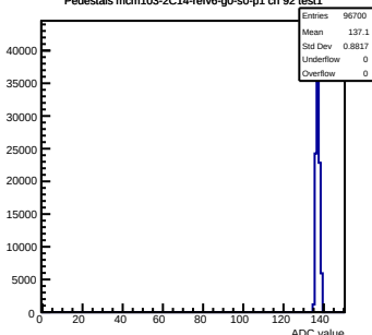
Pedestals mcm103-2C14-refV6-g0-s0-p1 ch 92 test1
