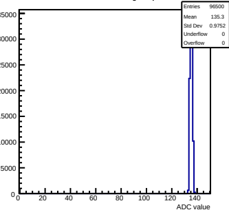
Pedestals mcm103-2C14-refV6-g0-s0-p1 ch 61 test1
