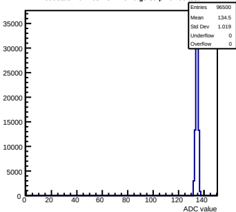
Pedestals mcm103-2C14-refV6-g0-s0-p1 ch 58 test1
