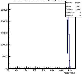
Pedestals mcm103-2C14-refV6-g0-s0-p1 ch 48 test1
