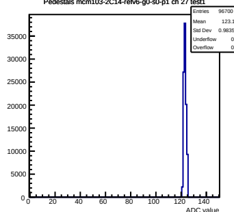
Pedestals mcm103-2C14-refV6-g0-s0-p1 ch 27 test1
