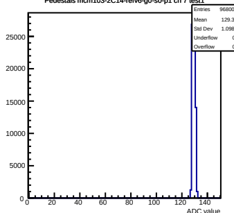
Pedestals mcm103-2C14-refV6-g0-s0-p1 ch 7 test1
