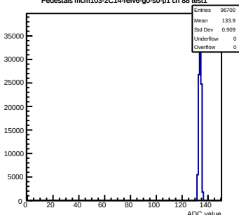
Pedestals mcm103-2C14-refV6-g0-s0-p1 ch 88 test1
