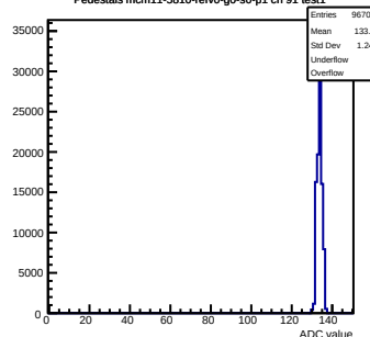
Pedestals mcm11-5810-refV0-g0-s0-p1 ch 91 test1
