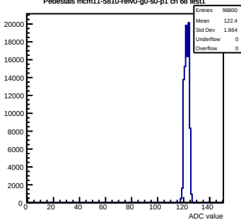
Pedestals mcm11-5810-refV0-g0-s0-p1 ch 68 test1
