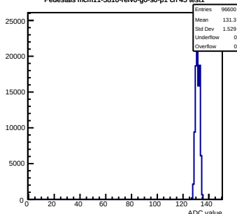
Pedestals mcm11-5810-refV0-g0-s0-p1 ch 45 test1
