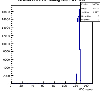
Pedestals mcm11-5810-refV0-g0-s0-p1 ch 72 test1
