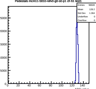
Pedestals mcm11-5810-refV0-g0-s0-p1 ch 61 test1
