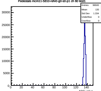
Pedestals mcm11-5810-refV0-g0-s0-p1 ch 60 test1
