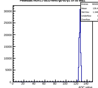
Pedestals mcm11-5810-refV0-g0-s0-p1 ch 55 test1
