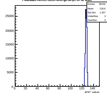
Pedestals mcm11-5810-refV0-g0-s0-p1 ch 92 test1
