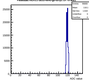
Pedestals mcm11-5810-refV0-g0-s0-p1 ch 79 test1
