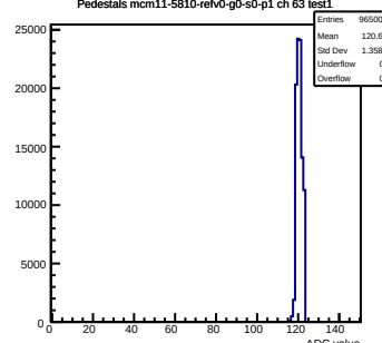
Pedestals mcm11-5810-refV0-g0-s0-p1 ch 63 test1
