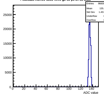
Pedestals mcm11-5810-refV0-g0-s0-p1 ch 98 test1
