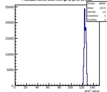
Pedestals mcm11-5810-refV0-g0-s0-p1 ch 36 test1
