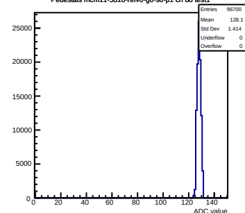
Pedestals mcm11-5810-refV0-g0-s0-p1 ch 88 test1
