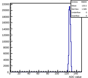
Pedestals mcm11-5810-refv0-g0-s0-p1 ch 5 test1
