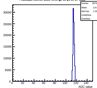
Pedestals mcm11-5810-refV0-g0-s0-p1 ch 87 test1
