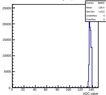
Pedestals mcm11-5810-refv0-g0-s0-p1 ch 9 test1
