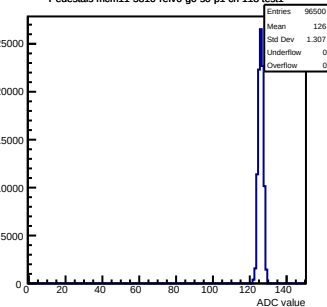
Pedestals mcm11-5810-refV0-g0-s0-p1 ch 118 test1
