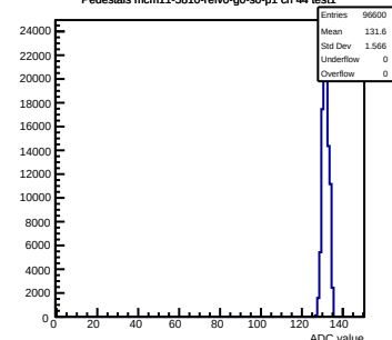
Pedestals mcm11-5810-refV0-g0-s0-p1 ch 44 test1
