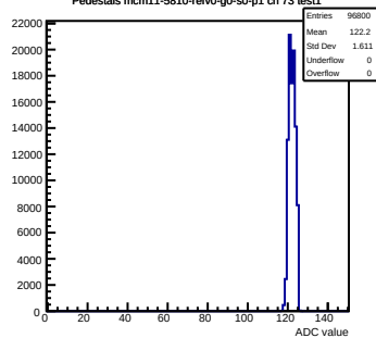
Pedestals mcm11-5810-refV0-g0-s0-p1 ch 73 test1
