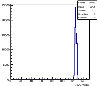
Pedestals mcm11-5810-refv0-g0-s0-p1 ch 8 test1
