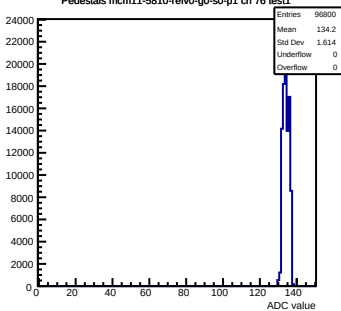
Pedestals mcm11-5810-refV0-g0-s0-p1 ch 76 test1
