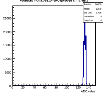
Pedestals mcm11-5810-refV0-g0-s0-p1 ch 71 test1
