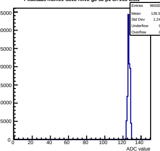
Pedestals mcm11-5810-refV0-g0-s0-p1 ch 115 test1
