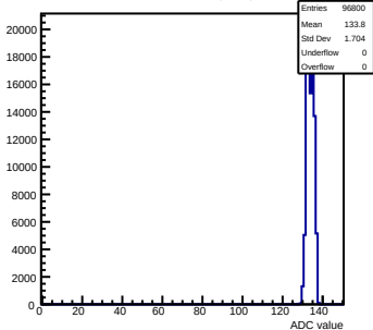
Pedestals mcm11-5810-refv0-g0-s0-p1 ch 4 test1
