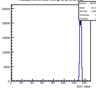
Pedestals mcm11-5810-refV0-g0-s0-p1 ch 82 test1
