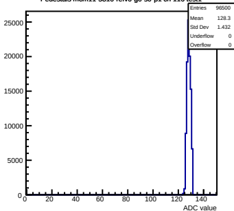
Pedestals mcm11-5810-refV0-g0-s0-p1 ch 116 test1
