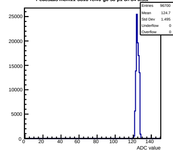
Pedestals mcm11-5810-refV0-g0-s0-p1 ch 84 test1
