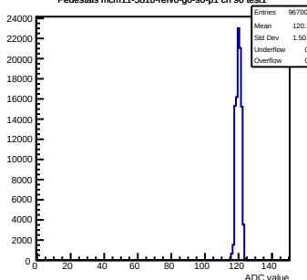
Pedestals mcm11-5810-refV0-g0-s0-p1 ch 90 test1
