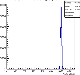
Pedestals mcm11-5810-refV0-g0-s0-p1 ch 126 test1
