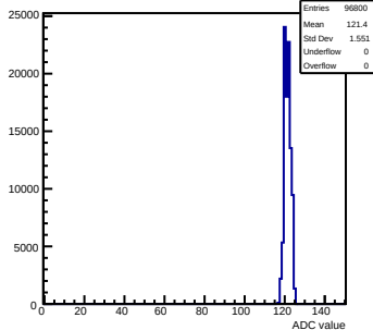
Pedestals mcm11-5810-refv0-g0-s0-p1 ch 13 test1
