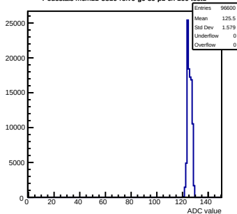
Pedestals mcm11-5810-refV0-g0-s0-p1 ch 109 test1
