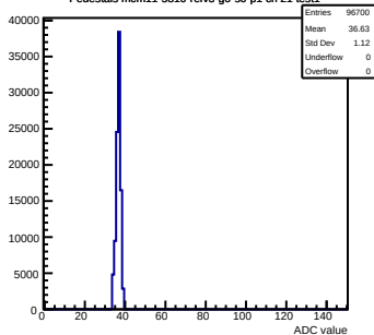
Pedestals mcm11-5810-refv3-g0-s0-p1 ch 17 test1
