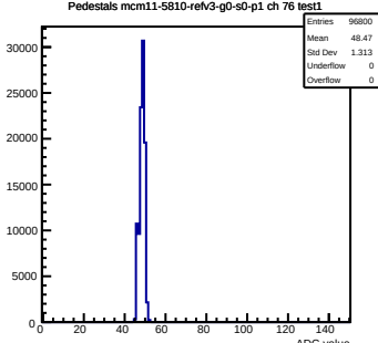
Pedestals mcm11-5810-refv3-g0-s0-p1 ch 76 test1
