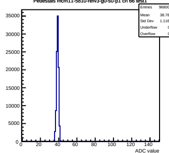
Pedestals mcm11-5810-refv3-g0-s0-p1 ch 66 test1
