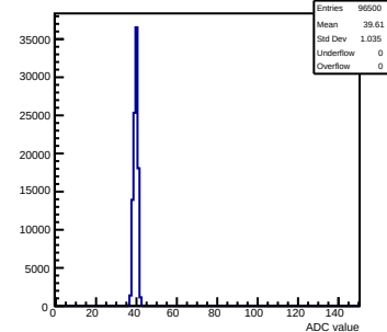
Pedestals mcm11-5810-refv3-g0-s0-p1 ch 120 test1
