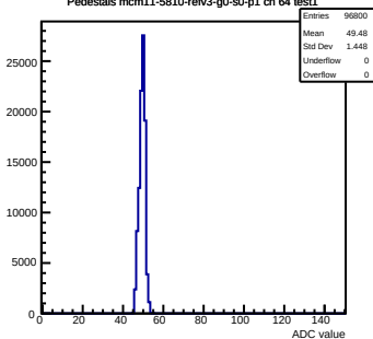
Pedestals mcm11-5810-refv3-g0-s0-p1 ch 64 test1
