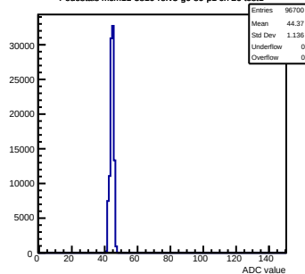
Pedestals mcm11-5810-refv3-g0-s0-p1 ch 26 test1
