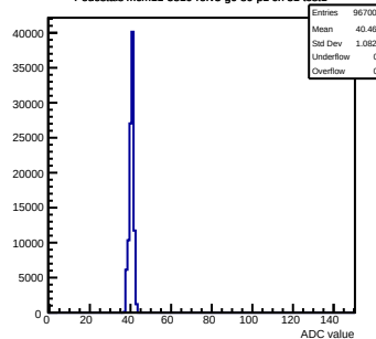
Pedestals mcm11-5810-refv3-g0-s0-p1 ch 27 test1
