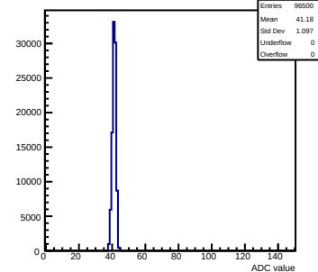
Pedestals mcm11-5810-refv3-g0-s0-p1 ch 112 test1
