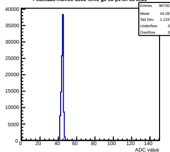
Pedestals mcm11-5810-refv3-g0-s0-p1 ch 18 test1
