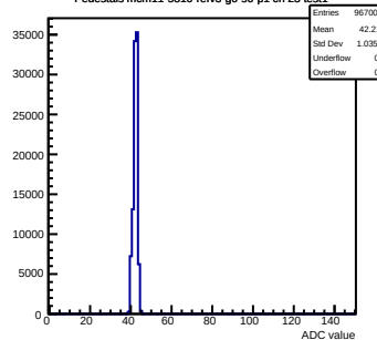
Pedestals mcm11-5810-refv3-g0-s0-p1 ch 19 test1
