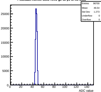
Pedestals mcm11-5810-refv3-g0-s0-p1 ch 16 test1
