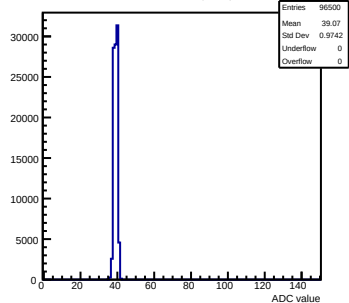
Pedestals mcm11-5810-refv3-g0-s0-p1 ch 115 test1
