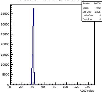
Pedestals mcm11-5810-refv3-g0-s0-p1 ch 28 test1
