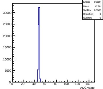
Pedestals mcm11-5810-refv3-g0-s0-p1 ch 119 test1
