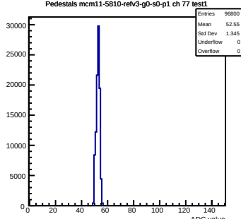
Pedestals mcm11-5810-refv3-g0-s0-p1 ch 77 test1
