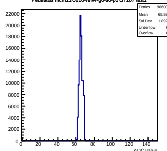
Pedestals mcm11-5810-refv4-g0-s0-p1 ch 107 test1
