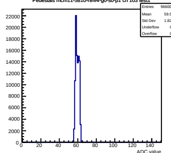
Pedestals mcm11-5810-refv4-g0-s0-p1 ch 103 test1
