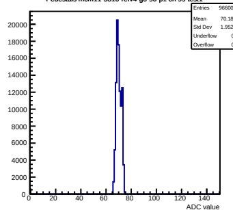
Pedestals mcm11-5810-refv4-g0-s0-p1 ch 99 test1
