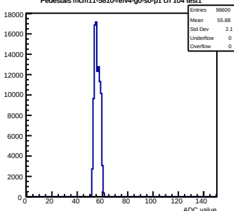
Pedestals mcm11-5810-refv4-g0-s0-p1 ch 104 test1
