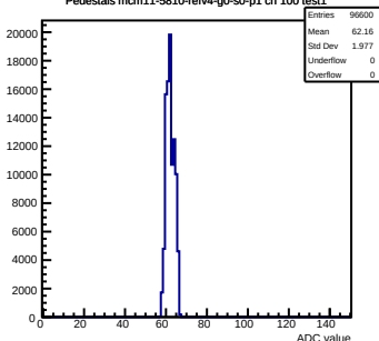
Pedestals mcm11-5810-refv4-g0-s0-p1 ch 100 test1
