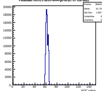
Pedestals mcm11-5810-refv4-g0-s0-p1 ch 106 test1
