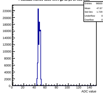
Pedestals mcm11-5810-refv4-g0-s0-p1 ch 113 test1
