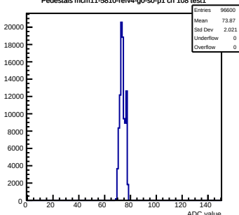
Pedestals mcm11-5810-refv4-g0-s0-p1 ch 108 test1
