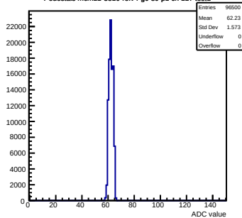
Pedestals mcm11-5810-refv4-g0-s0-p1 ch 117 test1
