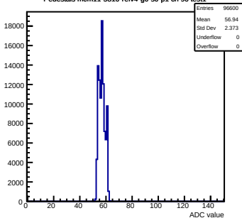
Pedestals mcm11-5810-refv4-g0-s0-p1 ch 96 test1
