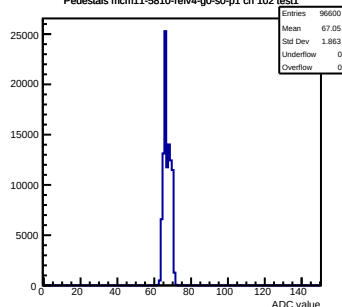
Pedestals mcm11-5810-refv4-g0-s0-p1 ch 102 test1
