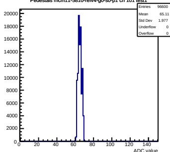
Pedestals mcm11-5810-refv4-g0-s0-p1 ch 101 test1
