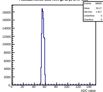
Pedestals mcm11-5810-refv4-g0-s0-p1 ch 97 test1
