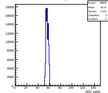
Pedestals mcm11-5810-refv4-g0-s0-p1 ch 8 test1
