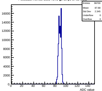
Pedestals mcm11-5810-refV5-g0-s0-p1 ch 80 test1
