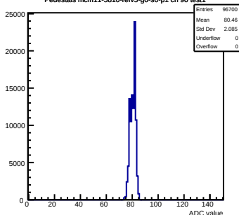
Pedestals mcm11-5810-refV5-g0-s0-p1 ch 90 test1
