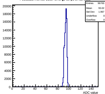
Pedestals mcm11-5810-refV5-g0-s0-p1 ch 83 test1
