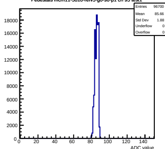
Pedestals mcm11-5810-refV5-g0-s0-p1 ch 95 test1
