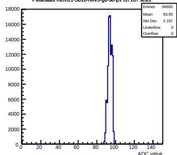
Pedestals mcm11-5810-refV5-g0-s0-p1 ch 107 test1
