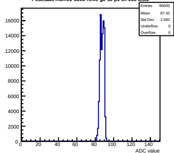
Pedestals mcm11-5810-refV5-g0-s0-p1 ch 103 test1
