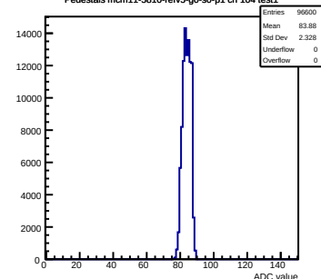
Pedestals mcm11-5810-refV5-g0-s0-p1 ch 104 test1
