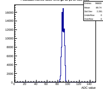
Pedestals mcm11-5810-refV5-g0-s0-p1 ch 96 test1
