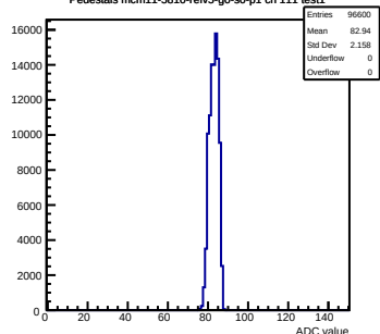
Pedestals mcm11-5810-refV5-g0-s0-p1 ch 111 test1
