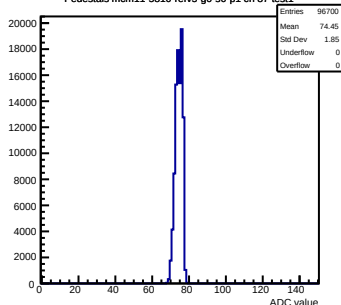
Pedestals mcm11-5810-refV5-g0-s0-p1 ch 87 test1
