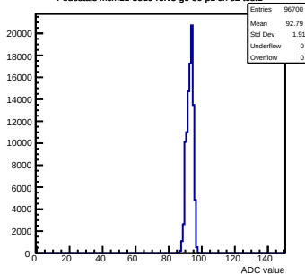
Pedestals mcm11-5810-refV5-g0-s0-p1 ch 82 test1
