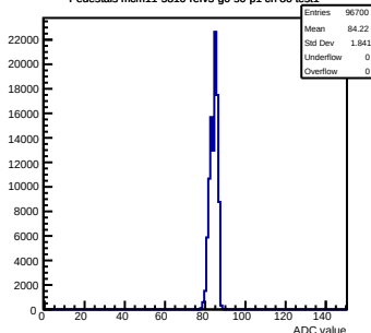
Pedestals mcm11-5810-refV5-g0-s0-p1 ch 86 test1
