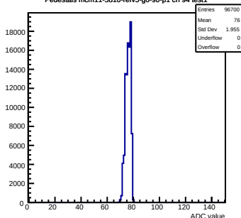
Pedestals mcm11-5810-refV5-g0-s0-p1 ch 94 test1
