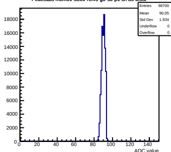
Pedestals mcm11-5810-refV5-g0-s0-p1 ch 85 test1
