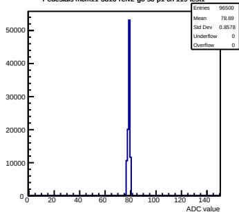
Pedestals mcm11-5810-ref2-g0-s0-p1 ch 119 test1
