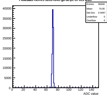
Pedestals mcm11-5810-ref2-g0-s0-p1 ch 123 test1
