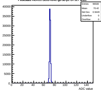
Pedestals mcm11-5810-ref2-g0-s0-p1 ch 127 test1
