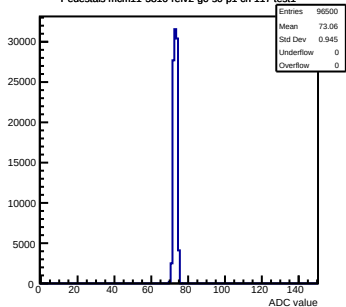
Pedestals mcm11-5810-ref2-g0-s0-p1 ch 117 test1
