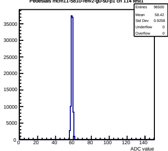
Pedestals mcm11-5810-ref2-g0-s0-p1 ch 114 test1
