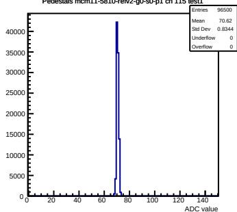
Pedestals mcm11-5810-ref2-g0-s0-p1 ch 115 test1
