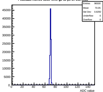
Pedestals mcm11-5810-ref2-g0-s0-p1 ch 118 test1
