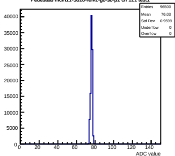
Pedestals mcm11-5810-ref2-g0-s0-p1 ch 121 test1
