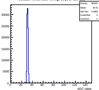
Pedestals mcm11-5810-refv3-g0-s0-p1 ch 126 test1
