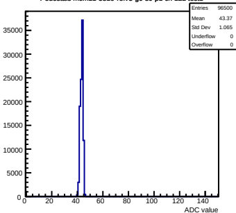
Pedestals mcm11-5810-refv3-g0-s0-p1 ch 122 test1
