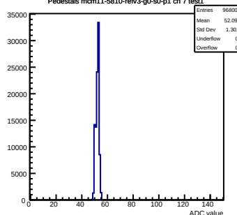
Pedestals mcm11-5810-refv3-g0-s0-p1 ch 7 test1
