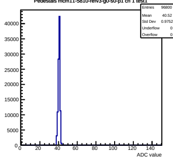
Pedestals mcm11-5810-refv3-g0-s0-p1 ch 1 test1
