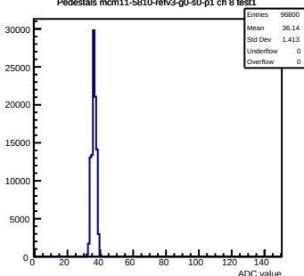
Pedestals mcm11-5810-refv3-g0-s0-p1 ch 8 test1
