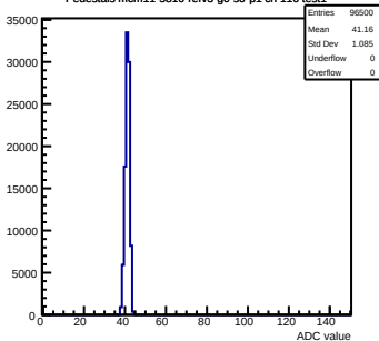
Pedestals mcm11-5810-refv3-g0-s0-p1 ch 116 test1
