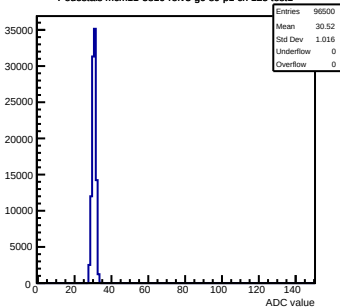
Pedestals mcm11-5810-refv3-g0-s0-p1 ch 125 test1
