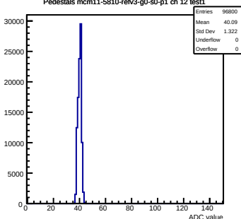
Pedestals mcm11-5810-refv3-g0-s0-p1 ch 12 test1
