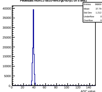
Pedestals mcm11-5810-refv3-g0-s0-p1 ch 5 test1
