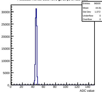
Pedestals mcm11-5810-refv3-g0-s0-p1 ch 121 test1
