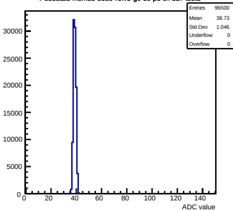
Pedestals mcm11-5810-refv3-g0-s0-p1 ch 127 test1
