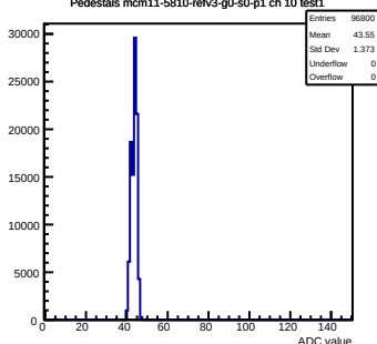
Pedestals mcm11-5810-refv3-g0-s0-p1 ch 10 test1
