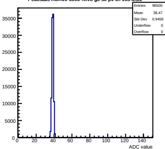
Pedestals mcm11-5810-refv3-g0-s0-p1 ch 118 test1
