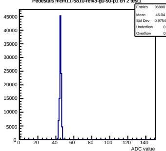
Pedestals mcm11-5810-refv3-g0-s0-p1 ch 2 test1
