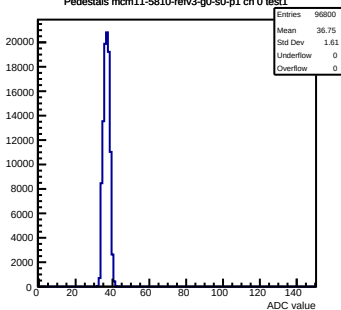
Pedestals mcm11-5810-refv3-g0-s0-p1 ch 0 test1
