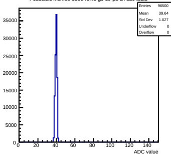
Pedestals mcm11-5810-refv3-g0-s0-p1 ch 120 test1
