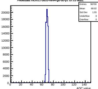
Pedestals mcm11-5810-refv4-g0-s0-p1 ch 25 test1
