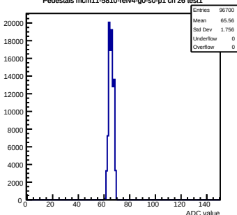
Pedestals mcm11-5810-refv4-g0-s0-p1 ch 26 test1
