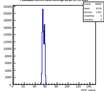
Pedestals mcm11-5810-refv4-g0-s0-p1 ch 15 test1
