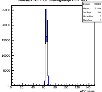
Pedestals mcm11-5810-refv4-g0-s0-p1 ch 22 test1
