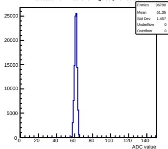
Pedestals mcm11-5810-refv4-g0-s0-p1 ch 93 test1
