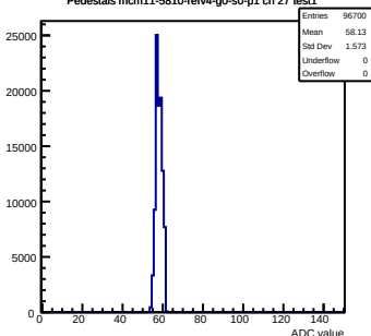
Pedestals mcm11-5810-refv4-g0-s0-p1 ch 27 test1
