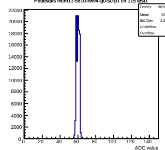
Pedestals mcm11-5810-refv4-g0-s0-p1 ch 115 test1
