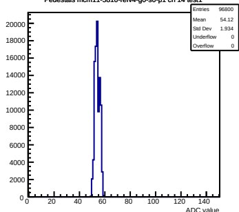
Pedestals mcm11-5810-refv4-g0-s0-p1 ch 14 test1
