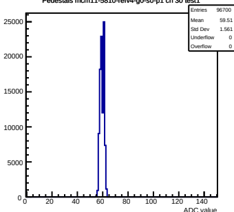
Pedestals mcm11-5810-refv4-g0-s0-p1 ch 30 test1
