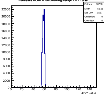
Pedestals mcm11-5810-refv4-g0-s0-p1 ch 21 test1
