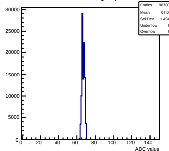
Pedestals mcm11-5810-refv4-g0-s0-p1 ch 91 test1
