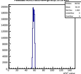
Pedestals mcm11-5810-refv4-g0-s0-p1 ch 29 test1
