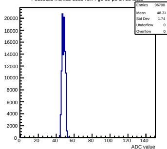
Pedestals mcm11-5810-refv4-g0-s0-p1 ch 81 test1
