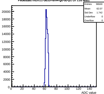
Pedestals mcm11-5810-refv4-g0-s0-p1 ch 116 test1
