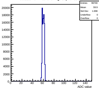
Pedestals mcm11-5810-refv4-g0-s0-p1 ch 88 test1
