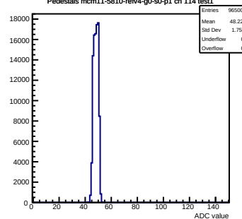
Pedestals mcm11-5810-refv4-g0-s0-p1 ch 114 test1
