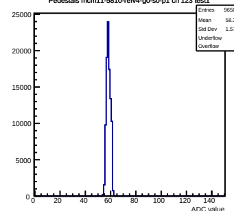
Pedestals mcm11-5810-refv4-g0-s0-p1 ch 123 test1
