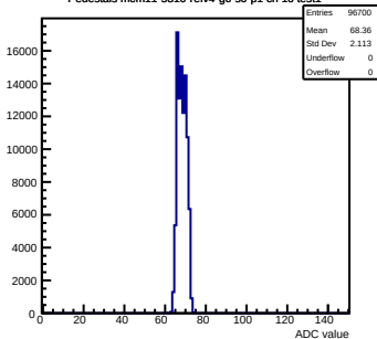
Pedestals mcm11-5810-refv4-g0-s0-p1 ch 16 test1
