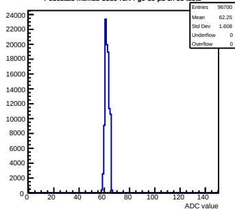
Pedestals mcm11-5810-refv4-g0-s0-p1 ch 85 test1
