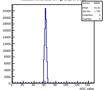
Pedestals mcm11-5810-refv4-g0-s0-p1 ch 1 test1
