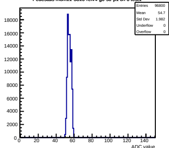
Pedestals mcm11-5810-refv4-g0-s0-p1 ch 6 test1
