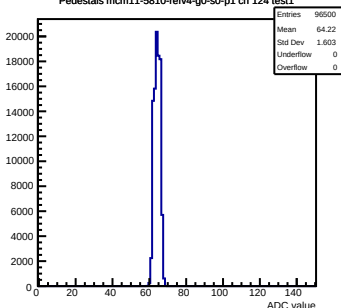
Pedestals mcm11-5810-refv4-g0-s0-p1 ch 124 test1
