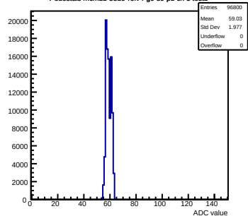
Pedestals mcm11-5810-refv4-g0-s0-p1 ch 3 test1
