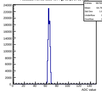
Pedestals mcm11-5810-refv4-g0-s0-p1 ch 83 test1
