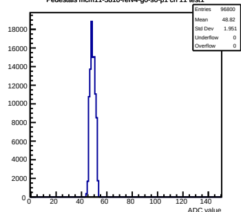
Pedestals mcm11-5810-refv4-g0-s0-p1 ch 11 test1
