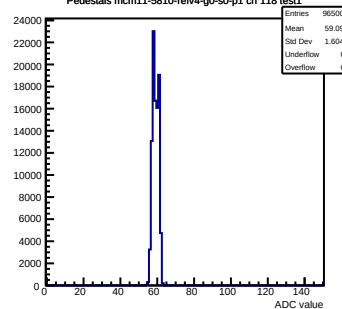
Pedestals mcm11-5810-refv4-g0-s0-p1 ch 118 test1
