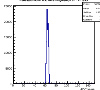
Pedestals mcm11-5810-refv4-g0-s0-p1 ch 122 test1
