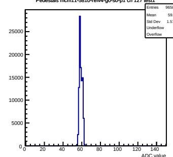
Pedestals mcm11-5810-refv4-g0-s0-p1 ch 127 test1
