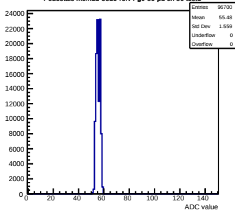
Pedestals mcm11-5810-refv4-g0-s0-p1 ch 86 test1
