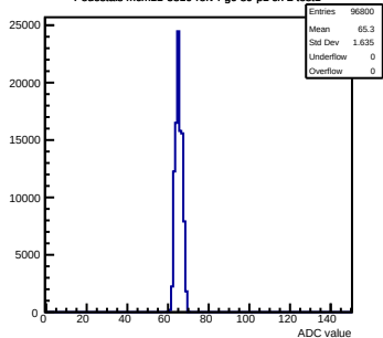
Pedestals mcm11-5810-refv4-g0-s0-p1 ch 2 test1
