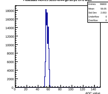
Pedestals mcm11-5810-refv4-g0-s0-p1 ch 8 test1
