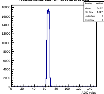
Pedestals mcm11-5810-refv4-g0-s0-p1 ch 18 test1
