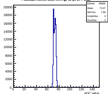
Pedestals mcm11-5810-refv4-g0-s0-p1 ch 7 test1
