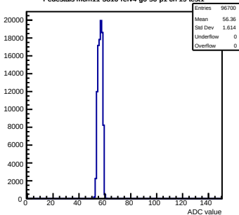
Pedestals mcm11-5810-refv4-g0-s0-p1 ch 19 test1
