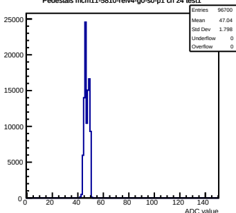
Pedestals mcm11-5810-refv4-g0-s0-p1 ch 24 test1
