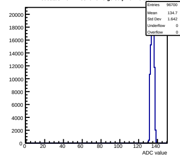
Pedestals mcm11-5810-refv6-g0-s0-p1 ch 16 test1
