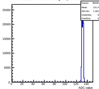
Pedestals mcm11-5810- refV6-g0-s0-p1 ch 58 test1
