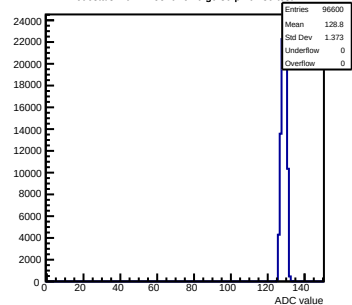
Pedestals mcm11-5810-refv6-g0-s0-p1 ch 39 test1
