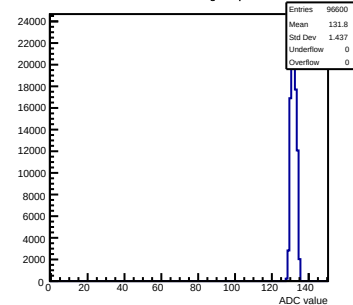
Pedestals mcm11-5810-refv6-g0-s0-p1 ch 44 test1
