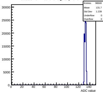
Pedestals mcm11-5810- refV6-g0-s0-p1 ch 57 test1
