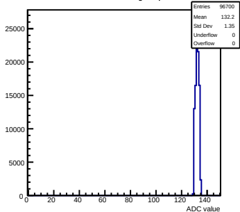
Pedestals mcm11-5810-refv6-g0-s0-p1 ch 26 test1
