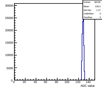
Pedestals mcm11-5810-refv6-g0-s0-p1 ch 28 test1
