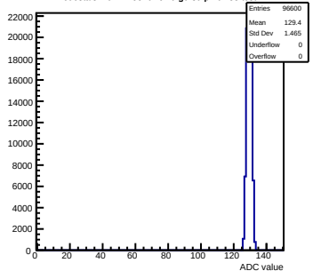
Pedestals mcm11-5810-refv6-g0-s0-p1 ch 33 test1
