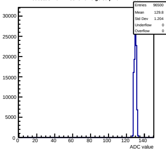
Pedestals mcm11-5810-refv6-g0-s0-p1 ch 122 test1
