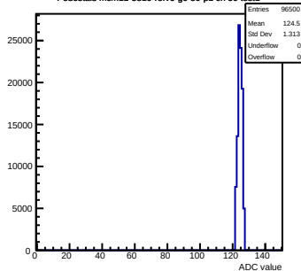
Pedestals mcm11-5810- refV6-g0-s0-p1 ch 50 test1
