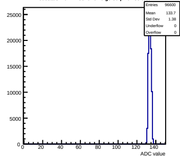
Pedestals mcm11-5810-refv6-g0-s0-p1 ch 35 test1
