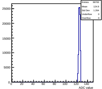
Pedestals mcm11-5810-refv6-g0-s0-p1 ch 21 test1
