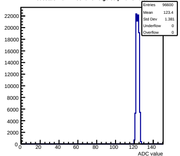
Pedestals mcm11-5810-refv6-g0-s0-p1 ch 37 test1
