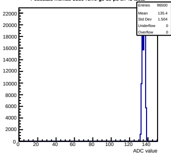
Pedestals mcm11-5810- refV6-g0-s0-p1 ch 48 test1
