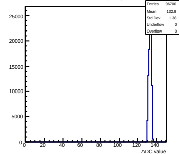
Pedestals mcm11-5810-refv6-g0-s0-p1 ch 20 test1
