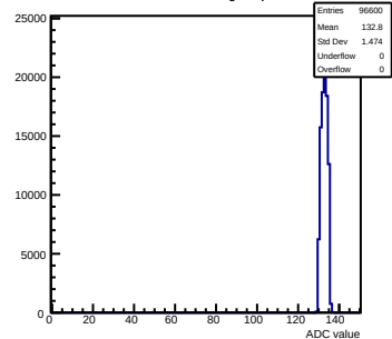
Pedestals mcm11-5810-refv6-g0-s0-p1 ch 43 test1
