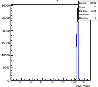
Pedestals mcm11-5810- refV6-g0-s0-p1 ch 56 test1
