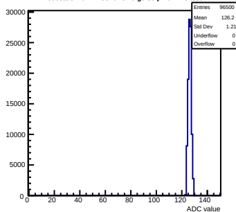
Pedestals mcm11-5810-refv6-g0-s0-p1 ch 123 test1
