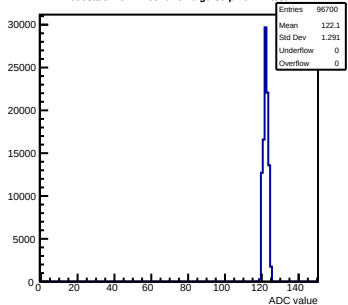
Pedestals mcm11-5810-refv6-g0-s0-p1 ch 17 test1
