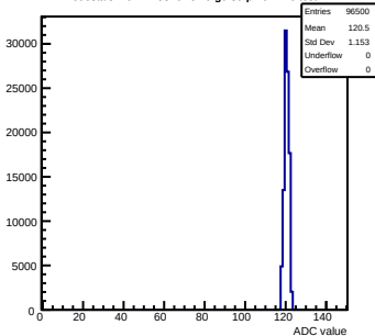
Pedestals mcm11-5810-refv6-g0-s0-p1 ch 126 test1
