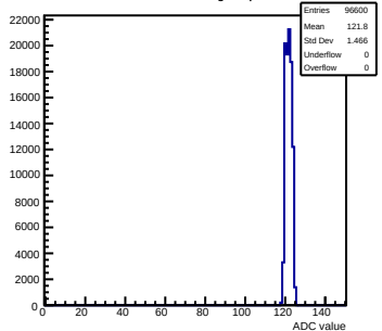
Pedestals mcm11-5810-refv6-g0-s0-p1 ch 41 test1
