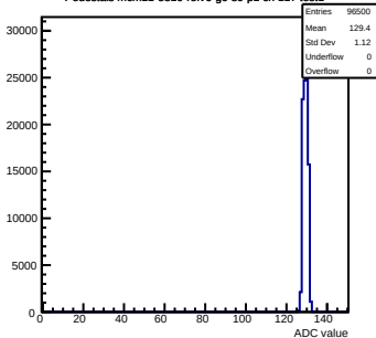
Pedestals mcm11-5810-refv6-g0-s0-p1 ch 117 test1
