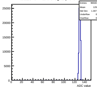
Pedestals mcm11-5810- refV6-g0-s0-p1 ch 62 test1
