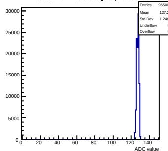
Pedestals mcm11-5810- refV6-g0-s0-p1 ch 59 test1
