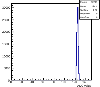
Pedestals mcm11-5810-refv6-g0-s0-p1 ch 29 test1
