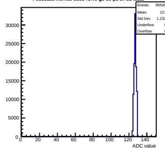
Pedestals mcm11-5810- refV6-g0-s0-p1 ch 55 test1
