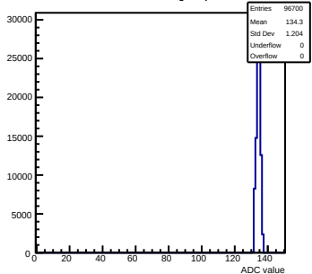
Pedestals mcm11-5810-refv6-g0-s0-p1 ch 25 test1
