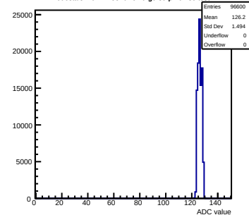
Pedestals mcm11-5810-refv6-g0-s0-p1 ch 36 test1
