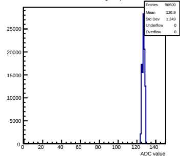
Pedestals mcm11-5810-refv6-g0-s0-p1 ch 47 test1
