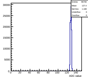
Pedestals mcm11-5810-refv6-g0-s0-p1 ch 31 test1
