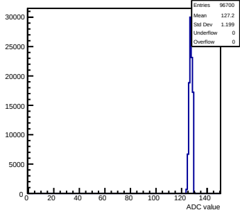
Pedestals mcm11-5810-refv6-g0-s0-p1 ch 30 test1
