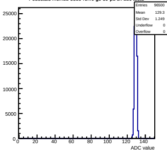
Pedestals mcm11-5810-refv6-g0-s0-p1 ch 116 test1
