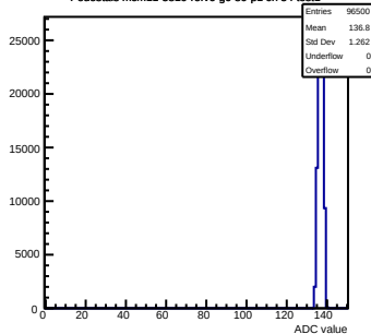
Pedestals mcm11-5810- refV6-g0-s0-p1 ch 54 test1
