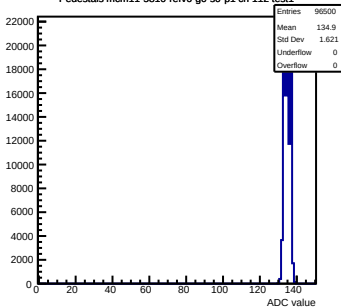
Pedestals mcm11-5810-refv6-g0-s0-p1 ch 112 test1
