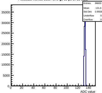
Pedestals mcm11-5810-refV0-g0-s0-p1 ch 33 test1
