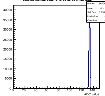
Pedestals mcm11-5810-refV0-g0-s0-p1 ch 18 test1
