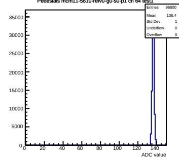
Pedestals mcm11-5810-refV0-g0-s0-p1 ch 64 test1
