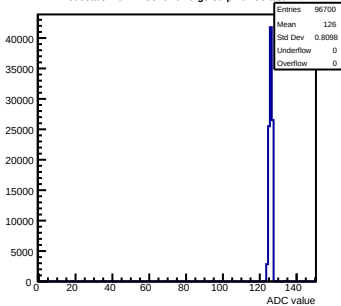
Pedestals mcm11-5810-refV0-g0-s0-p1 ch 86 test1
