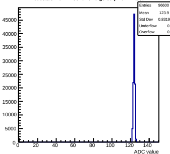
Pedestals mcm11-5810-refV0-g0-s0-p1 ch 41 test1
