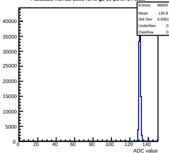
Pedestals mcm11-5810-refV0-g0-s0-p1 ch 34 test1
