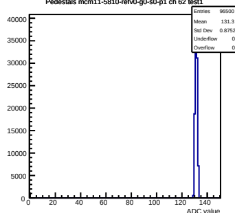
Pedestals mcm11-5810-refV0-g0-s0-p1 ch 62 test1
