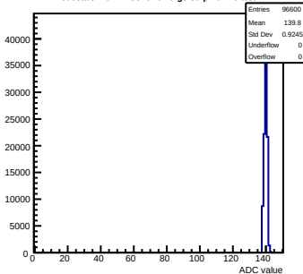
Pedestals mcm11-5810-refV0-g0-s0-p1 ch 46 test1
