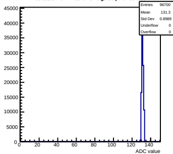
Pedestals mcm11-5810-refV0-g0-s0-p1 ch 85 test1
