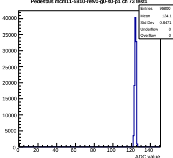
Pedestals mcm11-5810-refV0-g0-s0-p1 ch 73 test1
