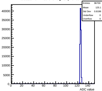
Pedestals mcm11-5810-refV0-g0-s0-p1 ch 90 test1
