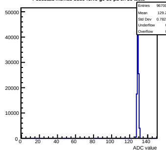
Pedestals mcm11-5810-refV0-g0-s0-p1 ch 30 test1
