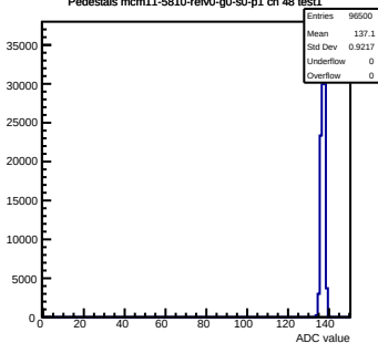
Pedestals mcm11-5810-refV0-g0-s0-p1 ch 48 test1
