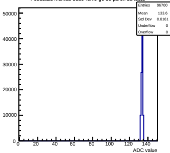
Pedestals mcm11-5810-refV0-g0-s0-p1 ch 82 test1
