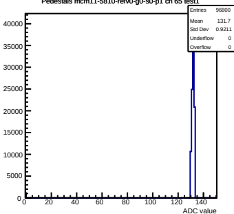
Pedestals mcm11-5810-refV0-g0-s0-p1 ch 65 test1
