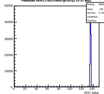
Pedestals mcm11-5810-refV0-g0-s0-p1 ch 51 test1
