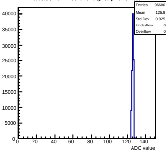
Pedestals mcm11-5810-refV0-g0-s0-p1 ch 37 test1
