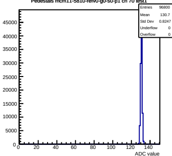
Pedestals mcm11-5810-refV0-g0-s0-p1 ch 70 test1
