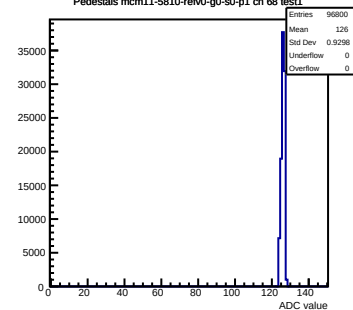
Pedestals mcm11-5810-refV0-g0-s0-p1 ch 68 test1
