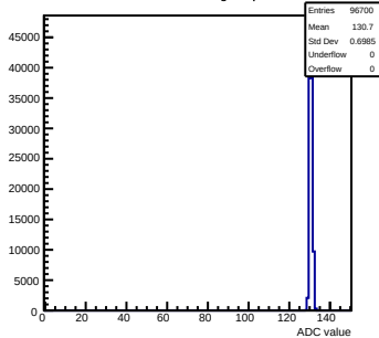
Pedestals mcm11-5810-refV0-g0-s0-p1 ch 93 test1
