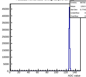
Pedestals mcm11-5810-refV0-g0-s0-p1 ch 21 test1
