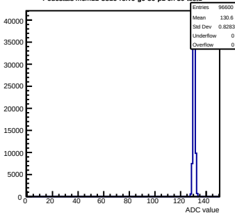
Pedestals mcm11-5810-refV0-g0-s0-p1 ch 39 test1
