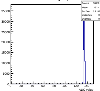
Pedestals mcm11-5810-refV0-g0-s0-p1 ch 45 test1
