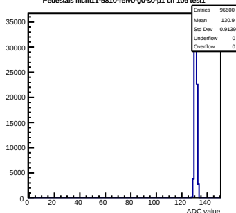
Pedestals mcm11-5810-refV0-g0-s0-p1 ch 106 test1
