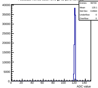
Pedestals mcm11-5810-refV0-g0-s0-p1 ch 81 test1
