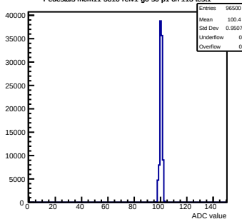
Pedestals mcm11-5810-refv1-g0-s0-p1 ch 115 test1
