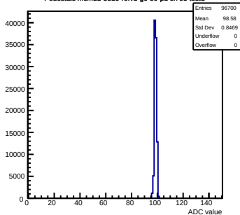
Pedestals mcm11-5810-refv1-g0-s0-p1 ch 95 test1
