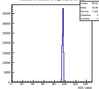
Pedestals mcm11-5810-refv1-g0-s0-p1 ch 90 test1
