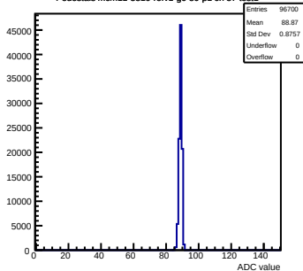
Pedestals mcm11-5810-refv1-g0-s0-p1 ch 87 test1
