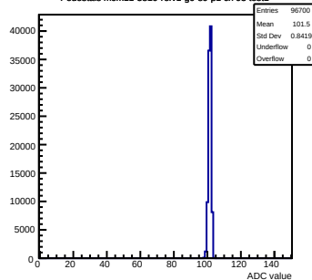
Pedestals mcm11-5810-refv1-g0-s0-p1 ch 93 test1
