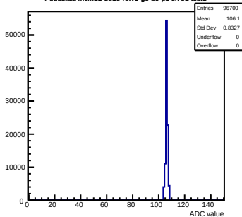
Pedestals mcm11-5810-refv1-g0-s0-p1 ch 91 test1
