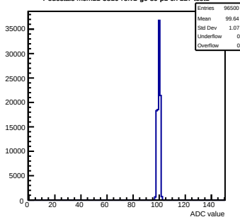
Pedestals mcm11-5810-refv1-g0-s0-p1 ch 127 test1
