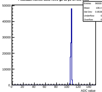
Pedestals mcm11-5810-refv1-g0-s0-p1 ch 119 test1
