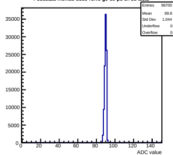
Pedestals mcm11-5810-refv1-g0-s0-p1 ch 81 test1
