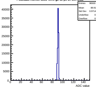
Pedestals mcm11-5810-refv1-g0-s0-p1 ch 114 test1
