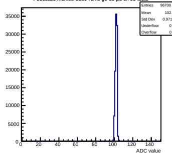
Pedestals mcm11-5810-refv1-g0-s0-p1 ch 85 test1
