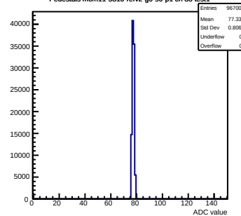
Pedestals mcm11-5810-refv2-g0-s0-p1 ch 83 test1
