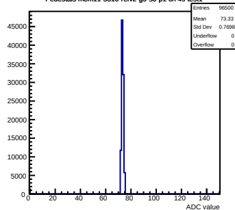
Pedestals mcm11-5810-refv2-g0-s0-p1 ch 49 test1
