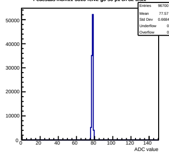
Pedestals mcm11-5810-refv2-g0-s0-p1 ch 82 test1
