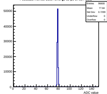
Pedestals mcm11-5810-refv2-g0-s0-p1 ch 107 test1
