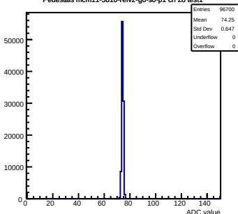
Pedestals mcm11-5810-ref2-g0-s0-p1 ch 28 test1
