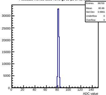
Pedestals mcm11-5810-ref2-g0-s0-p1 ch 16 test1
