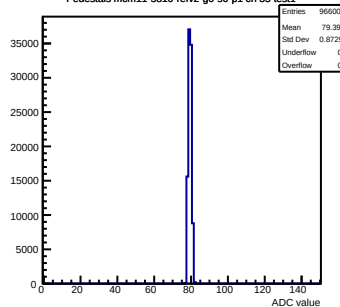
Pedestals mcm11-5810-refv2-g0-s0-p1 ch 35 test1
