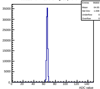
Pedestals mcm11-5810-refv4-g0-s0-p1 ch 67 test1
