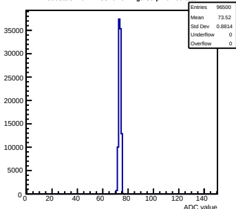
Pedestals mcm11-5810-refv4-g0-s0-p1 ch 60 test1
