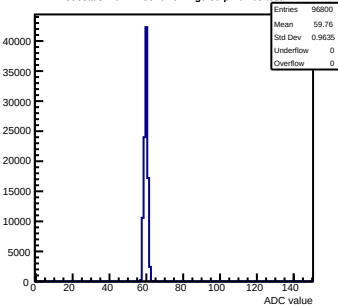
Pedestals mcm11-5810-refv4-g0-s0-p1 ch 68 test1
