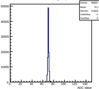
Pedestals mcm11-5810-refv4-g0-s0-p1 ch 76 test1
