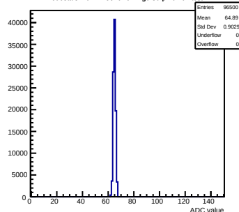
Pedestals mcm11-5810-refv4-g0-s0-p1 ch 62 test1
