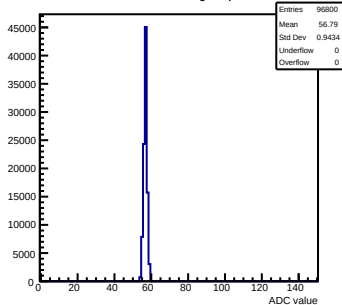
Pedestals mcm11-5810-refv4-g0-s0-p1 ch 73 test1
