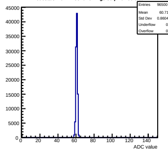
Pedestals mcm11-5810-refv4-g0-s0-p1 ch 50 test1
