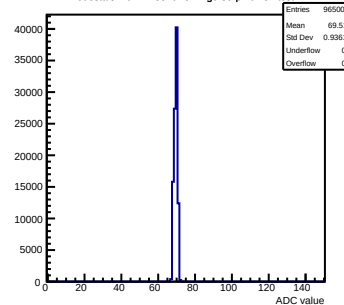
Pedestals mcm11-5810-refv4-g0-s0-p1 ch 51 test1
