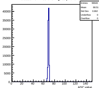
Pedestals mcm11-5810-refv4-g0-s0-p1 ch 57 test1
