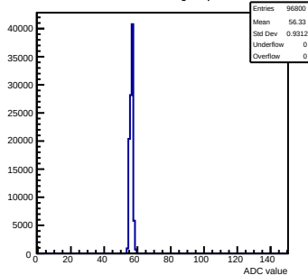
Pedestals mcm11-5810-refv4-g0-s0-p1 ch 79 test1
