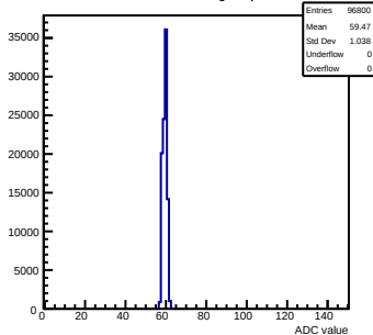
Pedestals mcm11-5810-refv4-g0-s0-p1 ch 78 test1
