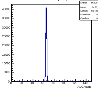
Pedestals mcm11-5810-refv4-g0-s0-p1 ch 66 test1
