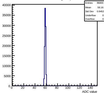
Pedestals mcm11-5810-refv4-g0-s0-p1 ch 74 test1
