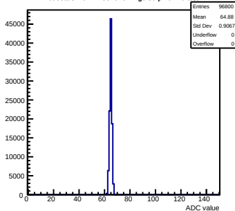
Pedestals mcm11-5810-refv4-g0-s0-p1 ch 70 test1
