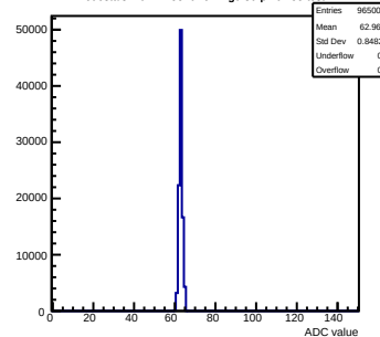
Pedestals mcm11-5810-refv4-g0-s0-p1 ch 55 test1
