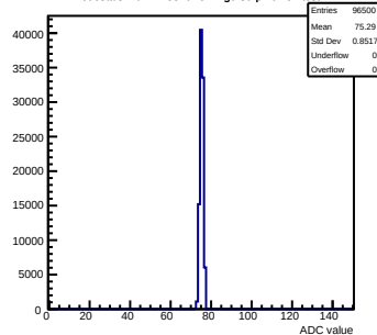
Pedestals mcm11-5810-refv4-g0-s0-p1 ch 54 test1
