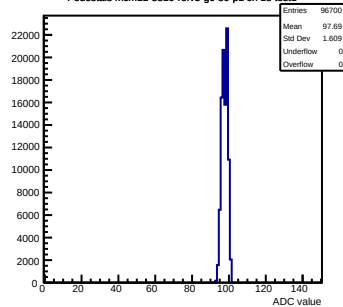
Pedestals mcm11-5810-refv5-g0-s0-p1 ch 18 test1
