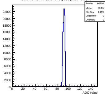
Pedestals mcm11-5810-refv5-g0-s0-p1 ch 29 test1
