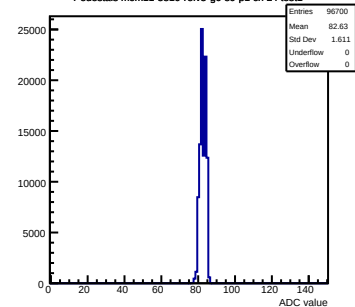
Pedestals mcm11-5810-refv5-g0-s0-p1 ch 24 test1
