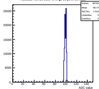
Pedestals mcm11-5810-refv5-g0-s0-p1 ch 26 test1
