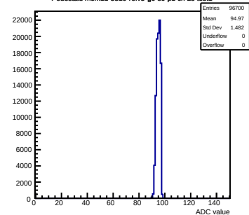
Pedestals mcm11-5810-refv5-g0-s0-p1 ch 28 test1
