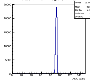
Pedestals mcm11-5810-refv5-g0-s0-p1 ch 19 test1
