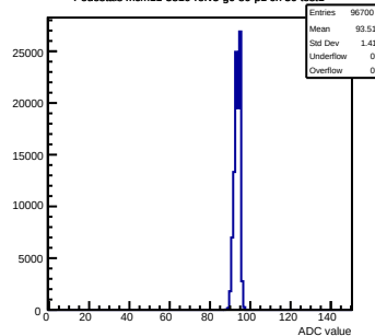
Pedestals mcm11-5810-refv5-g0-s0-p1 ch 30 test1
