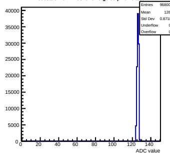
Pedestals mcm11-5810-rlv6-g0-s0-p1 ch 6 test1
