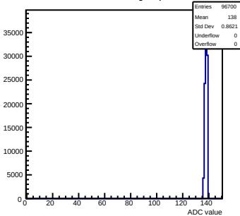
Pedestals mcm11-5810- rev6 -g0-s0-p1 ch 89 test1
