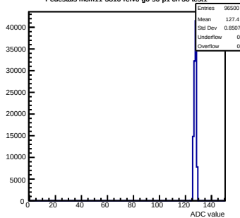
Pedestals mcm11-5810- rev6 -g0-s0-p1 ch 50 test1
