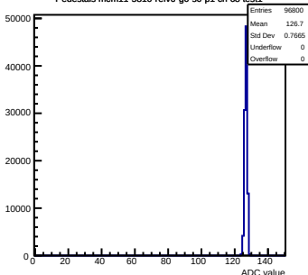
Pedestals mcm11-5810- rev6 -g0-s0-p1 ch 68 test1
