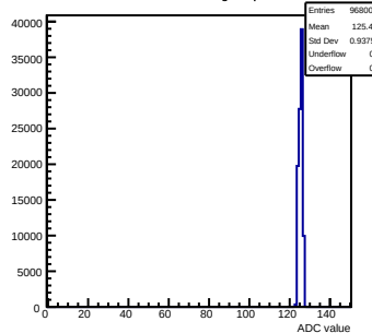
Pedestals mcm11-5810-rlv6-g0-s0-p1 ch 14 test1
