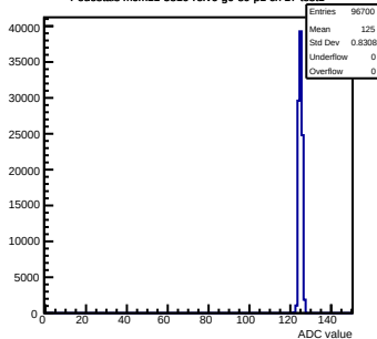
Pedestals mcm11-5810- rfv6-g0-s0-p1 ch 17 test1
