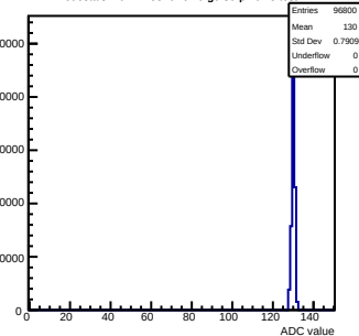
Pedestals mcm11-5810-rlv6-g0-s0-p1 ch 5 test1
