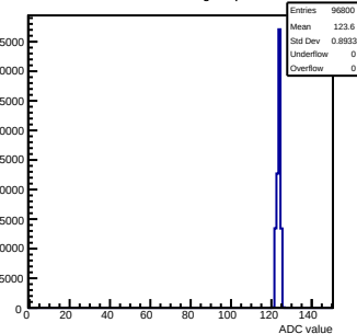
Pedestals mcm11-5810-rlv6-g0-s0-p1 ch 13 test1
