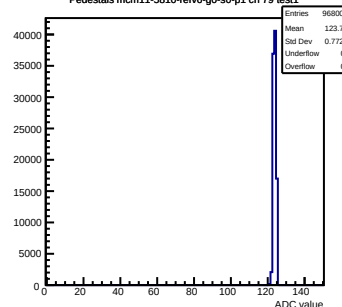
Pedestals mcm11-5810- rev6 -g0-s0-p1 ch 79 test1
