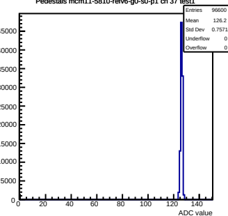
Pedestals mcm11-5810-refv6-g0-s0-p1 ch 37 test1
