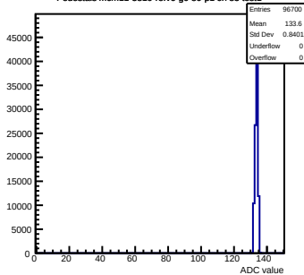
Pedestals mcm11-5810- rev6 -g0-s0-p1 ch 83 test1
