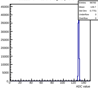
Pedestals mcm11-5810- rev6 -g0-s0-p1 ch 84 test1
