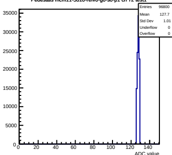
Pedestals mcm11-5810- rev6 -g0-s0-p1 ch 72 test1
