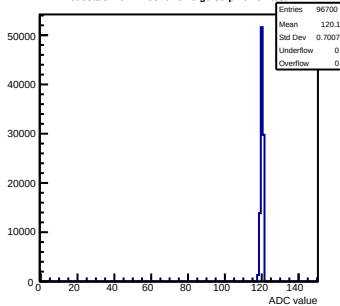
Pedestals mcm11-5810- rev6 -g0-s0-p1 ch 87 test1
