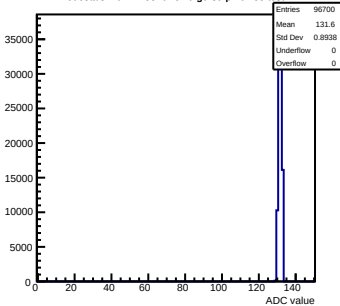
Pedestals mcm11-5810- rev6 -g0-s0-p1 ch 85 test1
