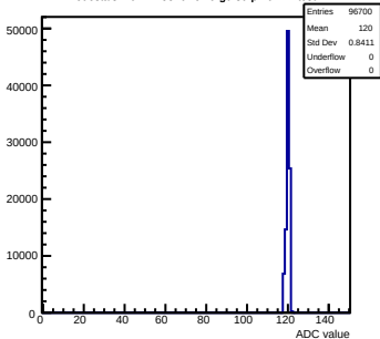
Pedestals mcm11-5810- rfv6-g0-s0-p1 ch 24 test1
