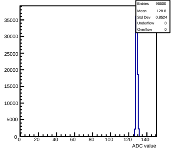
Pedestals mcm11-5810-rlv6-g0-s0-p1 ch 109 test1
