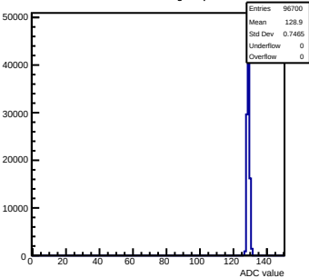
Pedestals mcm11-5810- rev6 -g0-s0-p1 ch 88 test1
