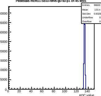
Pedestals mcm11-5810-refv6-g0-s0-p1 ch 45 test1
