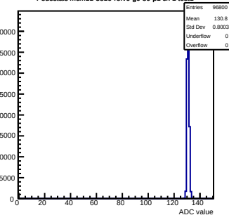
Pedestals mcm11-5810-rlv6-g0-s0-p1 ch 1 test1
