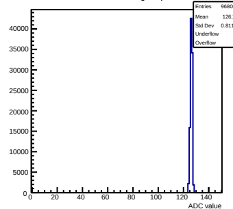
Pedestals mcm11-5810-rlv6-g0-s0-p1 ch 15 test1
