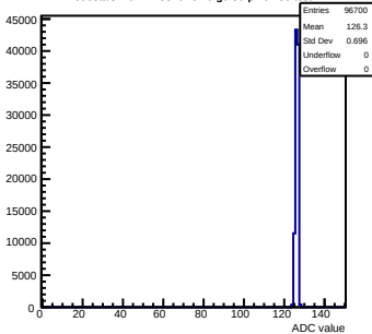
Pedestals mcm11-5810- rev6 -g0-s0-p1 ch 86 test1
