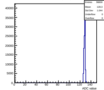
Pedestals mcm11-5810-rlv6-g0-s0-p1 ch 96 test1
