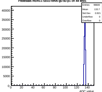
Pedestals mcm11-5810-refv6-g0-s0-p1 ch 44 test1
