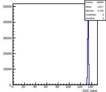
Pedestals mcm11-5810-rlv6-g0-s0-p1 ch 107 test1
