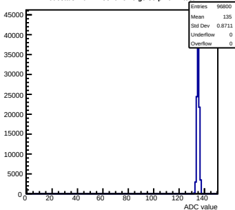
Pedestals mcm11-5810-rlv6-g0-s0-p1 ch 4 test1
