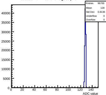
Pedestals mcm11-5810- rfv6-g0-s0-p1 ch 27 test1
