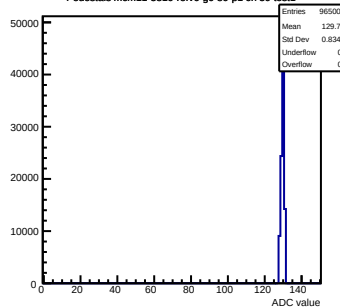
Pedestals mcm11-5810- rev6 -g0-s0-p1 ch 59 test1
