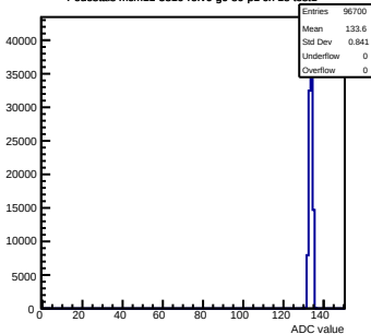
Pedestals mcm11-5810- rfv6-g0-s0-p1 ch 18 test1
