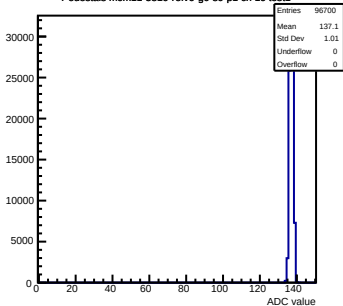
Pedestals mcm11-5810- rfv6-g0-s0-p1 ch 16 test1
