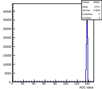
Pedestals mcm11-5810-rlv6-g0-s0-p1 ch 99 test1
