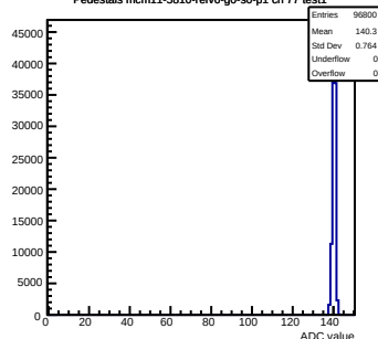
Pedestals mcm11-5810- rev6 -g0-s0-p1 ch 77 test1
