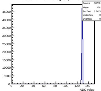
Pedestals mcm11-5810- rfv6-g0-s0-p1 ch 29 test1
