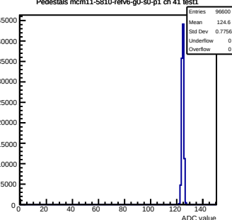
Pedestals mcm11-5810-refv6-g0-s0-p1 ch 41 test1
