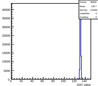
Pedestals mcm11-5810-rlv6-g0-s0-p1 ch 110 test1
