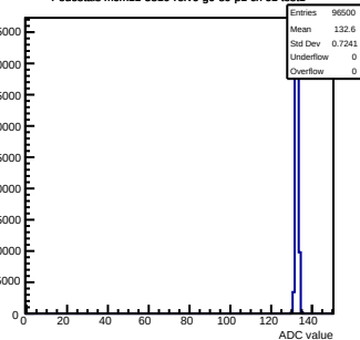
Pedestals mcm11-5810- rev6 -g0-s0-p1 ch 61 test1
