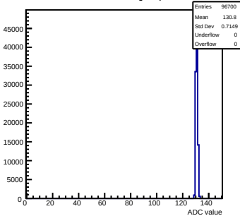
Pedestals mcm11-5810- rev6 -g0-s0-p1 ch 93 test1
