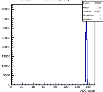
Pedestals mcm11-5810- rfv6-g0-s0-p1 ch 20 test1
