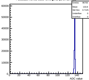
Pedestals mcm11-5810- rev6 -g0-s0-p1 ch 82 test1
