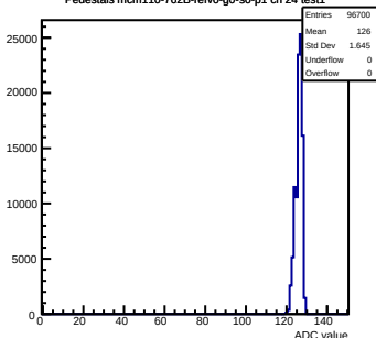
Pedestals mcm110-762B-refV0-g0-s0-p1 ch 24 test1
