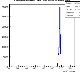
Pedestals mcm110-762B-refV0-g0-s0-p1 ch 26 test1
