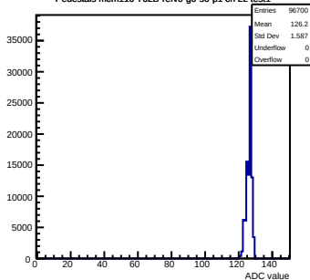
Pedestals mcm110-762B-refV0-g0-s0-p1 ch 22 test1
