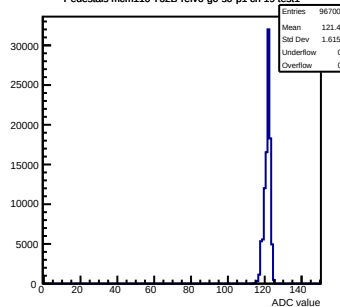
Pedestals mcm110-762B-refV0-g0-s0-p1 ch 19 test1
