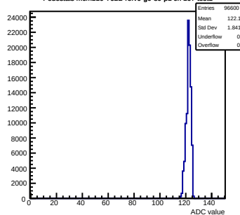
Pedestals mcm110-762B-refV0-g0-s0-p1 ch 107 test1
