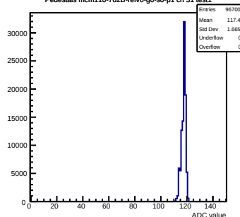
Pedestals mcm110-762B-refV0-g0-s0-p1 ch 31 test1
