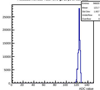
Pedestals mcm110-762B-refV0-g0-s0-p1 ch 109 test1
