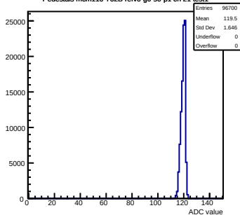
Pedestals mcm110-762B-refV0-g0-s0-p1 ch 21 test1
