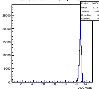
Pedestals mcm110-762B-refV0-g0-s0-p1 ch 106 test1
