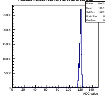
Pedestals mcm110-762B-refV0-g0-s0-p1 ch 102 test1
