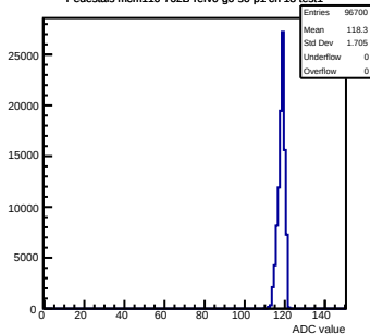
Pedestals mcm110-762B-refV0-g0-s0-p1 ch 18 test1
