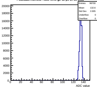
Pedestals mcm110-762B-refV0-g0-s0-p1 ch 16 test1
