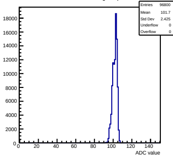
Pedestals mcm110-762B-refV1-g0-s0-p1 ch 12 test1
