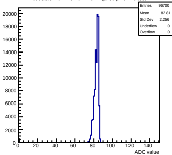
Pedestals mcm110-762B-refv1-g0-s0-p1 ch 25 test1
