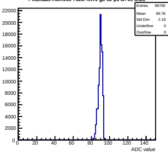
Pedestals mcm110-762B-refv1-g0-s0-p1 ch 19 test1
