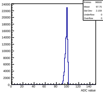
Pedestals mcm110-762B-refv1-g0-s0-p1 ch 56 test1
