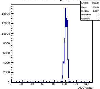
Pedestals mcm110-762B-refV1-g0-s0-p1 ch 0 test1
