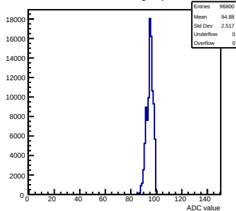
Pedestals mcm110-762B-refV1-g0-s0-p1 ch 15 test1
