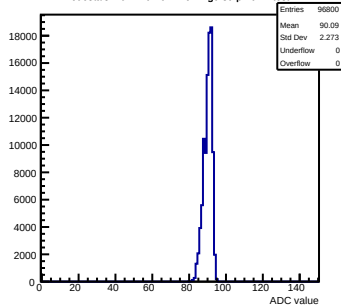
Pedestals mcm110-762B-refV1-g0-s0-p1 ch 1 test1
