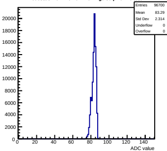
Pedestals mcm110-762B-refv1-g0-s0-p1 ch 26 test1
