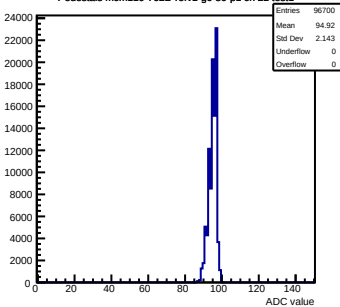
Pedestals mcm110-762B-refv1-g0-s0-p1 ch 22 test1
