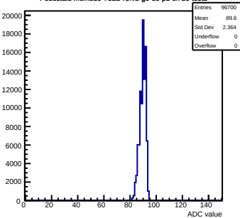
Pedestals mcm110-762B-refv1-g0-s0-p1 ch 20 test1
