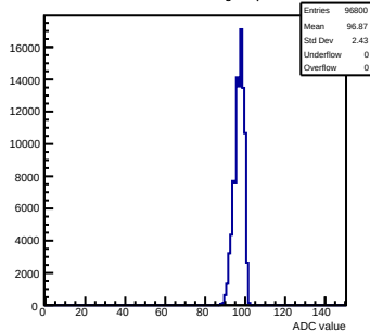
Pedestals mcm110-762B-refV1-g0-s0-p1 ch 9 test1
