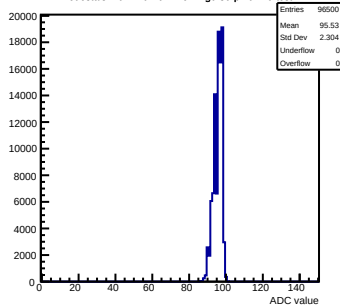
Pedestals mcm110-762B-refv1-g0-s0-p1 ch 49 test1
