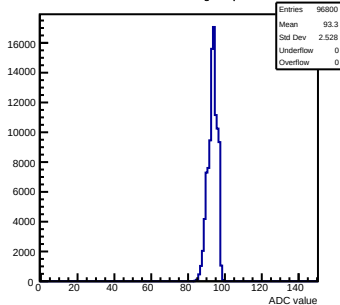
Pedestals mcm110-762B-refV1-g0-s0-p1 ch 10 test1
