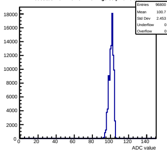
Pedestals mcm110-762B-refV1-g0-s0-p1 ch 6 test1
