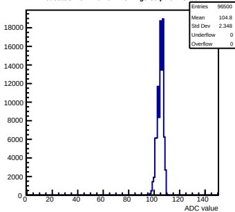
Pedestals mcm110-762B-refv1-g0-s0-p1 ch 48 test1
