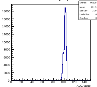
Pedestals mcm110-762B-refV1-g0-s0-p1 ch 2 test1
