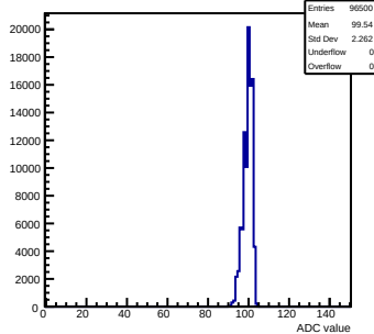
Pedestals mcm110-762B-refv1-g0-s0-p1 ch 61 test1
