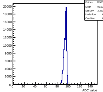
Pedestals mcm110-762B-refv1-g0-s0-p1 ch 63 test1
