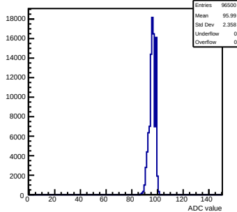
Pedestals mcm110-762B-refv1-g0-s0-p1 ch 58 test1
