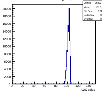
Pedestals mcm110-762B-refV1-g0-s0-p1 ch 7 test1
