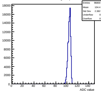
Pedestals mcm110-762B-refV1-g0-s0-p1 ch 14 test1
