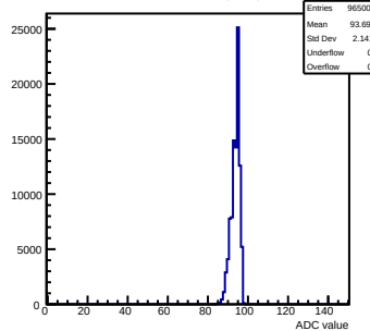
Pedestals mcm110-762B-refv1-g0-s0-p1 ch 55 test1
