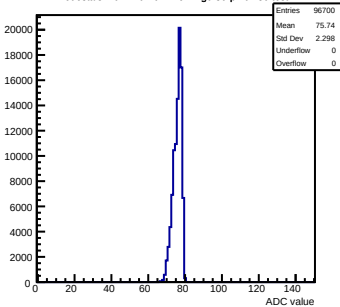
Pedestals mcm110-762B-refv1-g0-s0-p1 ch 30 test1
