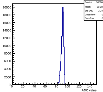
Pedestals mcm110-762B-refv1-g0-s0-p1 ch 57 test1
