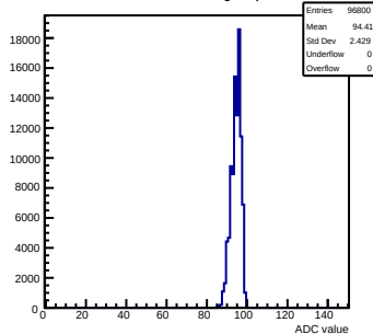
Pedestals mcm110-762B-refV1-g0-s0-p1 ch 13 test1
