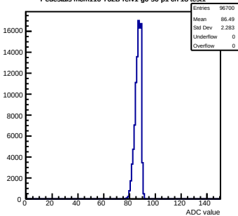
Pedestals mcm110-762B-refv1-g0-s0-p1 ch 18 test1
