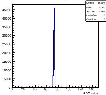
Pedestals mcm110-762B-refV2-g0-s0-p1 ch 62 test1
