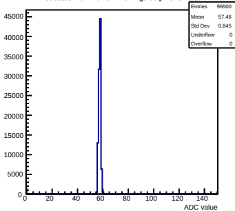
Pedestals mcm110-762B-refV2-g0-s0-p1 ch 52 test1
