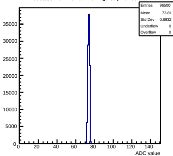
Pedestals mcm110-762B-refV2-g0-s0-p1 ch 56 test1
