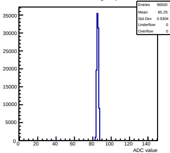
Pedestals mcm110-762B-refV2-g0-s0-p1 ch 60 test1
