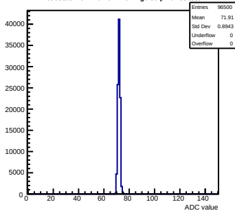
Pedestals mcm110-762B-refV2-g0-s0-p1 ch 58 test1
