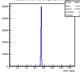
Pedestals mcm110-762B-refV2-g0-s0-p1 ch 51 test1
