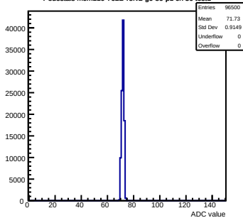
Pedestals mcm110-762B-g0-s0-p1 ch 50 test1
