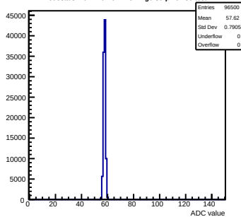
Pedestals mcm110-762B-refV2-g0-s0-p1 ch 59 test1
