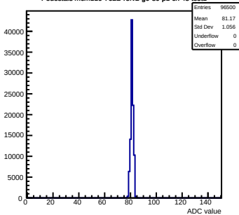
Pedestals mcm110-762B-g0-s0-p1 ch 48 test1
