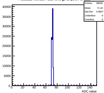
Pedestals mcm110-762B-g0-s0-p1 ch 49 test1
