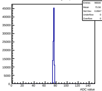
Pedestals mcm110-762B-refV2-g0-s0-p1 ch 61 test1
