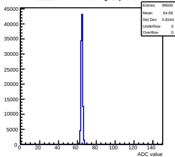
Pedestals mcm110-762B-refV2-g0-s0-p1 ch 57 test1
