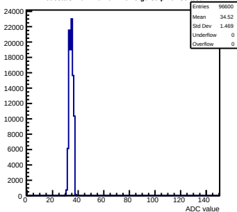
Pedestals mcm110-762B-refV3-g0-s0-p1 ch 36 test1
