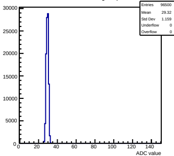
Pedestals mcm110-7628-refv3-g0-s0-p1 ch 125 test1
