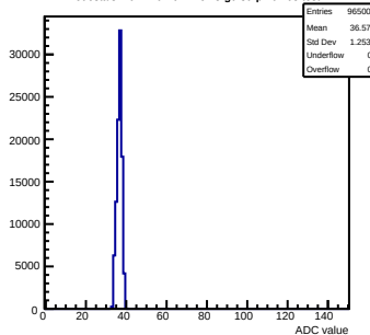
Pedestals mcm110-762B-refV3-g0-s0-p1 ch 63 test1
