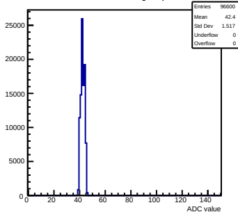
Pedestals mcm110-762B-refV3-g0-s0-p1 ch 42 test1
