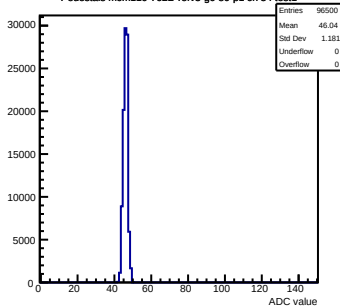
Pedestals mcm110-762B-refV3-g0-s0-p1 ch 54 test1
