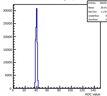
Pedestals mcm110-7628-refv3-g0-s0-p1 ch 123 test1
