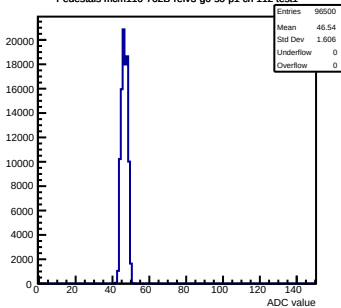
Pedestals mcm110-7628-refv3-g0-s0-p1 ch 112 test1
