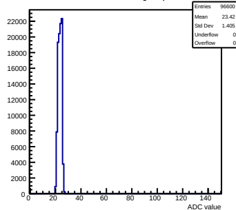
Pedestals mcm110-762B-refV3-g0-s0-p1 ch 43 test1
