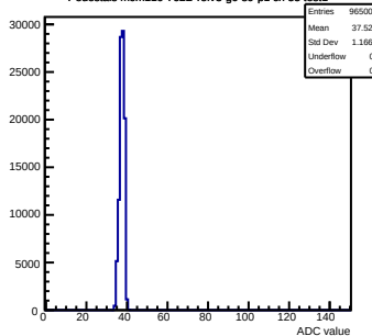
Pedestals mcm110-762B-refV3-g0-s0-p1 ch 55 test1
