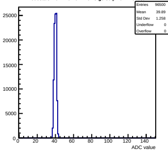
Pedestals mcm110-7628-refv3-g0-s0-p1 ch 116 test1
