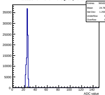
Pedestals mcm110-762B-refV3-g0-s0-p1 ch 59 test1
