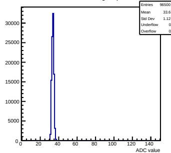
Pedestals mcm110-7628-refv3-g0-s0-p1 ch 126 test1
