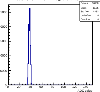
Pedestals mcm110-762B-refV3-g0-s0-p1 ch 33 test1
