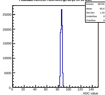
Pedestals mcm110-762B-refV5-g0-s0-p1 ch 93 test1
