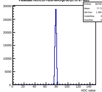
Pedestals mcm110-762B-refV5-g0-s0-p1 ch 87 test1
