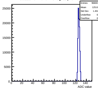
Pedestals mcm110-762B-relv6-g0-s0-p1 ch 10 test1
