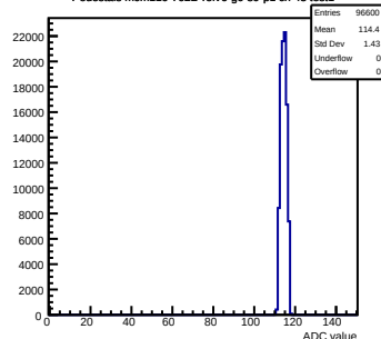
Pedestals mcm110-762B-refv6-g0-s0-p1 ch 43 test1
