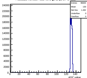
Pedestals mcm110-762B-refv6-g0-s0-p1 ch 42 test1
