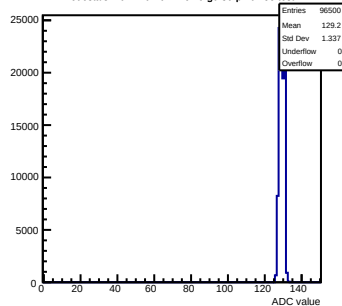
Pedestals mcm110-762B-refv6-g0-s0-p1 ch 58 test1
