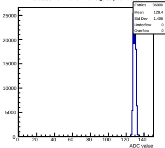
Pedestals mcm110-762B-relv6-g0-s0-p1 ch 9 test1
