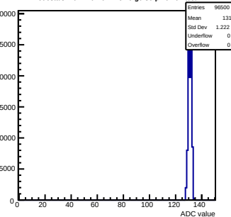
Pedestals mcm110-762B-refv6-g0-s0-p1 ch 61 test1
