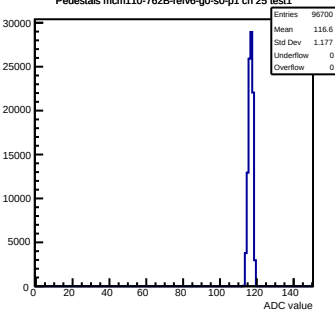
Pedestals mcm110-762B-refv6-g0-s0-p1 ch 25 test1
