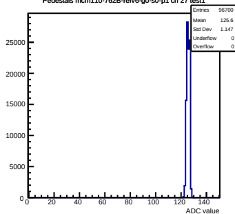
Pedestals mcm110-762B-refv6-g0-s0-p1 ch 27 test1
