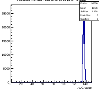
Pedestals mcm110-762B-refv6-g0-s0-p1 ch 48 test1
