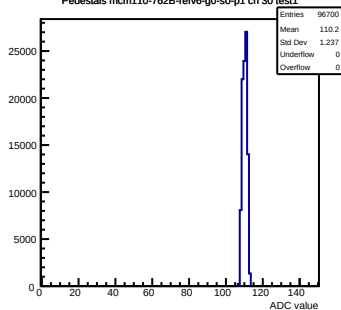
Pedestals mcm110-762B-refv6-g0-s0-p1 ch 30 test1
