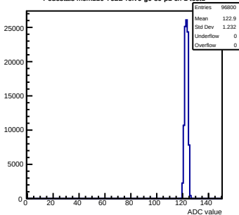
Pedestals mcm110-762B-relv6-g0-s0-p1 ch 1 test1
