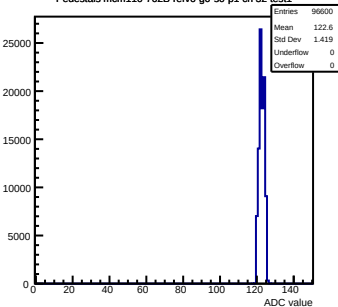
Pedestals mcm110-762B-refv6-g0-s0-p1 ch 32 test1
