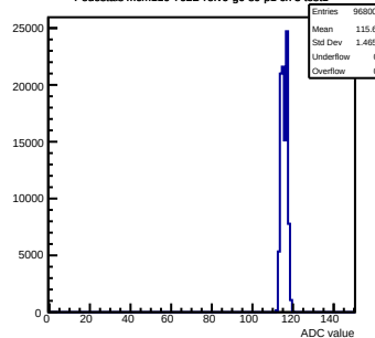
Pedestals mcm110-762B-relv6-g0-s0-p1 ch 3 test1
