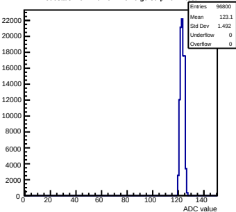
Pedestals mcm110-762B-relv6-g0-s0-p1 ch 4 test1
