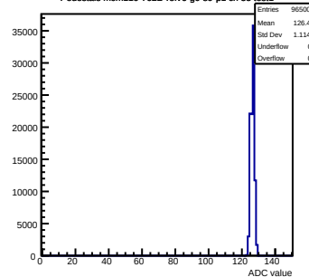
Pedestals mcm110-762B-refv6-g0-s0-p1 ch 55 test1
