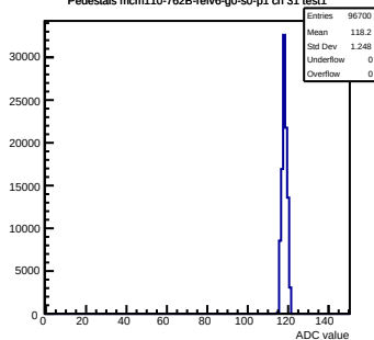
Pedestals mcm110-762B-refv6-g0-s0-p1 ch 31 test1
