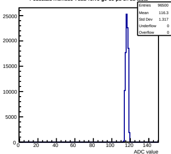
Pedestals mcm110-762B-refv6-g0-s0-p1 ch 52 test1
