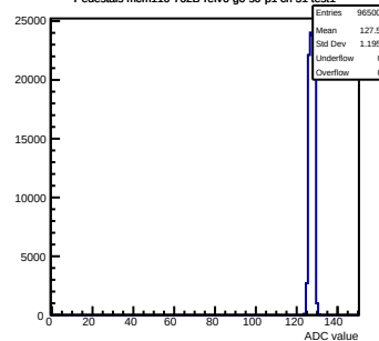
Pedestals mcm110-762B-refv6-g0-s0-p1 ch 51 test1
