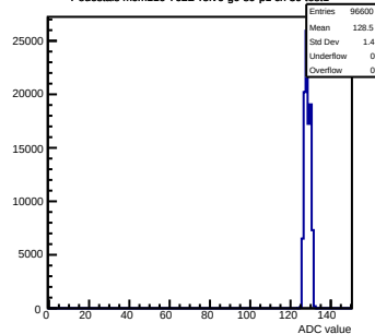
Pedestals mcm110-762B-refv6-g0-s0-p1 ch 39 test1
