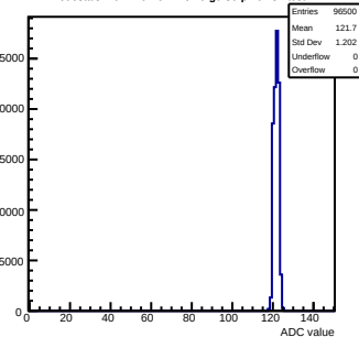
Pedestals mcm110-762B-refv6-g0-s0-p1 ch 57 test1
