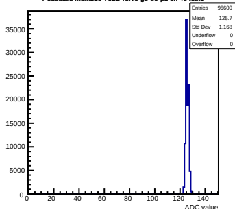
Pedestals mcm110-762B-refv6-g0-s0-p1 ch 46 test1
