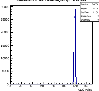
Pedestals mcm110-762B-refv6-g0-s0-p1 ch 29 test1
