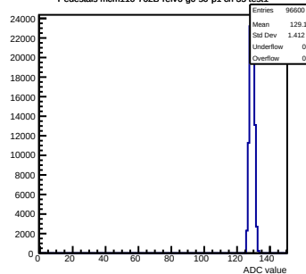
Pedestals mcm110-762B-refv6-g0-s0-p1 ch 35 test1
