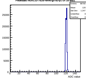
Pedestals mcm110-762B-refv6-g0-s0-p1 ch 18 test1
