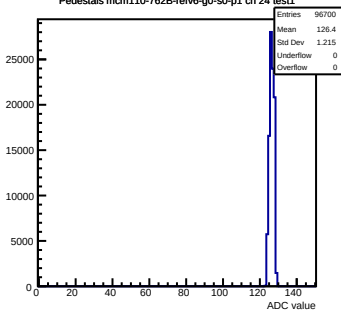
Pedestals mcm110-762B-refv6-g0-s0-p1 ch 24 test1
