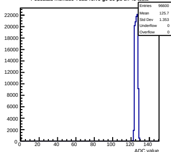
Pedestals mcm110-762B-refv6-g0-s0-p1 ch 45 test1
