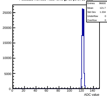
Pedestals mcm110-762B-refv6-g0-s0-p1 ch 38 test1
