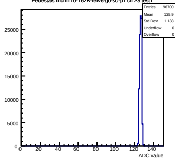
Pedestals mcm110-762B-refv6-g0-s0-p1 ch 23 test1
