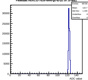
Pedestals mcm110-762B-refv6-g0-s0-p1 ch 19 test1
