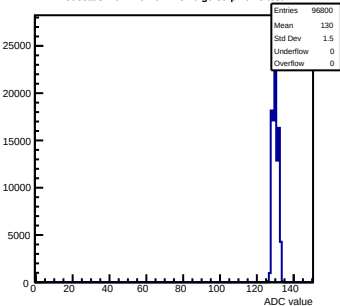
Pedestals mcm110-762B-relv6-g0-s0-p1 ch 8 test1
