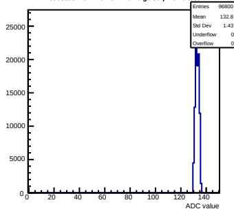
Pedestals mcm110-762B-relv6-g0-s0-p1 ch 6 test1
