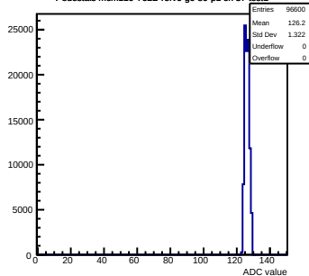
Pedestals mcm110-762B-refv6-g0-s0-p1 ch 37 test1
