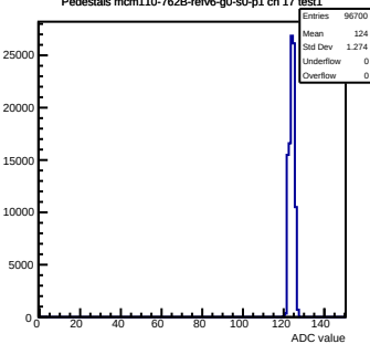
Pedestals mcm110-762B-refv6-g0-s0-p1 ch 17 test1
