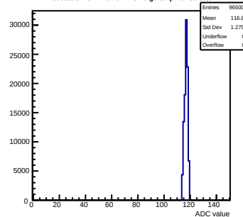
Pedestals mcm110-762B-refv6-g0-s0-p1 ch 59 test1
