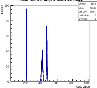
Pulse mcm 0 chip 1 chan 12 test1
