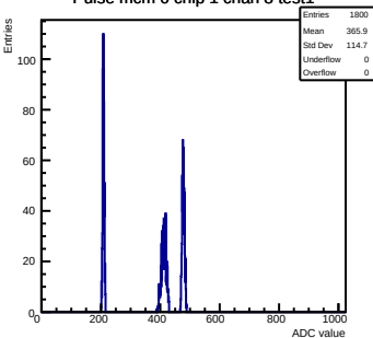
Pulse mcm 0 chip 1 chan 8 test1
