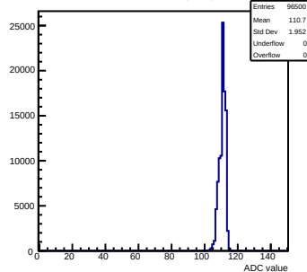
Pedestals mcm111-5610-rfv0-g0-s0-p1 ch 53 test1
