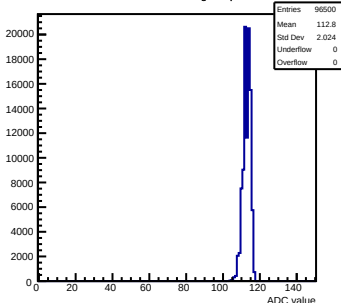
Pedestals mcm111-5610-rfv0-g0-s0-p1 ch 60 test1
