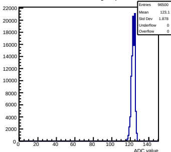
Pedestals mcm111-5610-rfv0-g0-s0-p1 ch 56 test1
