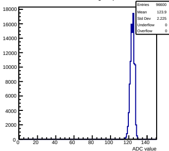
Pedestals mcm111-5610-refV0-g0-s0-p1 ch 104 test1
