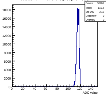
Pedestals mcm111-5610-rfv0-g0-s0-p1 ch 20 test1
