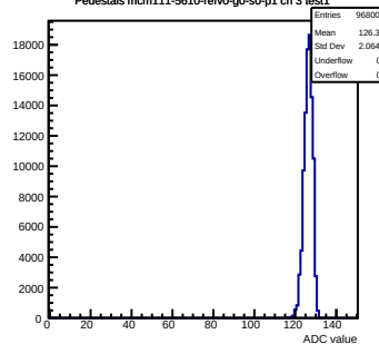
Pedestals mcm111-5610-refV0-g0-s0-p1 ch 3 test1
