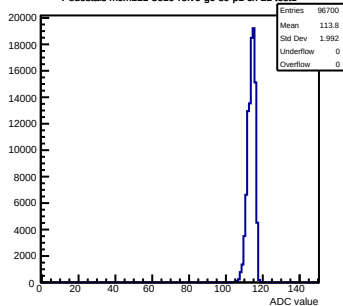
Pedestals mcm111-5610-rfv0-g0-s0-p1 ch 22 test1
