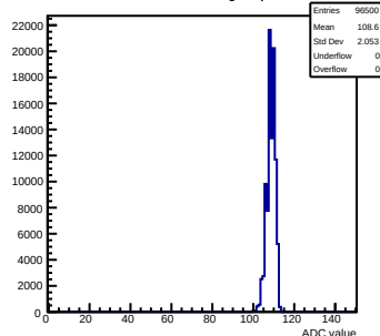
Pedestals mcm111-5610-rfv0-g0-s0-p1 ch 57 test1
