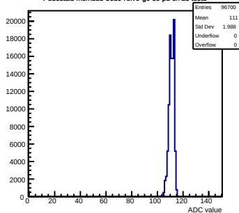
Pedestals mcm111-5610-rfv0-g0-s0-p1 ch 23 test1
