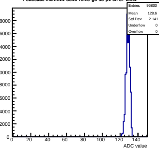
Pedestals mcm111-5610-rev0-g0-s0-p1 ch 67 test1
