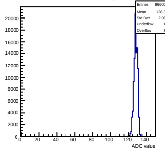
Pedestals mcm111-5610-refV0-g0-s0-p1 ch 111 test1
