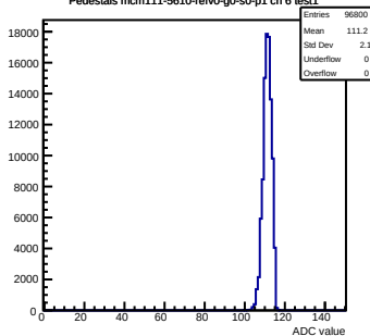
Pedestals mcm111-5610-refV0-g0-s0-p1 ch 6 test1
