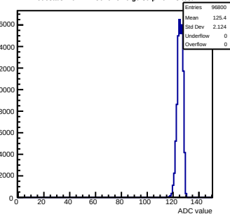
Pedestals mcm111-5610-rev0-g0-s0-p1 ch 73 test1
