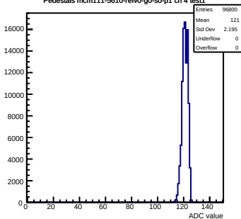
Pedestals mcm111-5610-refV0-g0-s0-p1 ch 4 test1
