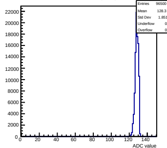
Pedestals mcm111-5610-rfv0-g0-s0-p1 ch 55 test1
