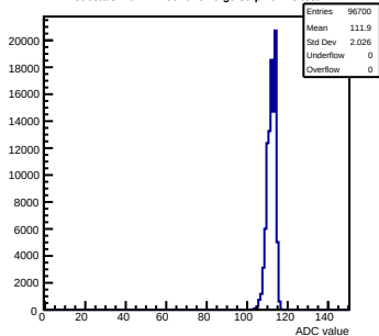
Pedestals mcm111-5610-rfv0-g0-s0-p1 ch 28 test1
