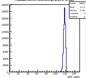
Pedestals mcm111-5610-refV0-g0-s0-p1 ch 12 test1
