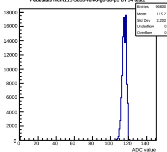
Pedestals mcm111-5610-refV0-g0-s0-p1 ch 14 test1
