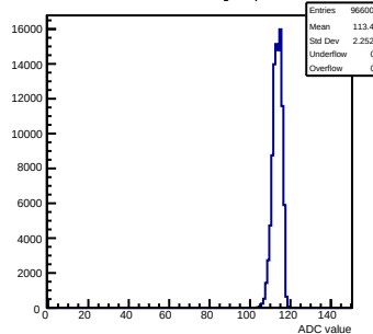
Pedestals mcm111-5610-refV0-g0-s0-p1 ch 110 test1
