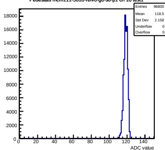
Pedestals mcm111-5610-refV0-g0-s0-p1 ch 10 test1
