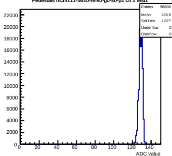
Pedestals mcm111-5610-refV0-g0-s0-p1 ch 2 test1
