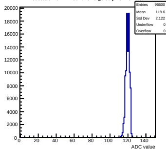
Pedestals mcm111-5610-refV0-g0-s0-p1 ch 101 test1
