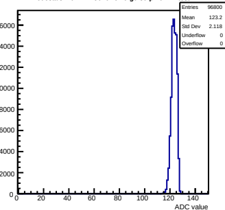
Pedestals mcm111-5610-rev0-g0-s0-p1 ch 74 test1
