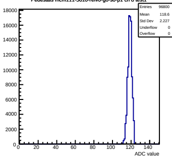
Pedestals mcm111-5610-refV0-g0-s0-p1 ch 8 test1
