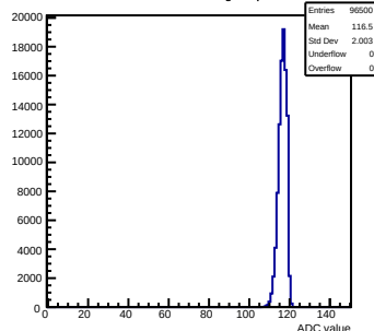
Pedestals mcm111-5610-rfv0-g0-s0-p1 ch 61 test1
