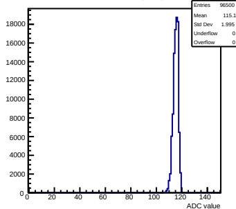
Pedestals mcm111-5610-rfv0-g0-s0-p1 ch 54 test1
