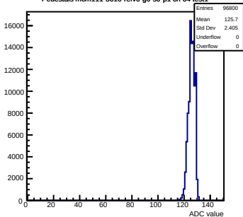
Pedestals mcm111-5610-rev0-g0-s0-p1 ch 64 test1
