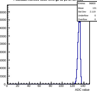
Pedestals mcm111-5610-rev0-g0-s0-p1 ch 65 test1
