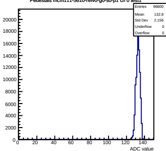
Pedestals mcm111-5610-refV0-g0-s0-p1 ch 0 test1
