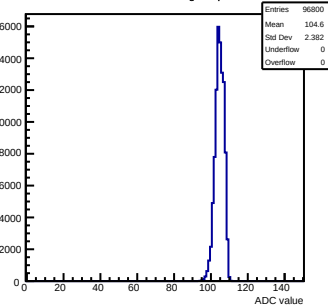
Pedestals mcm111-5610-rev0-g0-s0-p1 ch 78 test1
