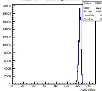
Pedestals mcm111-5610-refV0-g0-s0-p1 ch 97 test1
