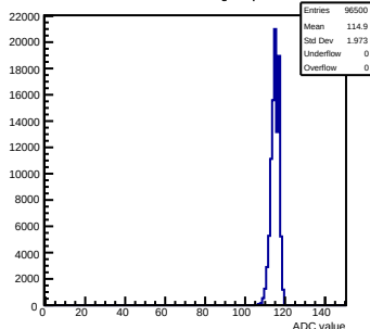
Pedestals mcm111-5610-rfv0-g0-s0-p1 ch 62 test1
