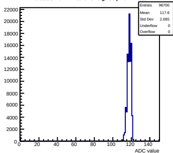
Pedestals mcm111-5610-rfv0-g0-s0-p1 ch 24 test1
