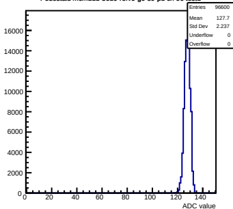
Pedestals mcm111-5610-refV0-g0-s0-p1 ch 96 test1
