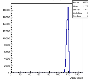
Pedestals mcm111-5610-refV0-g0-s0-p1 ch 106 test1
