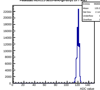
Pedestals mcm111-5610-refV0-g0-s0-p1 ch 7 test1
