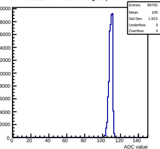
Pedestals mcm111-5610-rfv0-g0-s0-p1 ch 25 test1
