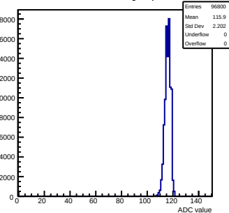
Pedestals mcm111-5610-rev0-g0-s0-p1 ch 79 test1
