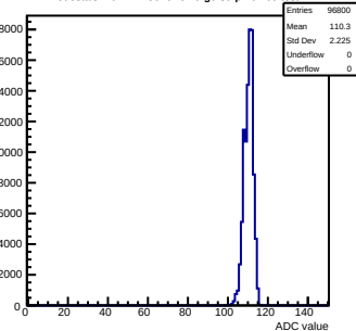
Pedestals mcm111-5610-rev0-g0-s0-p1 ch 69 test1
