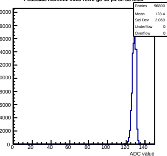
Pedestals mcm111-5610-rev0-g0-s0-p1 ch 66 test1
