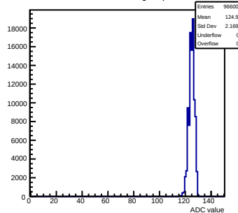
Pedestals mcm111-5610-refV0-g0-s0-p1 ch 107 test1
