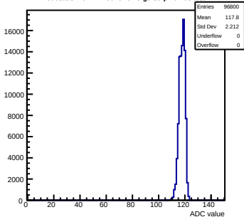
Pedestals mcm111-5610-rev0-g0-s0-p1 ch 68 test1
