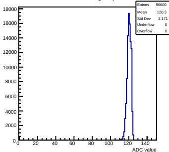
Pedestals mcm111-5610-refV0-g0-s0-p1 ch 108 test1
