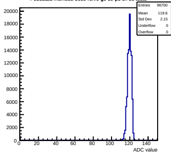
Pedestals mcm111-5610-rfv0-g0-s0-p1 ch 16 test1
