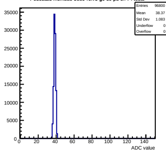
Pedestals mcm111-5610-refv3-g0-s0-p1 ch 74 test1
