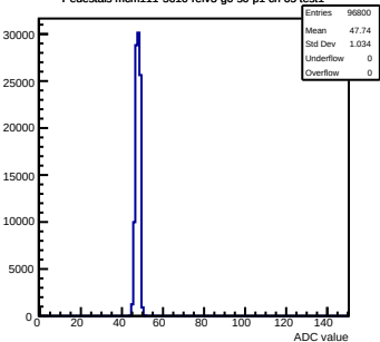
Pedestals mcm111-5610-refv3-g0-s0-p1 ch 65 test1
