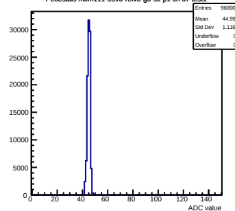
Pedestals mcm111-5610-refv3-g0-s0-p1 ch 67 test1
