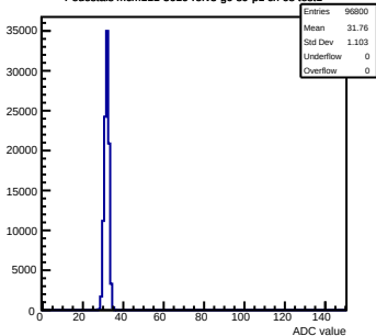
Pedestals mcm111-5610-refv3-g0-s0-p1 ch 68 test1
