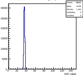
Pedestals mcm111-5610-refv3-g0-s0-p1 ch 77 test1
