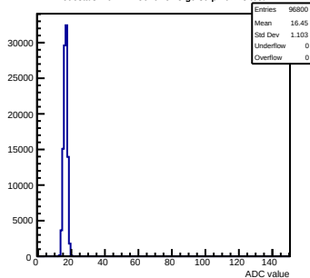
Pedestals mcm111-5610-refv3-g0-s0-p1 ch 78 test1
