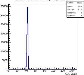
Pedestals mcm111-5610-refv3-g0-s0-p1 ch 73 test1
