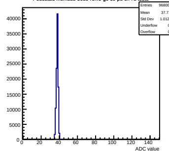
Pedestals mcm111-5610-refv3-g0-s0-p1 ch 71 test1
