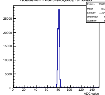
Pedestals mcm111-5610-refv5-g0-s0-p1 ch 38 test1
