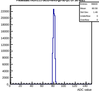
Pedestals mcm111-5610-refv5-g0-s0-p1 ch 36 test1
