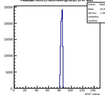
Pedestals mcm111-5610-refv5-g0-s0-p1 ch 47 test1
