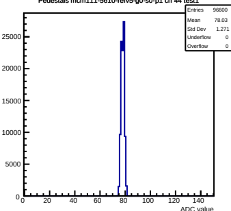
Pedestals mcm111-5610-refv5-g0-s0-p1 ch 44 test1
