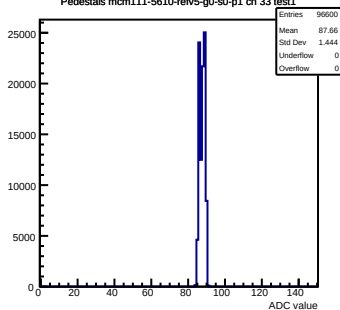
Pedestals mcm111-5610-refv5-g0-s0-p1 ch 33 test1
