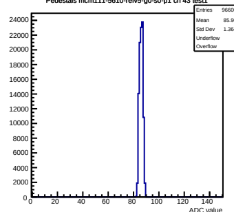
Pedestals mcm111-5610-refv5-g0-s0-p1 ch 43 test1
