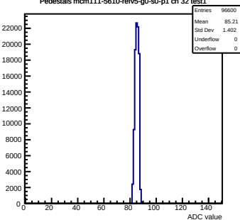
Pedestals mcm111-5610-refv5-g0-s0-p1 ch 32 test1
