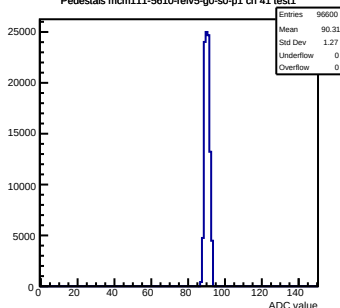
Pedestals mcm111-5610-refv5-g0-s0-p1 ch 41 test1
