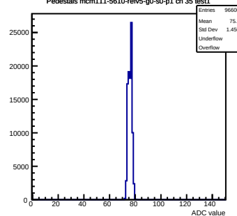
Pedestals mcm111-5610-refv5-g0-s0-p1 ch 35 test1
