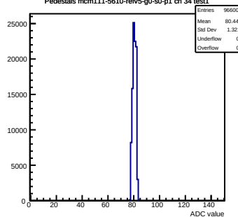
Pedestals mcm111-5610-refv5-g0-s0-p1 ch 34 test1
