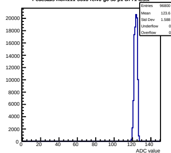
Pedestals mcm111-5610-relv6-g0-s0-p1 ch 71 test1
