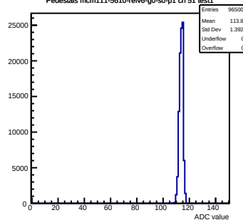
Pedestals mcm111-5610-rlv6-g0-s0-p1 ch 51 test1
