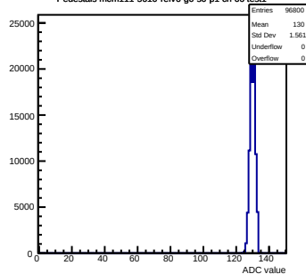
Pedestals mcm111-5610-relv6-g0-s0-p1 ch 66 test1
