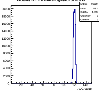
Pedestals mcm111-5610-rlv6-g0-s0-p1 ch 48 test1
