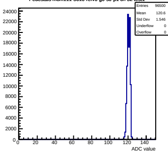
Pedestals mcm111-5610-rlv6-g0-s0-p1 ch 52 test1
