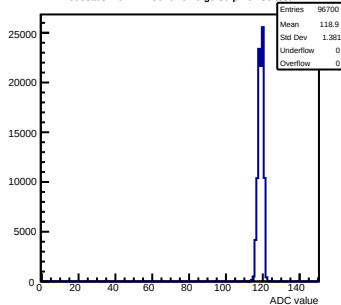
Pedestals mcm111-5610-refv6-g0-s0-p1 ch 86 test1
