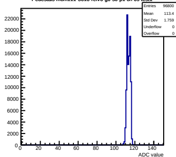
Pedestals mcm111-5610-relv6-g0-s0-p1 ch 69 test1
