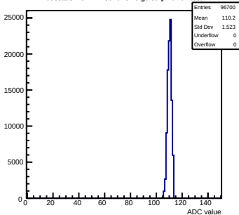
Pedestals mcm111-5610-refv6-g0-s0-p1 ch 92 test1
