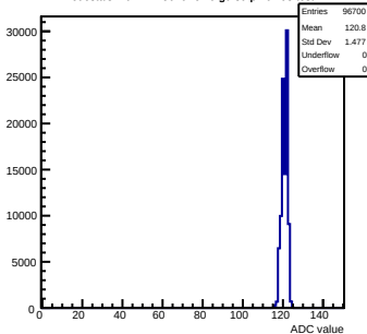
Pedestals mcm111-5610-refv6-g0-s0-p1 ch 93 test1
