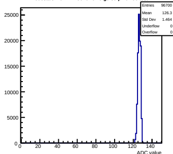
Pedestals mcm111-5610-refv6-g0-s0-p1 ch 90 test1
