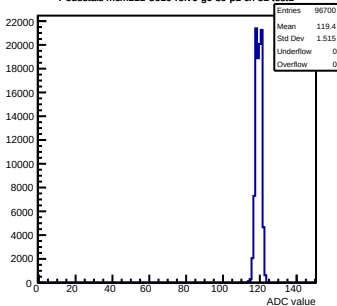
Pedestals mcm111-5610-refv6-g0-s0-p1 ch 81 test1
