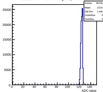
Pedestals mcm111-5610-refv6-g0-s0-p1 ch 95 test1
