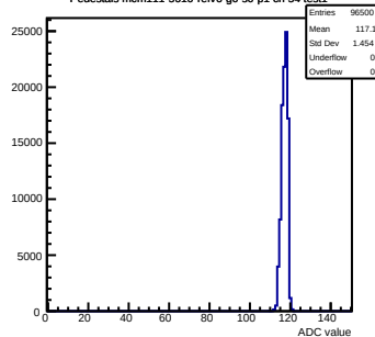
Pedestals mcm111-5610-rlv6-g0-s0-p1 ch 54 test1
