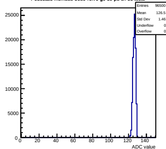
Pedestals mcm111-5610-rlv6-g0-s0-p1 ch 58 test1
