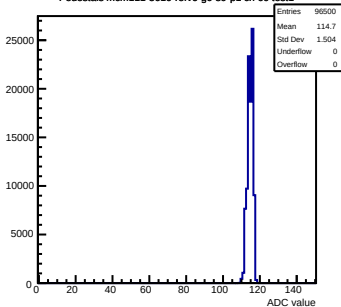
Pedestals mcm111-5610-rlv6-g0-s0-p1 ch 60 test1
