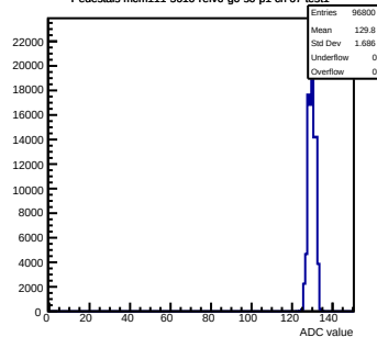
Pedestals mcm111-5610-relv6-g0-s0-p1 ch 67 test1
