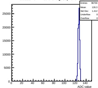
Pedestals mcm111-5610-refv6-g0-s0-p1 ch 94 test1
