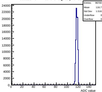
Pedestals mcm111-5610-refv6-g0-s0-p1 ch 85 test1
