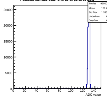
Pedestals mcm111-5610-rlv6-g0-s0-p1 ch 55 test1
