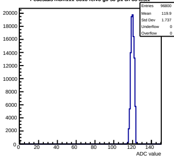
Pedestals mcm111-5610-relv6-g0-s0-p1 ch 68 test1
