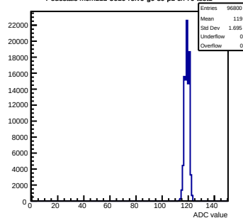
Pedestals mcm111-5610-relv6-g0-s0-p1 ch 79 test1
