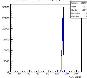
Pedestals mcm111-5610-rlv6-g0-s0-p1 ch 57 test1
