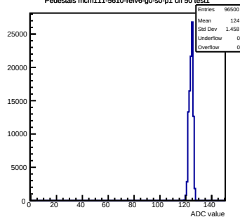
Pedestals mcm111-5610-rlv6-g0-s0-p1 ch 50 test1
