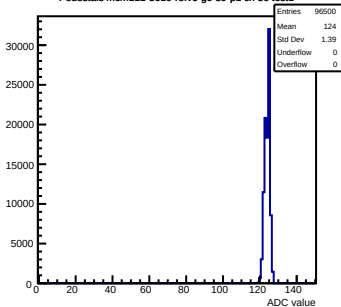
Pedestals mcm111-5610-rlv6-g0-s0-p1 ch 56 test1
