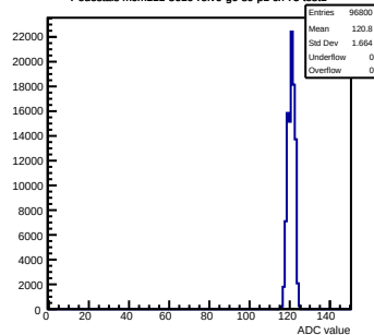
Pedestals mcm111-5610-relv6-g0-s0-p1 ch 75 test1
