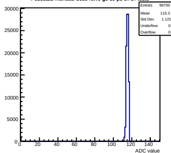
Pedestals mcm111-5610-refV0-g0-s0-p1 ch 17 test1
